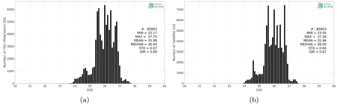
Figure 2: Histograms of SSS from TSG (Polarstern) (a) and SMAP SSS L4 OI v2 - Monthly (IPRC) (b) considering all match-up pairs per bins of 0.1 over the Mid-Low Latitudes 45N-45S Pi-MEP region and for the full satellite product period.
