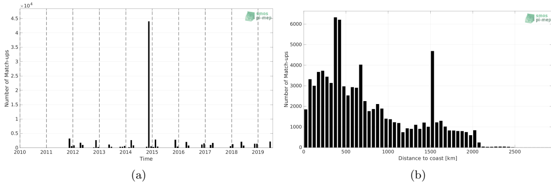
Figure 1: Number of match-ups between TSG (Polarstern) and SMAP SSS L4 OI v2 - Monthly (IPRC) SSS as a function of time (a) and as function of the distance to coast (b) over the Mid-Low Latitudes 45N-45S Pi-MEP region and for the full satellite product period.
