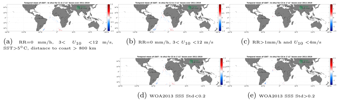
Figure 12: Temporal mean gridded over spatial boxes of size 1^\circ \times 1^\circ of \Delta SSS (SMAP SSS L4 OI v2 - Monthly (IPRC) - TSG (Polarstern)) for 5 different subdatasets corresponding to:RR=0 mm/h, 3 < U_{10} < 12 m/s, SST >5^\circ\text{C} , distance to coast > 800 km (a), RR=0 mm/h, 3 < U_{10} < 12 m/s (b), RR >1 mm/h and U_{10} < 4 m/s (c), WOA2013 SSS Std <0.2 (d), WOA2013 SSS Std >0.2 (e).
