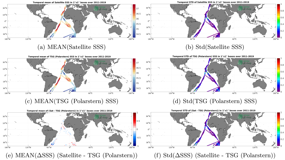
Figure 6: Temporal mean (left) and Std (right) of SSS from SMAP SSS L4 OI v2 - Monthly (IPRC) (top), TSG (Polarstern) (middle), and of \Delta SSS (Satellite - TSG (Polarstern)). Only match-up pairs are used to generate these maps.
