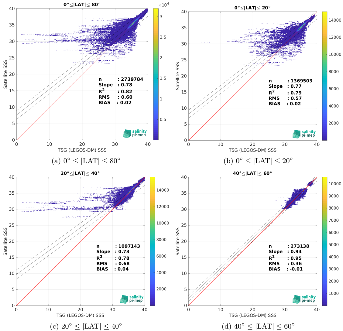
Figure 9: Contour maps of the concentration of SMAP SSS L4 OI v2 - Monthly (IPRC) SSS (y-axis) versus TSG (LEGOS-DM) SSS (x-axis) at match-up pairs for different latitude bands. For each plot, the red line shows x=y . The black thin and dashed lines indicate a linear fit through the data cloud and the \pm 95\% confidence levels, respectively. The number match-up pairs n , the slope and R^2 coefficient of the linear fit, the root mean square (RMS) and the mean bias between satellite and in situ data are indicated for each latitude band in each plots.
