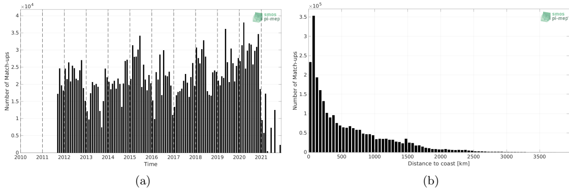
Figure 1: Number of match-ups between TSG (LEGOS-DM) and SMAP SSS L4 OI v2 - Monthly (IPRC) SSS as a function of time (a) and as function of the distance to coast (b) over the Mid-Low Latitudes 45N-45S Pi-MEP region and for the full satellite product period.
