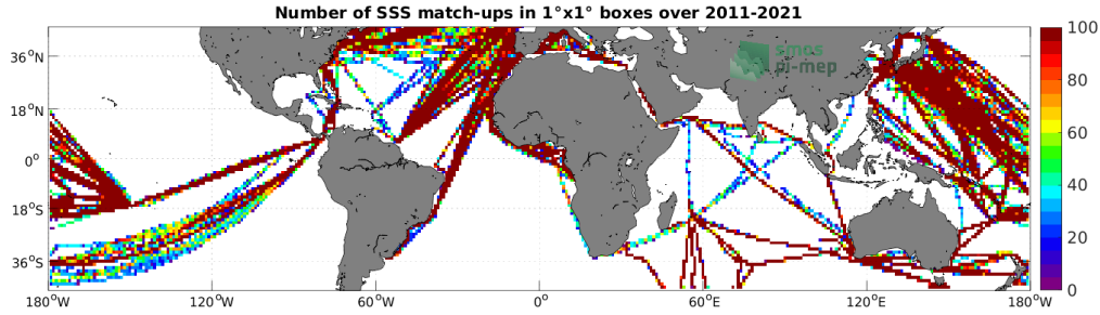
Figure 4: Number of SSS match-ups between TSG (LEGOS-DM) SSS and the SMAP SSS L4 OI v2 - Monthly (IPRC) SSS product for the Mid-Low Latitudes 45N-45S Pi-MEP region over 1^\circ \times 1^\circ boxes and for the full satellite product period.
