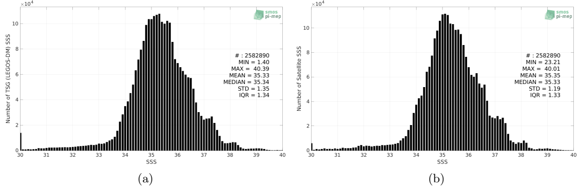
Figure 2: Histograms of SSS from TSG (LEGOS-DM) (a) and SMAP SSS L4 OI v2 - Monthly (IPRC) (b) considering all match-up pairs per bins of 0.1 over the Mid-Low Latitudes 45N-45S Pi-MEP region and for the full satellite product period.
