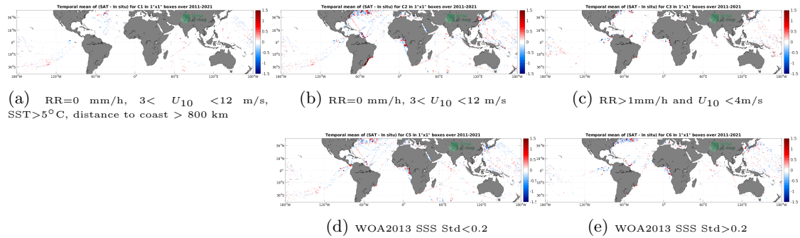
Figure 12: Temporal mean gridded over spatial boxes of size 1^\circ \times 1^\circ of \Delta SSS (SMAP SSS L4 OI v2 - Monthly (IPRC) - TSG (LEGOS-DM)) for 5 different subdatasets corresponding to:RR=0 mm/h, 3 < U_{10} < 12 m/s, SST >5^\circ\text{C} , distance to coast > 800 km (a), RR=0 mm/h, 3 < U_{10} < 12 m/s (b), RR >1 mm/h and U_{10} < 4 m/s (c), WOA2013 SSS Std <0.2 (d), WOA2013 SSS Std >0.2 (e).
