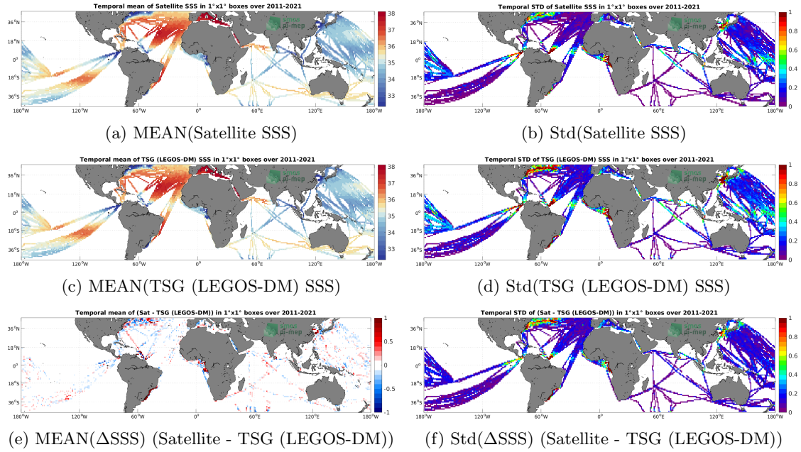
Figure 6: Temporal mean (left) and Std (right) of SSS from SMAP SSS L4 OI v2 - Monthly (IPRC) (top), TSG (LEGOS-DM) (middle), and of \Delta SSS (Satellite - TSG (LEGOS-DM)). Only match-up pairs are used to generate these maps.
