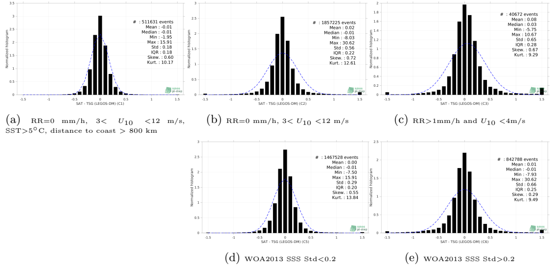
Figure 13: Normalized histogram of \Delta SSS (SMAP SSS L4 OI v2 - Monthly (IPRC) - TSG (LEGOS-DM)) for 5 different subdatasets corresponding to: RR=0 mm/h, 3 < U_{10} < 12 m/s, SST > 5°C, distance to coast > 800 km (a), RR=0 mm/h, 3 < U_{10} < 12 m/s (b), RR > 1mm/h and U_{10} < 4 m/s (c), WOA2013 SSS Std < 0.2 (d), WOA2013 SSS Std > 0.2 (e).
