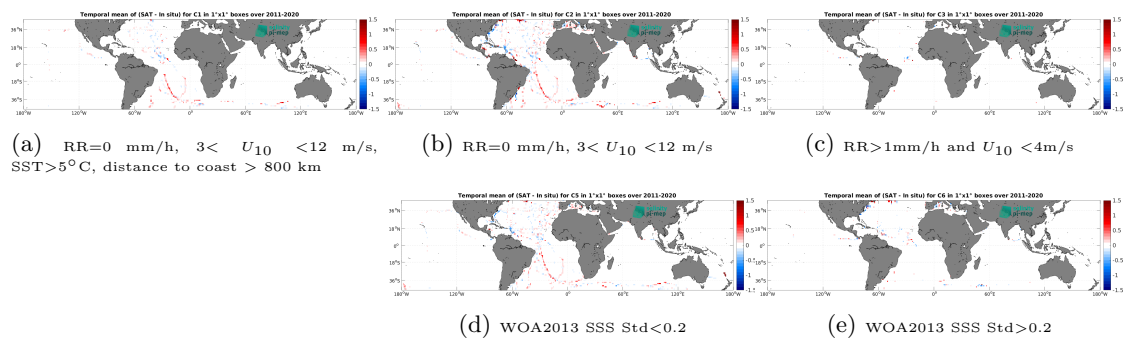
Figure 12: Temporal mean gridded over spatial boxes of size 1^\circ \times 1^\circ of \Delta SSS (SMAP SSS L4 OI v2 - Monthly (IPRC) - TSG (GOSUD-Sailing-ship)) for 5 different subdatasets corresponding to: RR=0 mm/h, 3 < U_{10} < 12 m/s, SST > 5°C, distance to coast > 800 km (a), RR=0 mm/h, 3 < U_{10} < 12 m/s (b), RR > 1mm/h and U_{10} < 4 m/s (c), WOA2013 SSS Std < 0.2 (d), WOA2013 SSS Std > 0.2 (e).
