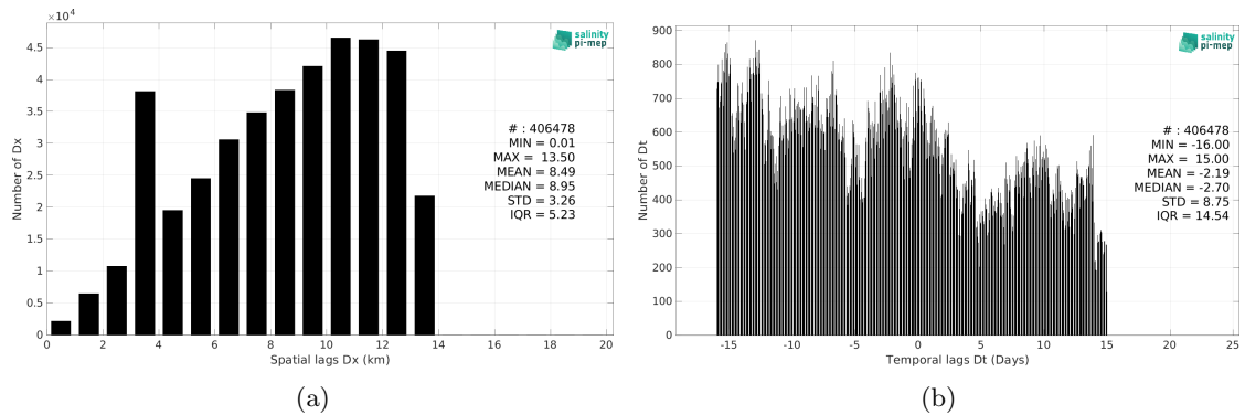
Figure 5: Histograms of the spatial (a) and temporal (b) lags between the location/time of the TSG (GOSUD-Sailing-ship) measurement and the date of the corresponding SMAP SSS L4 OI v2 - Monthly (IPRC) SSS pixel.
