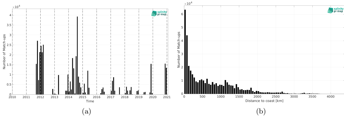
Figure 1: Number of match-ups between TSG (GOSUD-Sailing-ship) and SMAP SSS L4 OI v2 - Monthly (IPRC) SSS as a function of time (a) and as function of the distance to coast (b) over the Mid-Low Latitudes 45N-45S Pi-MEP region and for the full satellite product period.
