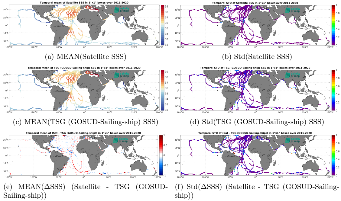
Figure 6: Temporal mean (left) and Std (right) of SSS from SMAP SSS L4 OI v2 - Monthly (IPRC) (top), TSG (GOSUD-Sailing-ship) (middle), and of \Delta SSS (Satellite - TSG (GOSUD-Sailing-ship)). Only match-up pairs are used to generate these maps.
