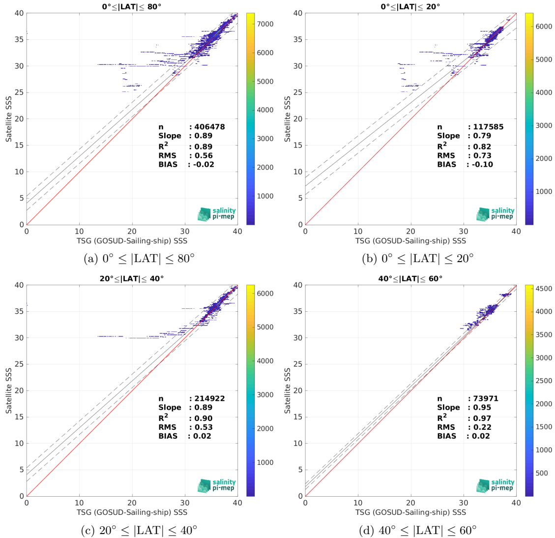
Figure 9: Contour maps of the concentration of SMAP SSS L4 OI v2 - Monthly (IPRC) SSS (y-axis) versus TSG (GOSUD-Sailing-ship) SSS (x-axis) at match-up pairs for different latitude bands. For each plot, the red line shows x=y . The black thin and dashed lines indicate a linear fit through the data cloud and the \pm 95\% confidence levels, respectively. The number match-up pairs n , the slope and R^2 coefficient of the linear fit, the root mean square (RMS) and the mean bias between satellite and in situ data are indicated for each latitude band in each plots.
