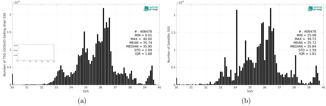
Figure 2: Histograms of SSS from TSG (GOSUD-Sailing-ship) (a) and SMAP SSS L4 OI v2 - Monthly (IPRC) (b) considering all match-up pairs per bins of 0.1 over the Mid-Low Latitudes 45N-45S Pi-MEP region and for the full satellite product period.
