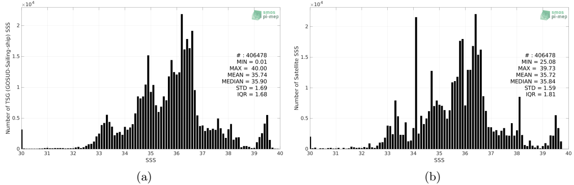
Figure 2: Histograms of SSS from TSG (GOSUD-Sailing-ship) (a) and SMAP SSS L4 OI v2 - Monthly (IPRC) (b) considering all match-up pairs per bins of 0.1 over the Mid-Low Latitudes 45N-45S Pi-MEP region and for the full satellite product period.
