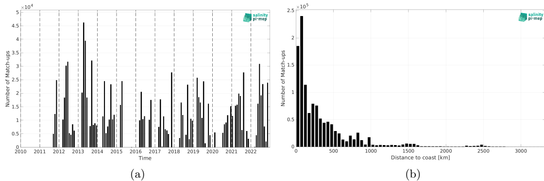
Figure 1: Number of match-ups between TSG (CSIC-UTM) and SMAP SSS L4 OI v2 - Monthly (IPRC) SSS as a function of time (a) and as function of the distance to coast (b) over the Mid-Low Latitudes 45N-45S Pi-MEP region and for the full satellite product period.
