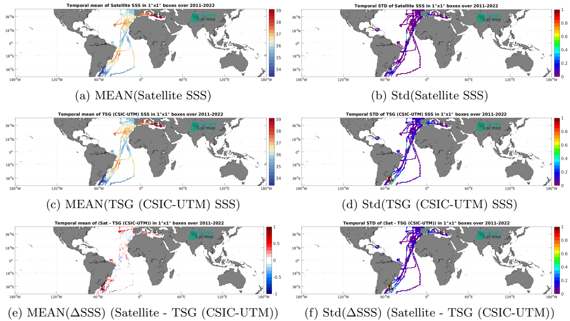
Figure 6: Temporal mean (left) and Std (right) of SSS from SMAP SSS L4 OI v2 - Monthly (IPRC) (top), TSG (CSIC-UTM) (middle), and of \Delta SSS (Satellite - TSG (CSIC-UTM)). Only match-up pairs are used to generate these maps.
