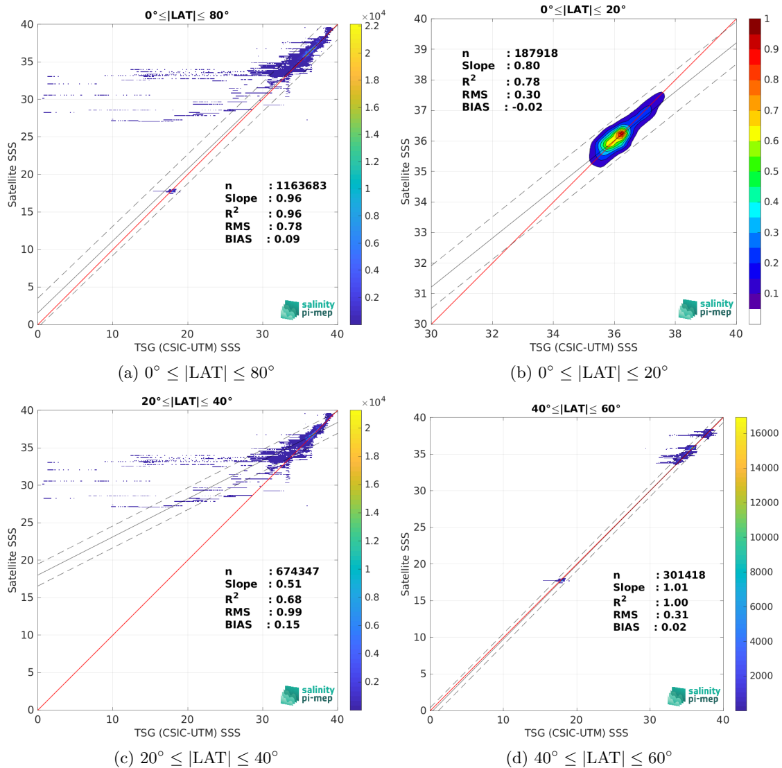
Figure 9: Contour maps of the concentration of SMAP SSS L4 OI v2 - Monthly (IPRC) SSS (y-axis) versus TSG (CSIC-UTM) SSS (x-axis) at match-up pairs for different latitude bands. For each plot, the red line shows x=y . The black thin and dashed lines indicate a linear fit through the data cloud and the \pm 95\% confidence levels, respectively. The number match-up pairs n , the slope and R^2 coefficient of the linear fit, the root mean square (RMS) and the mean bias between satellite and in situ data are indicated for each latitude band in each plots.
