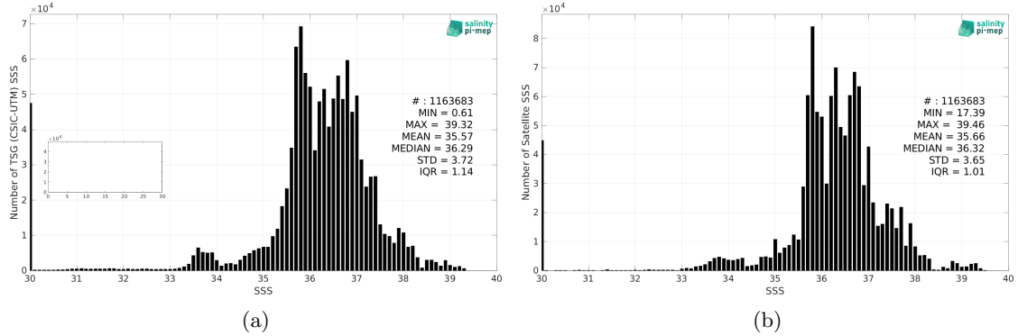
Figure 2: Histograms of SSS from TSG (CSIC-UTM) (a) and SMAP SSS L4 OI v2 - Monthly (IPRC) (b) considering all match-up pairs per bins of 0.1 over the Mid-Low Latitudes 45N-45S Pi-MEP region and for the full satellite product period.
