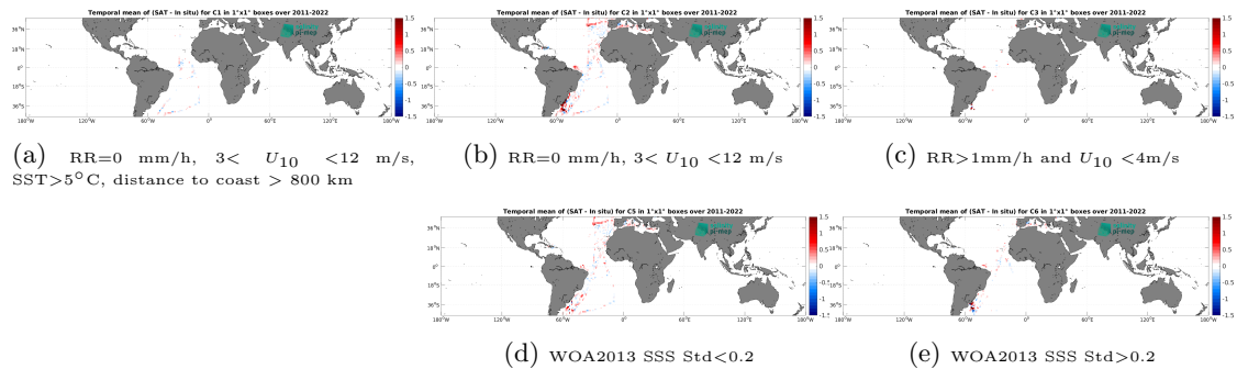
Figure 12: Temporal mean gridded over spatial boxes of size 1^\circ \times 1^\circ of \Delta SSS (SMAP SSS L4 OI v2 - Monthly (IPRC) - TSG (CSIC-UTM)) for 5 different subdatasets corresponding to:RR=0 mm/h, 3 < U_{10} < 12 m/s, SST > 5^\circ C , distance to coast > 800 km (a), RR=0 mm/h, 3 < U_{10} < 12 m/s (b), RR >1 mm/h and U_{10} < 4 m/s (c), WOA2013 SSS Std <0.2 (d), WOA2013 SSS Std >0.2 (e).
