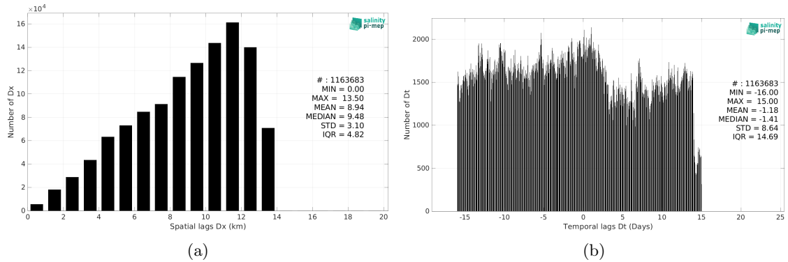
Figure 5: Histograms of the spatial (a) and temporal (b) lags between the location/time of the TSG (CSIC-UTM) measurement and the date of the corresponding SMAP SSS L4 OI v2 - Monthly (IPRC) SSS pixel.
