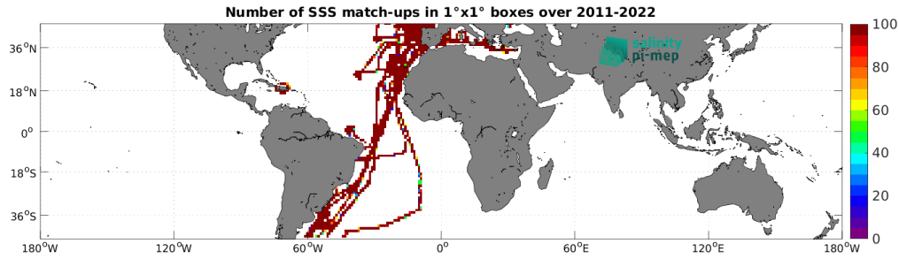
Figure 4: Number of SSS match-ups between TSG (CSIC-UTM) SSS and the SMAP SSS L4 OI v2 - Monthly (IPRC) SSS product for the Mid-Low Latitudes 45N-45S Pi-MEP region over 1^\circ \times 1^\circ boxes and for the full satellite product period.
