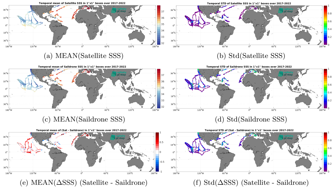
Figure 6: Temporal mean (left) and Std (right) of SSS from SMAP SSS L4 OI v2 - Monthly (IPRC) (top), Saildrone (middle), and of \Delta SSS (Satellite - Saildrone). Only match-up pairs are used to generate these maps.
