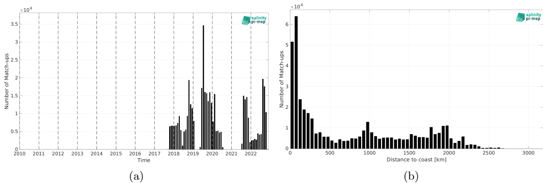
Figure 1: Number of match-ups between Saildrone and SMAP SSS L4 OI v2 - Monthly (IPRC) SSS as a function of time (a) and as function of the distance to coast (b) over the Mid-Low Latitudes 45N-45S Pi-MEP region and for the full satellite product period.
