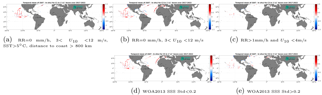
Figure 12: Temporal mean gridded over spatial boxes of size 1^\circ \times 1^\circ of \Delta SSS (SMAP SSS L4 OI v2 - Monthly (IPRC) - Saildrone) for 5 different subdatasets corresponding to: RR=0 mm/h, 3 < U_{10} < 12 m/s, SST >5^\circ\text{C} , distance to coast > 800 km (a), RR=0 mm/h, 3 < U_{10} < 12 m/s (b), RR >1 mm/h and U_{10} < 4 m/s (c), WOA2013 SSS Std <0.2 (d), WOA2013 SSS Std >0.2 (e).
