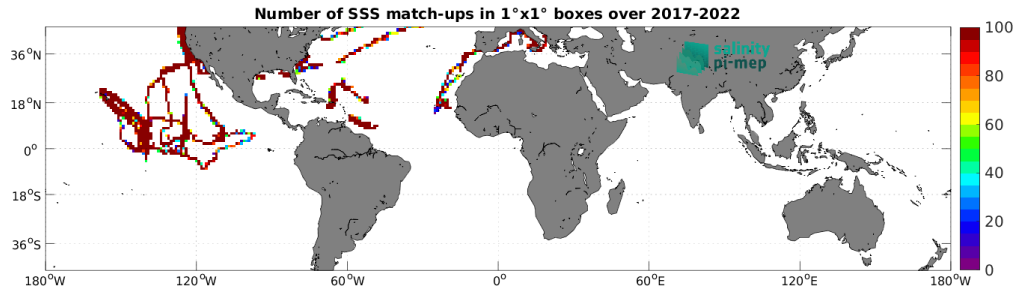
Figure 4: Number of SSS match-ups between Saildrone SSS and the SMAP SSS L4 OI v2 - Monthly (IPRC) SSS product for the Mid-Low Latitudes 45N-45S Pi-MEP region over 1^\circ \times 1^\circ boxes and for the full satellite product period.
