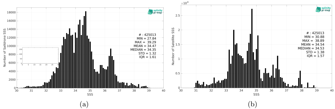
Figure 2: Histograms of SSS from Saildrone (a) and SMAP SSS L4 OI v2 - Monthly (IPRC) (b) considering all match-up pairs per bins of 0.1 over the Mid-Low Latitudes 45N-45S Pi-MEP region and for the full satellite product period.
