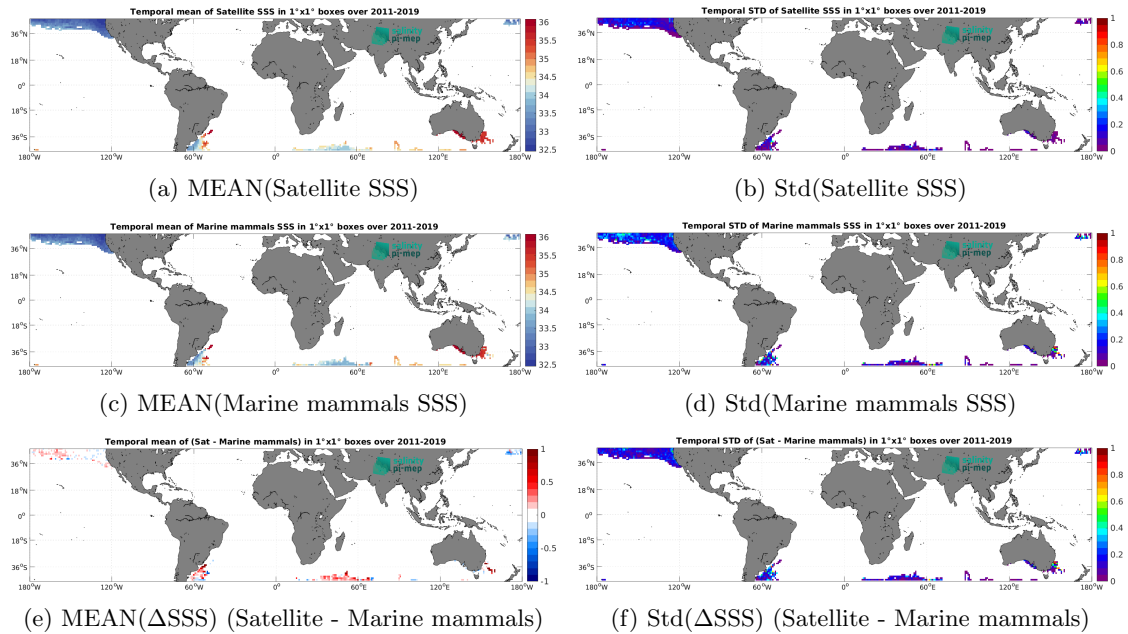
Figure 6: Temporal mean (left) and Std (right) of SSS from SMAP SSS L4 OI v2 - Monthly (IPRC) (top), Marine mammals (middle), and of \Delta SSS (Satellite - Marine mammals). Only match-up pairs are used to generate these maps.
