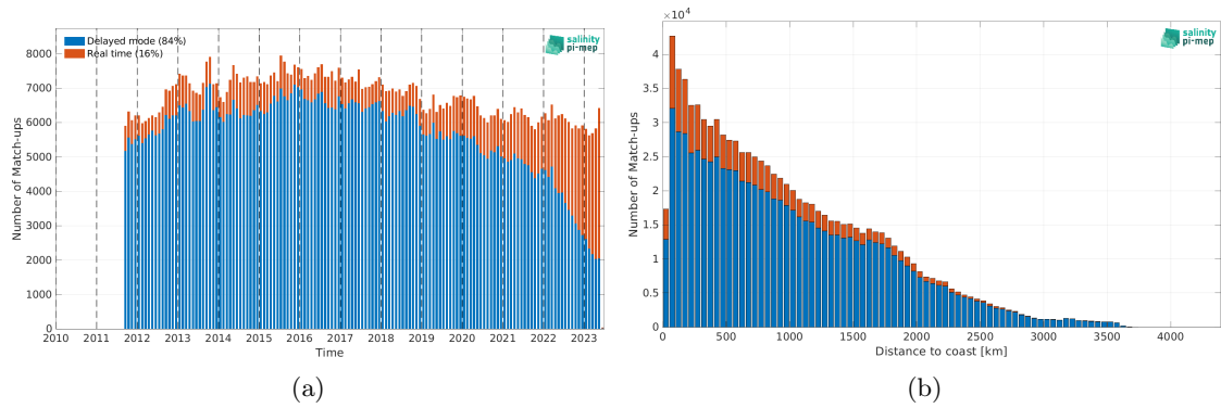
Figure 1: Number of match-ups between Argo and SMAP SSS L4 OI v2 - Monthly (IPRC) SSS as a function of time (a) and as function of the distance to coast (b) over the Mid-Low Latitudes 45N-45S Pi-MEP region and for the full satellite product period.
