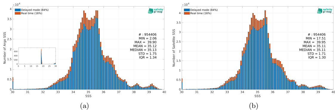
Figure 2: Histograms of SSS from Argo (a) and SMAP SSS L4 OI v2 - Monthly (IPRC) (b) considering all match-up pairs per bins of 0.1 over the Mid-Low Latitudes 45N-45S Pi-MEP region and for the full satellite product period.
