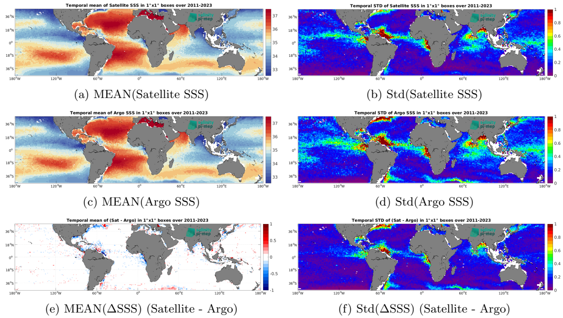
Figure 6: Temporal mean (left) and Std (right) of SSS from SMAP SSS L4 OI v2 - Monthly (IPRC) (top), Argo (middle), and of \Delta SSS (Satellite - Argo). Only match-up pairs are used to generate these maps.
