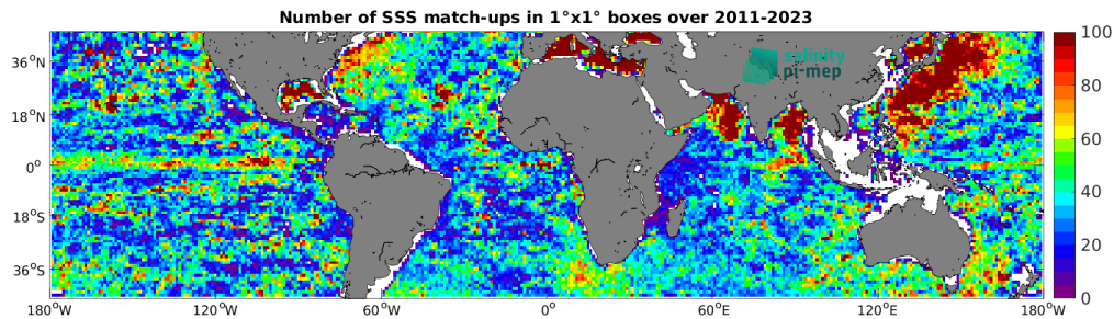
Figure 4: Number of SSS match-ups between Argo SSS and the SMAP SSS L4 OI v2 - Monthly (IPRC) SSS product for the Mid-Low Latitudes 45N-45S Pi-MEP region over 1^\circ \times 1^\circ boxes and for the full satellite product period.
