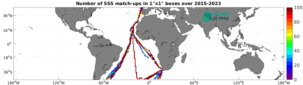
Figure 5: Number of SSS match-ups between TSG (Polarstern) SSS and the SMAP SSS L3 v6 - 8-Day running (RSS) SSS product for the Mid-Low Latitudes 45N-45S Pi-MEP region over 1^\circ \times 1^\circ boxes and for the full satellite product period.
