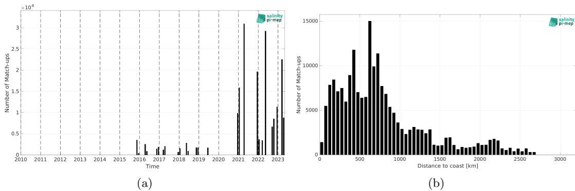
Figure 2: Number of match-ups between TSG (Polarstern) and SMAP SSS L3 v6 - 8-Day running (RSS) SSS as a function of time (a) and as function of the distance to coast (b) over the Mid-Low Latitudes 45N-45S Pi-MEP region and for the full satellite product period.
