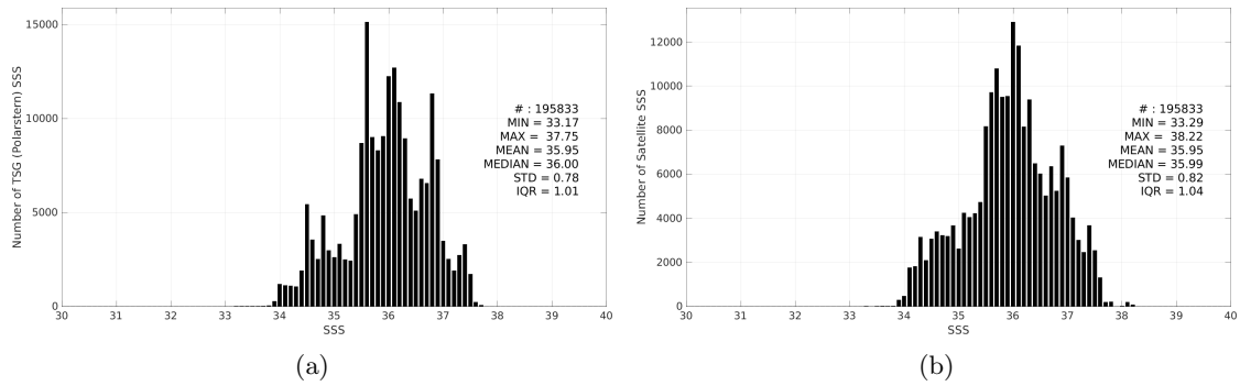
Figure 3: Histograms of SSS from TSG (Polarstern) (a) and SMAP SSS L3 v6 - 8-Day running (RSS) (b) considering all match-up pairs per bins of 0.1 over the Mid-Low Latitudes 45N-45S Pi-MEP region and for the full satellite product period.
