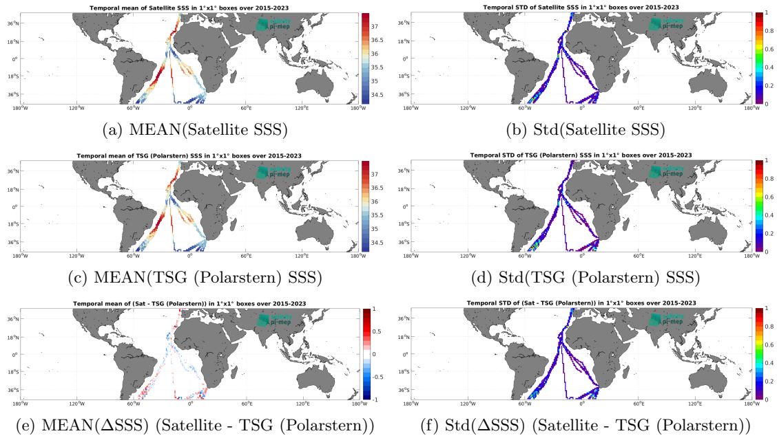
Figure 7: Temporal mean (left) and Std (right) of SSS from SMAP SSS L3 v6 - 8-Day running (RSS) (top), TSG (Polarstern) (middle), and of \Delta SSS (Satellite - TSG (Polarstern)). Only match-up pairs are used to generate these maps.
