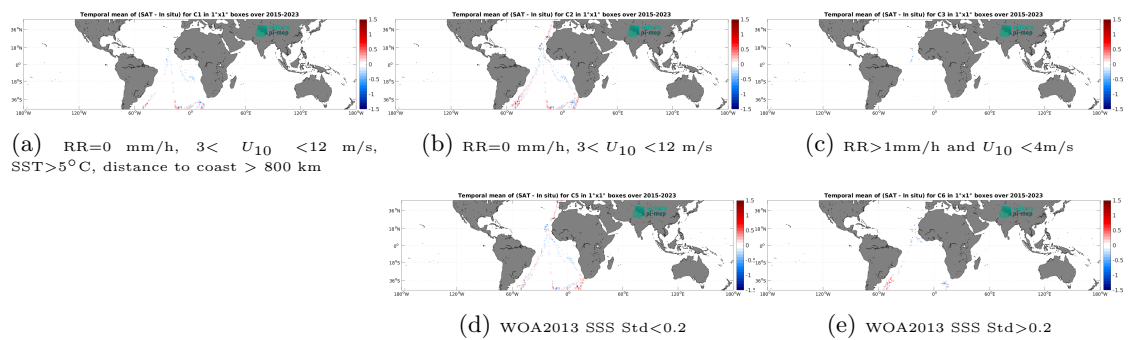
Figure 14: Temporal mean gridded over spatial boxes of size 1^\circ \times 1^\circ of \Delta\text{SSS} (SMAP SSS L3 v6 - 8-Day running (RSS) - TSG (Polarstern)) for 5 different subdatasets corresponding to: RR=0 mm/h, 3 < U_{10} < 12 m/s, SST > 5°C, distance to coast > 800 km (a), RR=0 mm/h, 3 < U_{10} < 12 m/s (b), RR > 1mm/h and U_{10} < 4 m/s (c), WOA2013 SSS Std < 0.2 (d), WOA2013 SSS Std > 0.2 (e).
