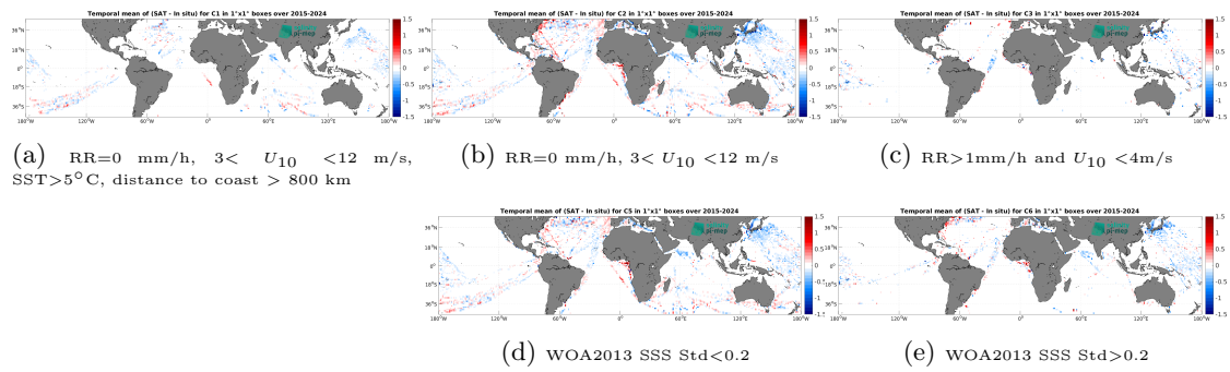
Figure 14: Temporal mean gridded over spatial boxes of size 1^\circ \times 1^\circ of \Delta\text{SSS} (SMAP SSS L3 v6 - 8-Day running (RSS) - TSG (LEGOS-DM)) for 5 different subdatasets corresponding to: RR=0 mm/h, 3 < U_{10} < 12 m/s, SST > 5°C, distance to coast > 800 km (a), RR=0 mm/h, 3 < U_{10} < 12 m/s (b), RR > 1mm/h and U_{10} < 4 m/s (c), WOA2013 SSS Std < 0.2 (d), WOA2013 SSS Std > 0.2 (e).
