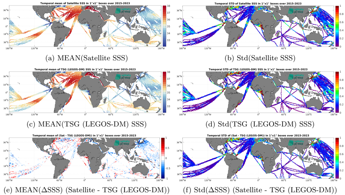
Figure 7: Temporal mean (left) and Std (right) of SSS from SMAP SSS L3 v6 - 8-Day running (RSS) (top), TSG (LEGOS-DM) (middle), and of \Delta SSS (Satellite - TSG (LEGOS-DM)). Only match-up pairs are used to generate these maps.
