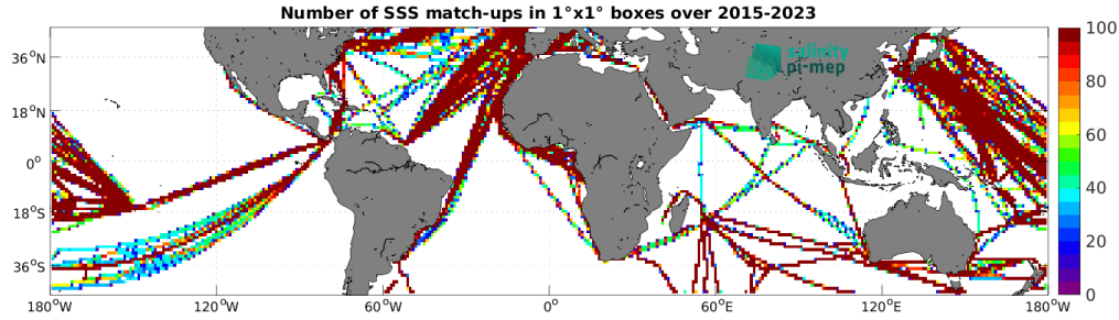
Figure 5: Number of SSS match-ups between TSG (LEGOS-DM) SSS and the SMAP SSS L3 v6 - 8-Day running (RSS) SSS product for the Mid-Low Latitudes 45N-45S Pi-MEP region over 1^\circ \times 1^\circ boxes and for the full satellite product period.
