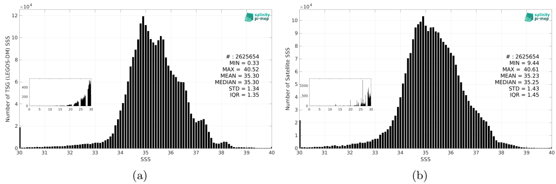
Figure 3: Histograms of SSS from TSG (LEGOS-DM) (a) and SMAP SSS L3 v6 - 8-Day running (RSS) (b) considering all match-up pairs per bins of 0.1 over the Mid-Low Latitudes 45N-45S Pi-MEP region and for the full satellite product period.
