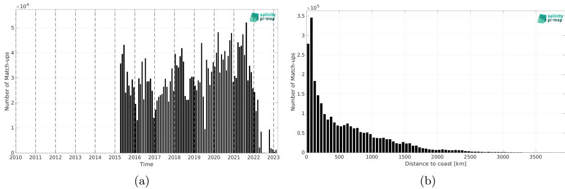
Figure 2: Number of match-ups between TSG (LEGOS-DM) and SMAP SSS L3 v6 - 8-Day running (RSS) SSS as a function of time (a) and as function of the distance to coast (b) over the Mid-Low Latitudes 45N-45S Pi-MEP region and for the full satellite product period.
