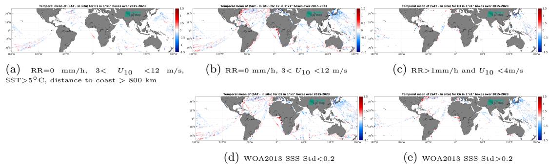
Figure 14: Temporal mean gridded over spatial boxes of size 1^\circ \times 1^\circ of \Delta SSS (SMAP SSS L3 v6 - 8-Day running (RSS) - TSG (LEGOS-DM)) for 5 different subdatasets corresponding to:RR=0 mm/h, 3 < U_{10} < 12 m/s, SST >5^\circ\text{C} , distance to coast > 800 km (a), RR=0 mm/h, 3 < U_{10} < 12 m/s (b), RR >1 mm/h and U_{10} < 4 m/s (c), WOA2013 SSS Std <0.2 (d), WOA2013 SSS Std >0.2 (e).
