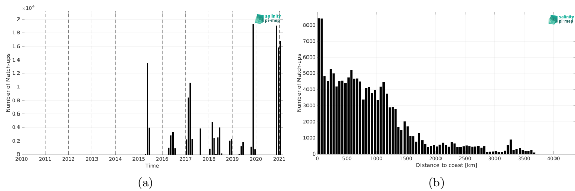
Figure 2: Number of match-ups between TSG (GOSUD-Sailing-ship) and SMAP SSS L3 v6 - 8-Day running (RSS) SSS as a function of time (a) and as function of the distance to coast (b) over the Mid-Low Latitudes 45N-45S Pi-MEP region and for the full satellite product period.
