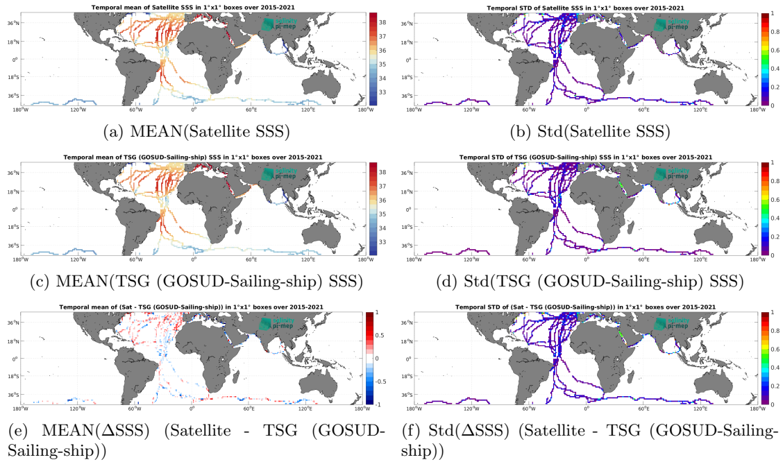
Figure 7: Temporal mean (left) and Std (right) of SSS from SMAP SSS L3 v6 - 8-Day running (RSS) (top), TSG (GOSUD-Sailing-ship) (middle), and of \Delta SSS (Satellite - TSG (GOSUD-Sailing-ship)). Only match-up pairs are used to generate these maps.
