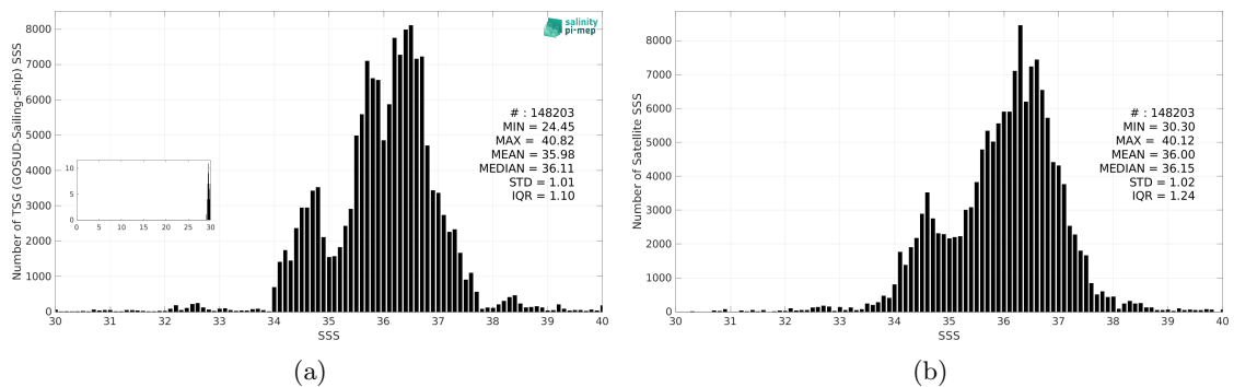
Figure 3: Histograms of SSS from TSG (GOSUD-Sailing-ship) (a) and SMAP SSS L3 v6 - 8-Day running (RSS) (b) considering all match-up pairs per bins of 0.1 over the Mid-Low Latitudes 45N-45S Pi-MEP region and for the full satellite product period.
