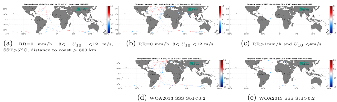
Figure 14: Temporal mean gridded over spatial boxes of size 1^\circ \times 1^\circ of \Delta SSS (SMAP SSS L3 v6 - 8-Day running (RSS) - TSG (GOSUD-Sailing-ship)) for 5 different subdatasets corresponding to:RR=0 mm/h, 3 < U_{10} < 12 m/s, SST>5°C, distance to coast > 800 km (a), RR=0 mm/h, 3 < U_{10} < 12 m/s (b), RR>1mm/h and U_{10} < 4 m/s (c), WOA2013 SSS Std<0.2 (d), WOA2013 SSS Std>0.2 (e).
