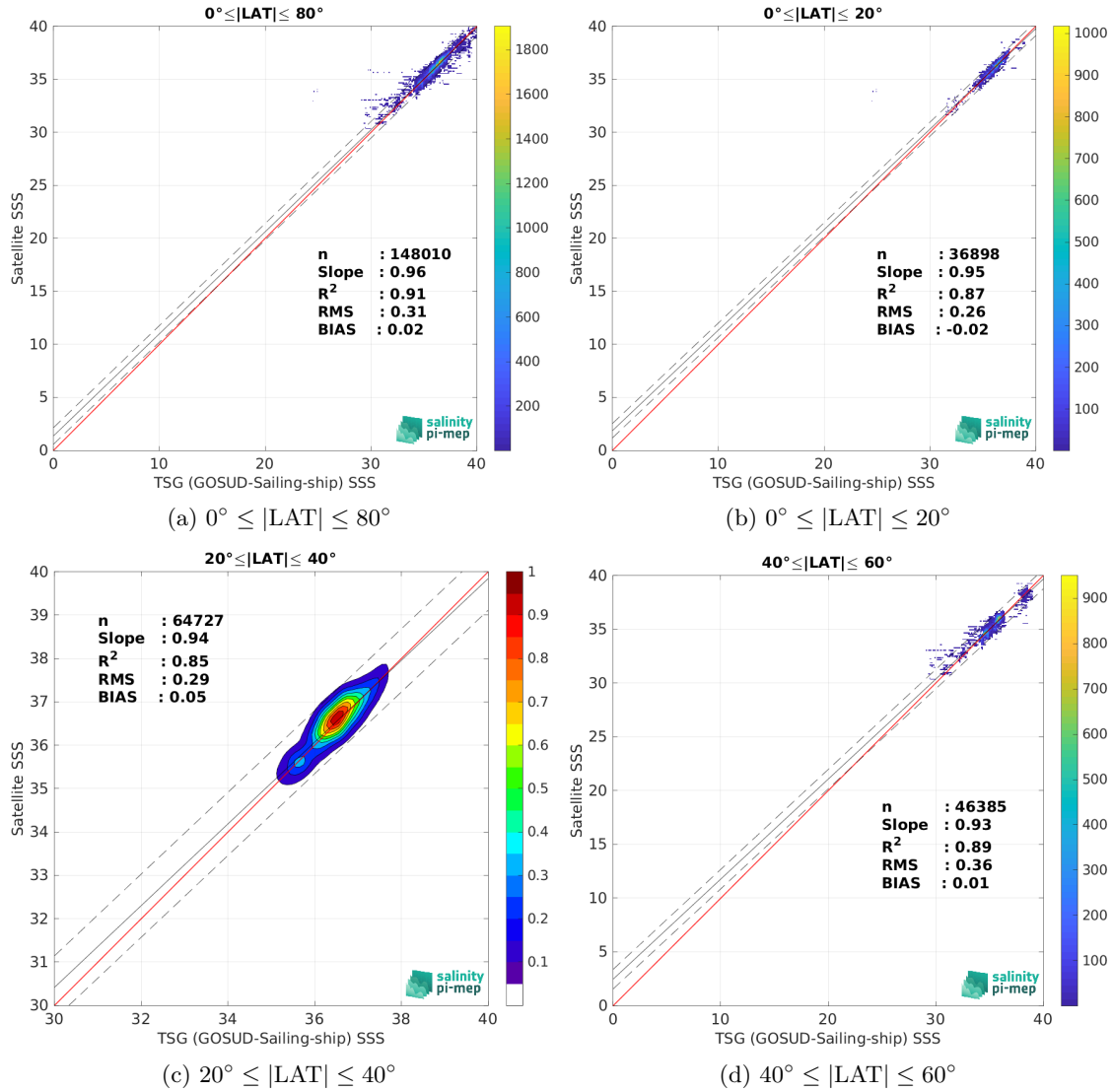
Figure 10: Contour maps of the concentration of SMAP SSS L3 v6 - 8-Day running (RSS) SSS (y-axis) versus TSG (GOSUD-Sailing-ship) SSS (x-axis) at match-up pairs for different latitude bands. For each plot, the red line shows x=y . The black thin and dashed lines indicate a linear fit through the data cloud and the \pm 95\% confidence levels, respectively. The number match-up pairs n , the slope and R^2 coefficient of the linear fit, the root mean square (RMS) and the mean bias between satellite and in situ data are indicated for each latitude band in each plots.
