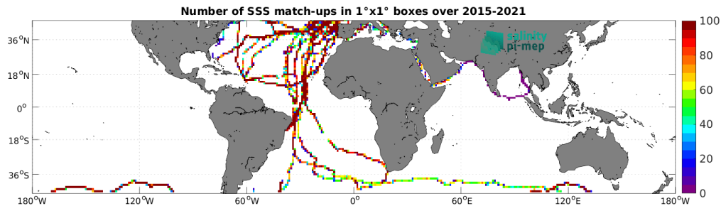
Figure 5: Number of SSS match-ups between TSG (GOSUD-Sailing-ship) SSS and the SMAP SSS L3 v6 - 8-Day running (RSS) SSS product for the Mid-Low Latitudes 45N-45S Pi-MEP region over 1^\circ \times 1^\circ boxes and for the full satellite product period.
