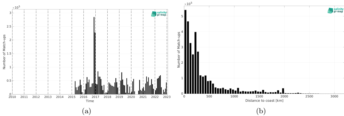
Figure 2: Number of match-ups between TSG (GOSUD-Research-vessel) and SMAP SSS L3 v6 - 8-Day running (RSS) SSS as a function of time (a) and as function of the distance to coast (b) over the Mid-Low Latitudes 45N-45S Pi-MEP region and for the full satellite product period.
