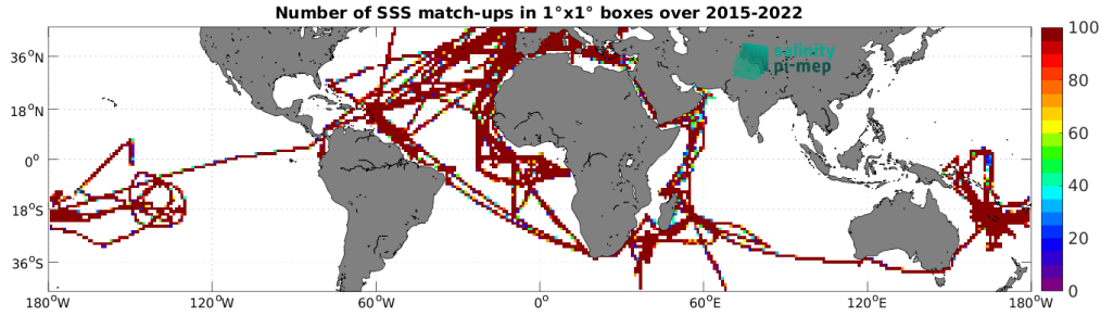
Figure 5: Number of SSS match-ups between TSG (GOSUD-Research-vessel) SSS and the SMAP SSS L3 v6 - 8-Day running (RSS) SSS product for the Mid-Low Latitudes 45N-45S Pi-MEP region over 1^\circ \times 1^\circ boxes and for the full satellite product period.
