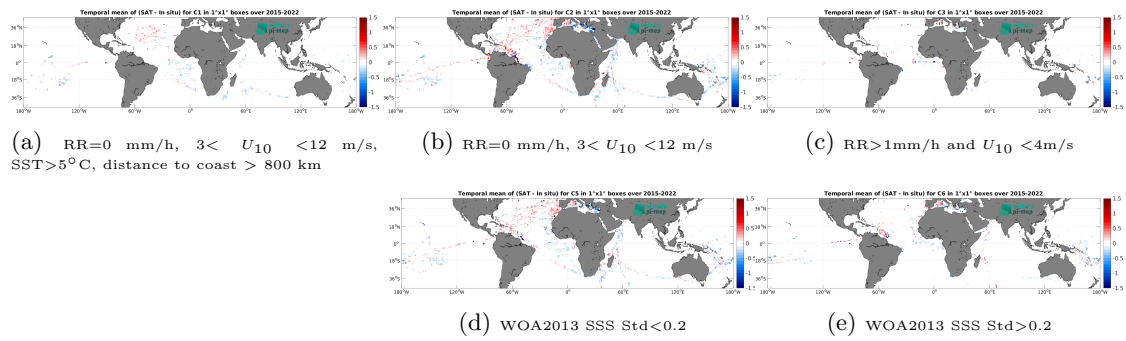
Figure 14: Temporal mean gridded over spatial boxes of size 1^\circ \times 1^\circ of \Delta\text{SSS} (SMAP SSS L3 v6 - 8-Day running (RSS) - TSG (GOSUD-Research-vessel)) for 5 different subdatasets corresponding to:RR=0 mm/h, 3 < U_{10} < 12 m/s, SST >5^\circ\text{C} , distance to coast > 800 km (a), RR=0 mm/h, 3 < U_{10} < 12 m/s (b), RR >1 mm/h and U_{10} < 4 m/s (c), WOA2013 SSS Std <0.2 (d), WOA2013 SSS Std >0.2 (e).
