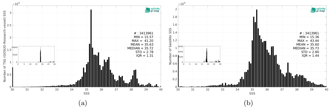
Figure 3: Histograms of SSS from TSG (GOSUD-Research-vessel) (a) and SMAP SSS L3 v6 - 8-Day running (RSS) (b) considering all match-up pairs per bins of 0.1 over the Mid-Low Latitudes 45N-45S Pi-MEP region and for the full satellite product period.
