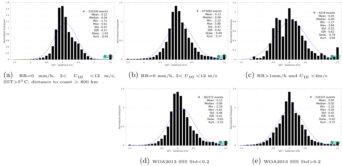
Figure 15: Normalized histogram of \Delta SSS (SMAP SSS L3 v6 - 8-Day running (RSS) - Sairdron) for 5 different subdatasets corresponding to: RR=0 mm/h, 3 < U_{10} < 12 m/s, SST>5°C, distance to coast > 800 km (a), RR=0 mm/h, 3 < U_{10} < 12 m/s (b), RR>1mm/h and U_{10} < 4 m/s (c), WOA2013 SSS Std<0.2 (d), WOA2013 SSS Std>0.2 (e).
