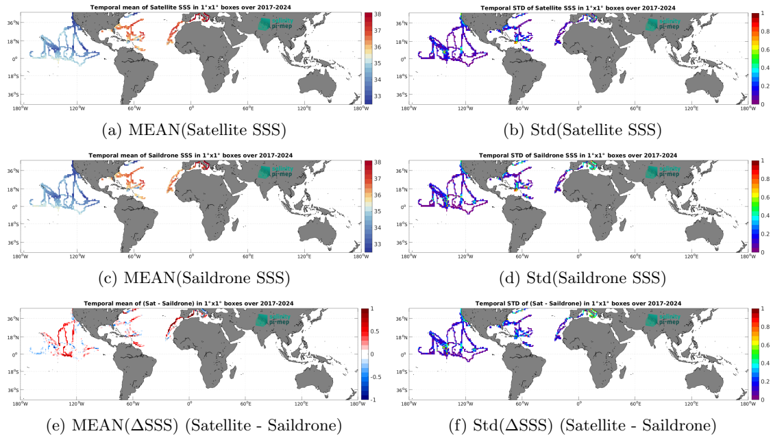
Figure 7: Temporal mean (left) and Std (right) of SSS from SMAP SSS L3 v6 - 8-Day running (RSS) (top), Saildrone (middle), and of \Delta SSS (Satellite - Saildrone). Only match-up pairs are used to generate these maps.
