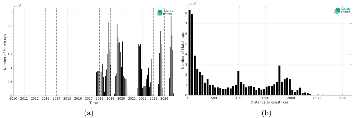
Figure 2: Number of match-ups between Saildrone and SMAP SSS L3 v6 - 8-Day running (RSS) SSS as a function of time (a) and as function of the distance to coast (b) over the Mid-Low Latitudes 45N-45S Pi-MEP region and for the full satellite product period.
