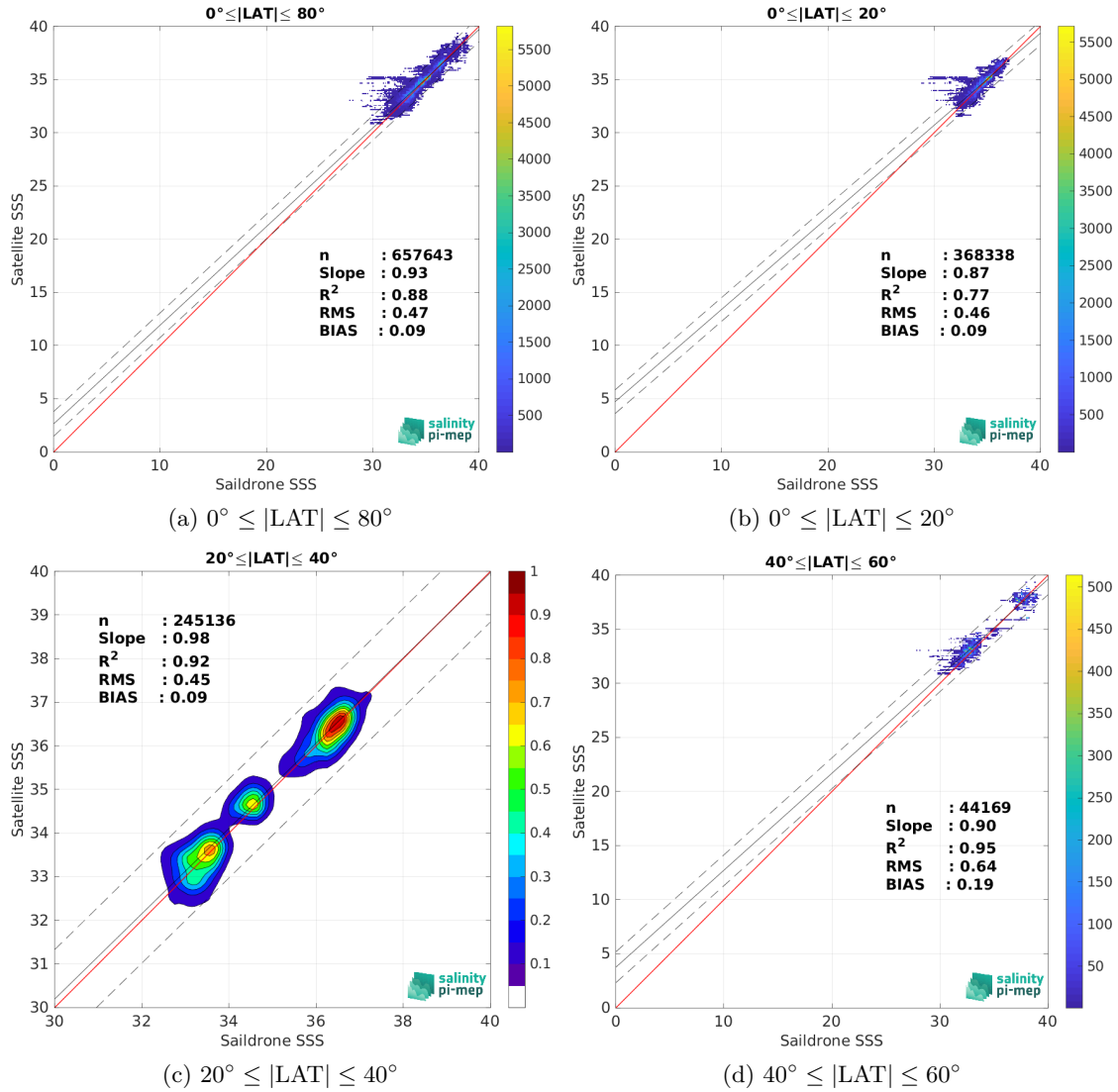
Figure 10: Contour maps of the concentration of SMAP SSS L3 v6 - 8-Day running (RSS) SSS (y-axis) versus Sairdrone SSS (x-axis) at match-up pairs for different latitude bands. For each plot, the red line shows x=y . The black thin and dashed lines indicate a linear fit through the data cloud and the \pm 95\% confidence levels, respectively. The number match-up pairs n , the slope and R^2 coefficient of the linear fit, the root mean square (RMS) and the mean bias between satellite and in situ data are indicated for each latitude band in each plots.
