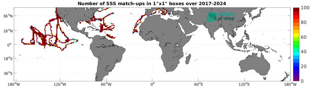
Figure 5: Number of SSS match-ups between Saildrone SSS and the SMAP SSS L3 v6 - 8-Day running (RSS) SSS product for the Mid-Low Latitudes 45N-45S Pi-MEP region over 1^\circ \times 1^\circ boxes and for the full satellite product period.
