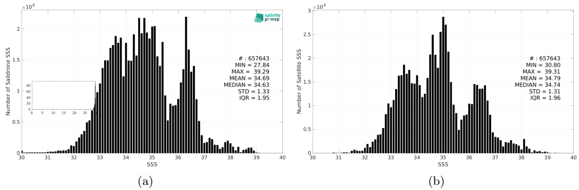
Figure 3: Histograms of SSS from Saildrone (a) and SMAP SSS L3 v6 - 8-Day running (RSS) (b) considering all match-up pairs per bins of 0.1 over the Mid-Low Latitudes 45N-45S Pi-MEP region and for the full satellite product period.
