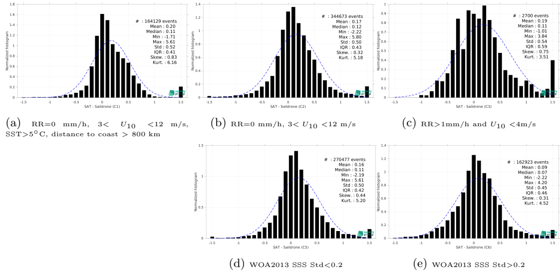
Figure 15: Normalized histogram of \Delta SSS (SMAP SSS L3 v6 - 8-Day running (RSS) - Sairdrone) for 5 different subdatasets corresponding to: RR=0 mm/h, 3 < U_{10} < 12 m/s, SST > 5°C, distance to coast > 800 km (a), RR=0 mm/h, 3 < U_{10} < 12 m/s (b), RR > 1mm/h and U_{10} < 4 m/s (c), WOA2013 SSS Std < 0.2 (d), WOA2013 SSS Std > 0.2 (e).
