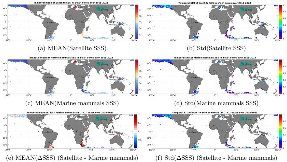
Figure 7: Temporal mean (left) and Std (right) of SSS from SMAP SSS L3 v6 - 8-Day running (RSS) (top), Marine mammals (middle), and of \Delta SSS (Satellite - Marine mammals). Only match-up pairs are used to generate these maps.
