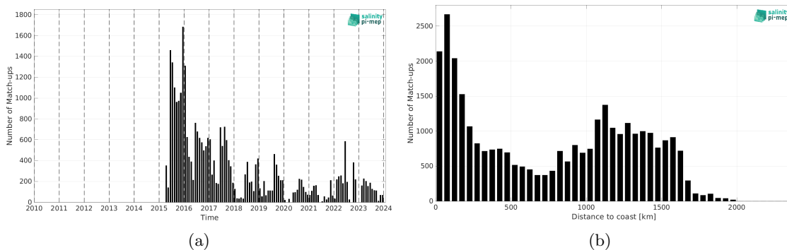
Figure 2: Number of match-ups between Marine mammals and SMAP SSS L3 v6 - 8-Day running (RSS) SSS as a function of time (a) and as function of the distance to coast (b) over the Mid-Low Latitudes 45N-45S Pi-MEP region and for the full satellite product period.
