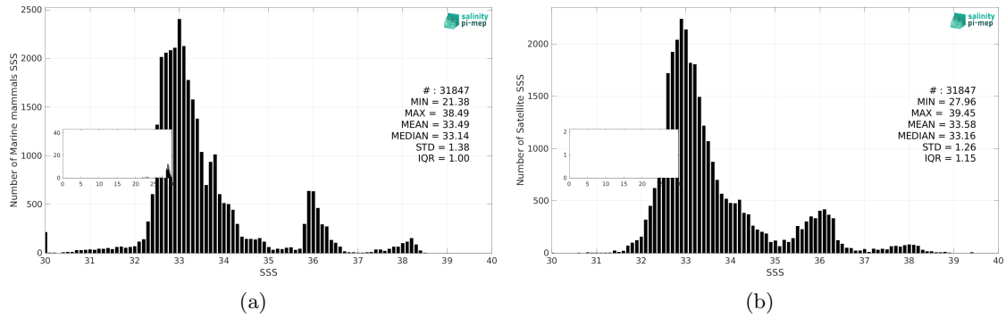
Figure 3: Histograms of SSS from Marine mammals (a) and SMAP SSS L3 v6 - 8-Day running (RSS) (b) considering all match-up pairs per bins of 0.1 over the Mid-Low Latitudes 45N-45S Pi-MEP region and for the full satellite product period.
