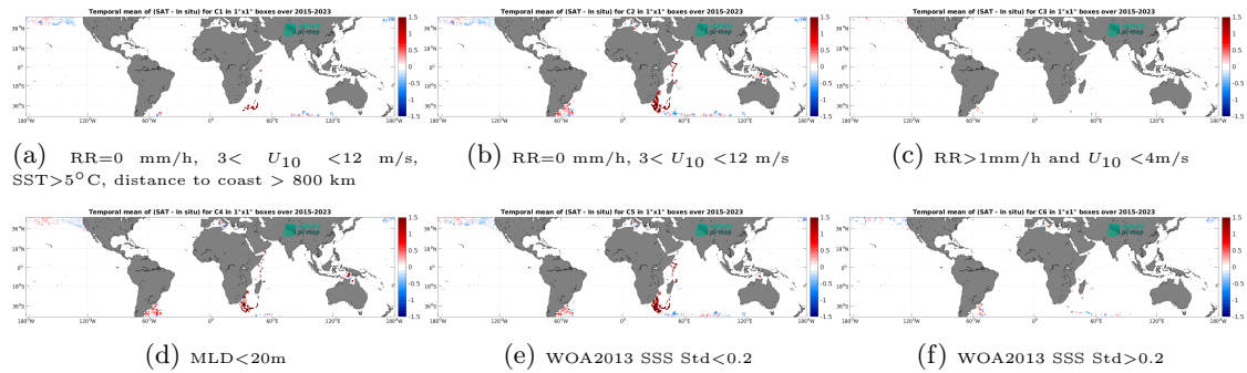
Figure 14: Temporal mean gridded over spatial boxes of size 1^\circ \times 1^\circ of \Delta SSS (SMAP SSS L3 v6 - 8-Day running (RSS) - Marine mammals) for 6 different subdatasets corresponding to:RR=0 mm/h, 3 < U_{10} < 12 m/s, SST > 5°C, distance to coast > 800 km (a), RR=0 mm/h, 3 < U_{10} < 12 m/s (b), RR > 1mm/h and U_{10} < 4 m/s (c),MLD < 20m (d),WOA2013 SSS Std < 0.2 (e),WOA2013 SSS Std > 0.2 (f).
