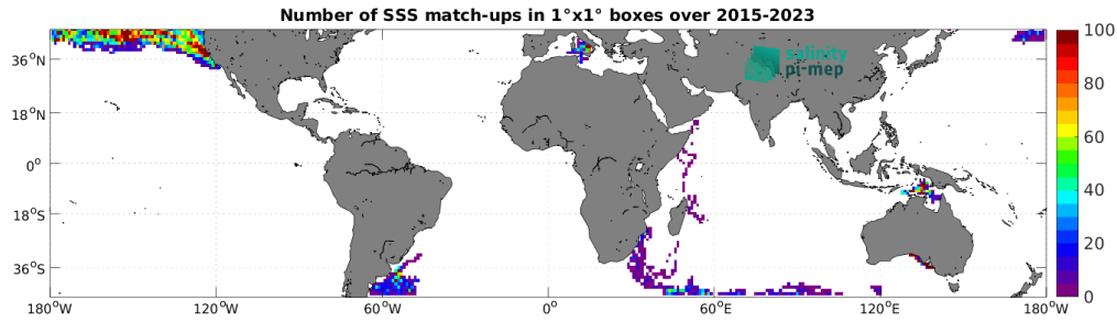
Figure 5: Number of SSS match-ups between Marine mammals SSS and the SMAP SSS L3 v6 - 8-Day running (RSS) SSS product for the Mid-Low Latitudes 45N-45S Pi-MEP region over 1^{\circ} \times 1^{\circ} boxes and for the full satellite product period.
