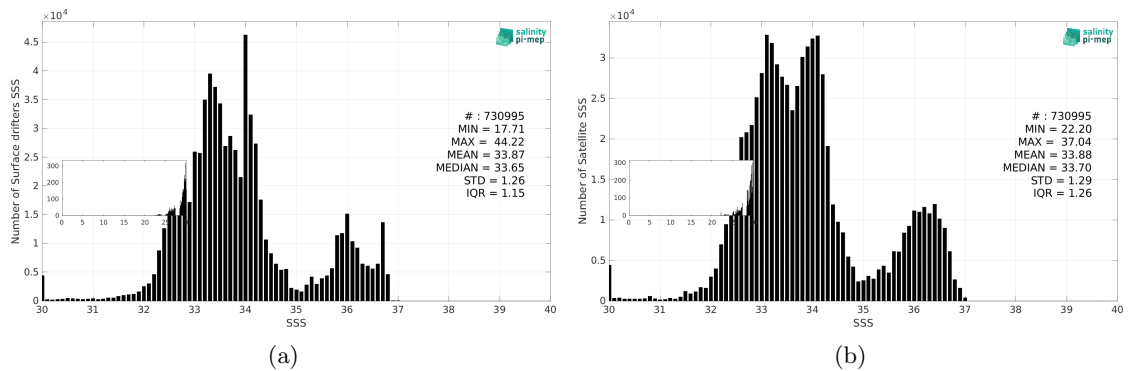
Figure 3: Histograms of SSS from Surface drifters (a) and SMAP SSS L3 v6 - 8-Day running (RSS) (b) considering all match-up pairs per bins of 0.1 over the Mid-Low Latitudes 45N-45S Pi-MEP region and for the full satellite product period.
