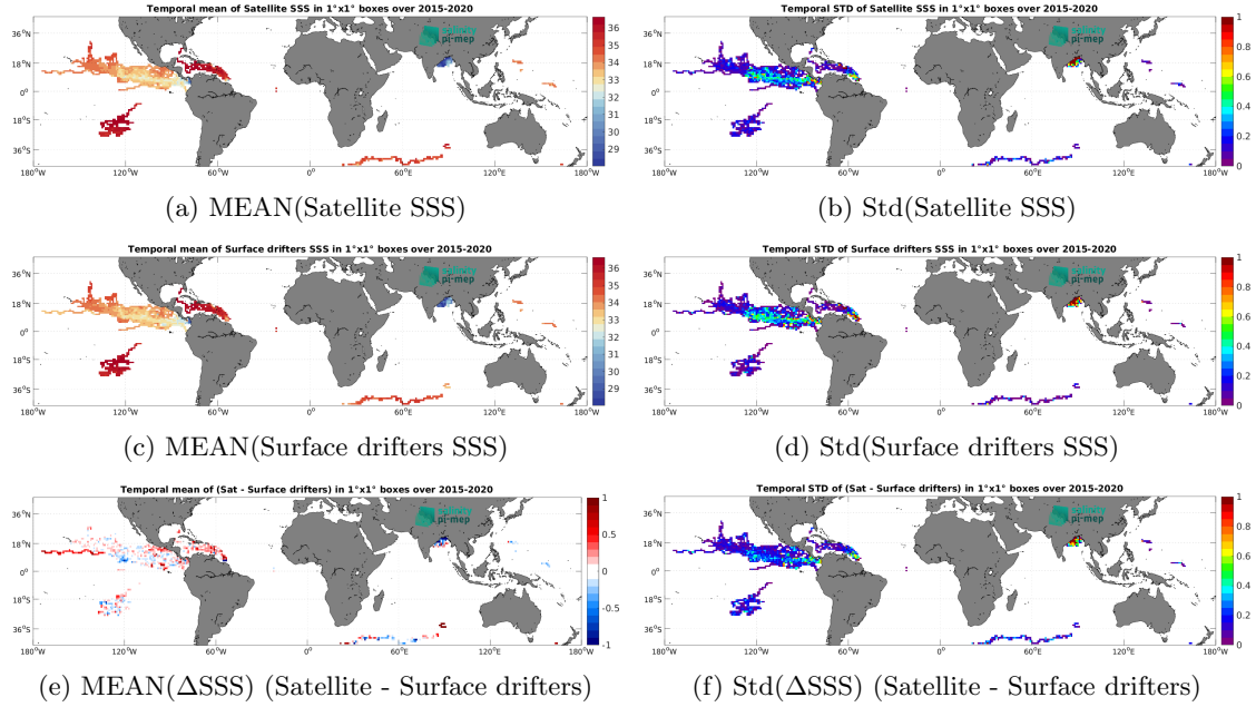
Figure 6: Temporal mean (left) and Std (right) of SSS from SMAP SSS L3 v6 - 8-Day running (RSS) (top), Surface drifters (middle), and of \Delta SSS (Satellite - Surface drifters). Only match-up pairs are used to generate these maps.
