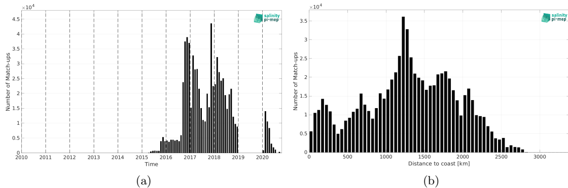
Figure 2: Number of match-ups between Surface drifters and SMAP SSS L3 v6 - 8-Day running (RSS) SSS as a function of time (a) and as function of the distance to coast (b) over the Mid-Low Latitudes 45N-45S Pi-MEP region and for the full satellite product period.
