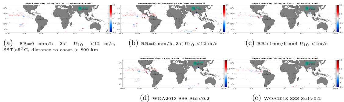
Figure 13: Temporal mean gridded over spatial boxes of size 1^\circ \times 1^\circ of \Delta SSS (SMAP SSS L3 v6 - 8-Day running (RSS) - Surface drifters) for 5 different subdatasets corresponding to:RR=0 mm/h, 3 < U_{10} < 12 m/s, SST >5^\circ\text{C} , distance to coast > 800 km (a), RR=0 mm/h, 3 < U_{10} < 12 m/s (b), RR >1 mm/h and U_{10} < 4 m/s (c), WOA2013 SSS Std <0.2 (d), WOA2013 SSS Std >0.2 (e).
