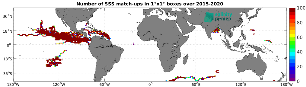
Figure 4: Number of SSS match-ups between Surface drifters SSS and the SMAP SSS L3 v6 - 8-Day running (RSS) SSS product for the Mid-Low Latitudes 45N-45S Pi-MEP region over 1^\circ \times 1^\circ boxes and for the full satellite product period.
