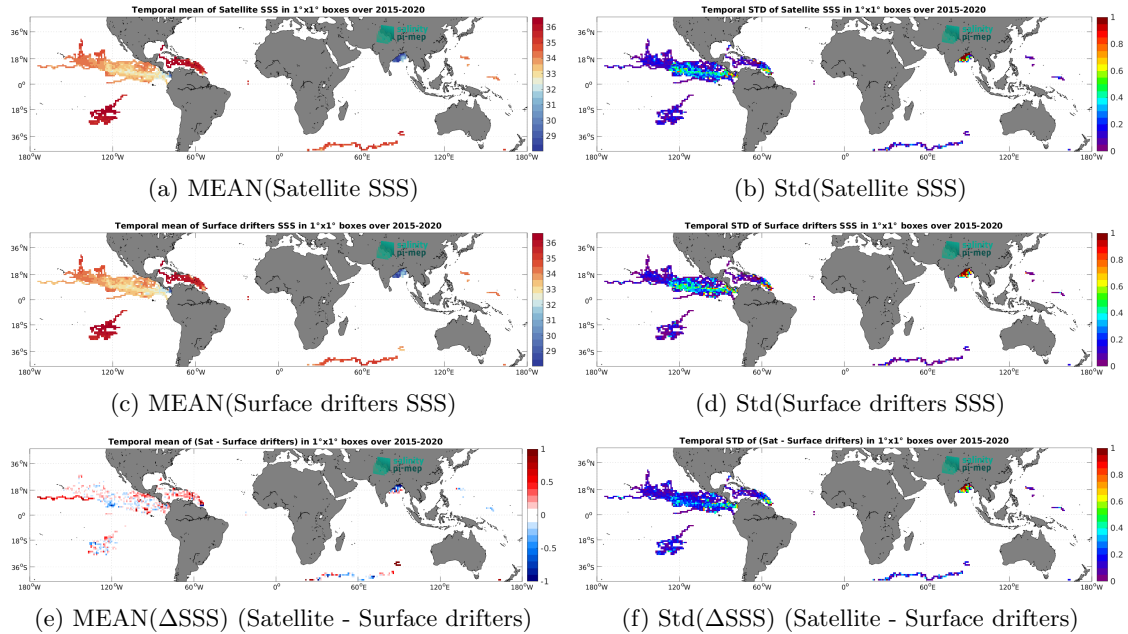
Figure 6: Temporal mean (left) and Std (right) of SSS from SMAP SSS L3 v6 - 8-Day running (RSS) (top), Surface drifters (middle), and of \Delta SSS (Satellite - Surface drifters). Only match-up pairs are used to generate these maps.
