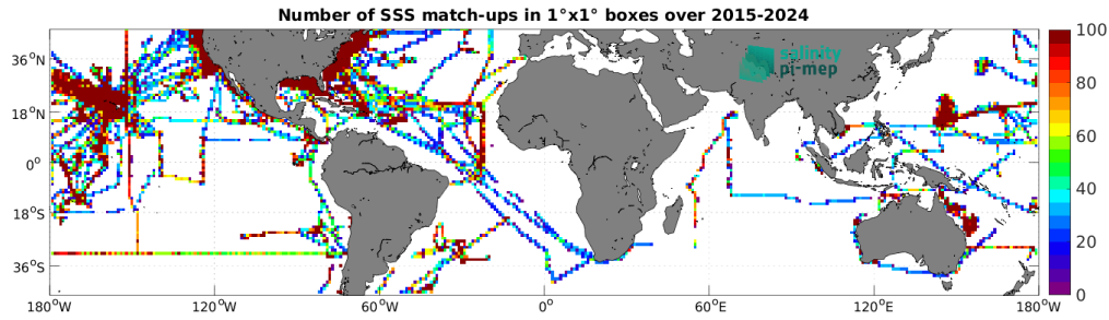
Figure 5: Number of SSS match-ups between TSG (SAMOS) SSS and the SMAP SSS L3 v6 - Monthly (RSS) SSS product for the Mid-Low Latitudes 45N-45S Pi-MEP region over 1^\circ \times 1^\circ boxes and for the full satellite product period.
