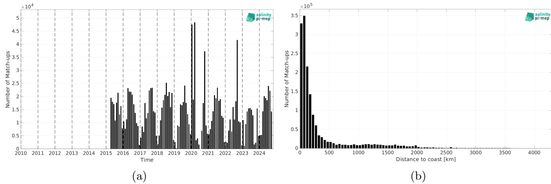
Figure 2: Number of match-ups between TSG (SAMOS) and SMAP SSS L3 v6 - Monthly (RSS) SSS as a function of time (a) and as function of the distance to coast (b) over the Mid-Low Latitudes 45N-45S Pi-MEP region and for the full satellite product period.
