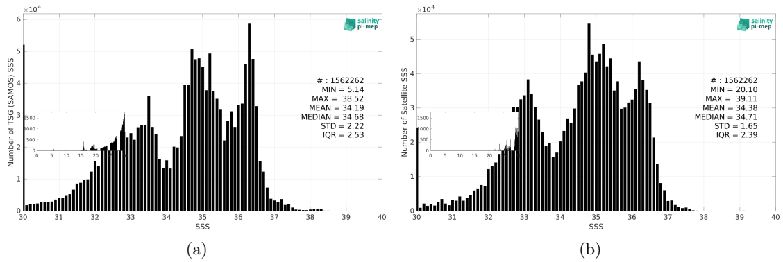
Figure 3: Histograms of SSS from TSG (SAMOS) (a) and SMAP SSS L3 v6 - Monthly (RSS) (b) considering all match-up pairs per bins of 0.1 over the Mid-Low Latitudes 45N-45S Pi-MEP region and for the full satellite product period.
