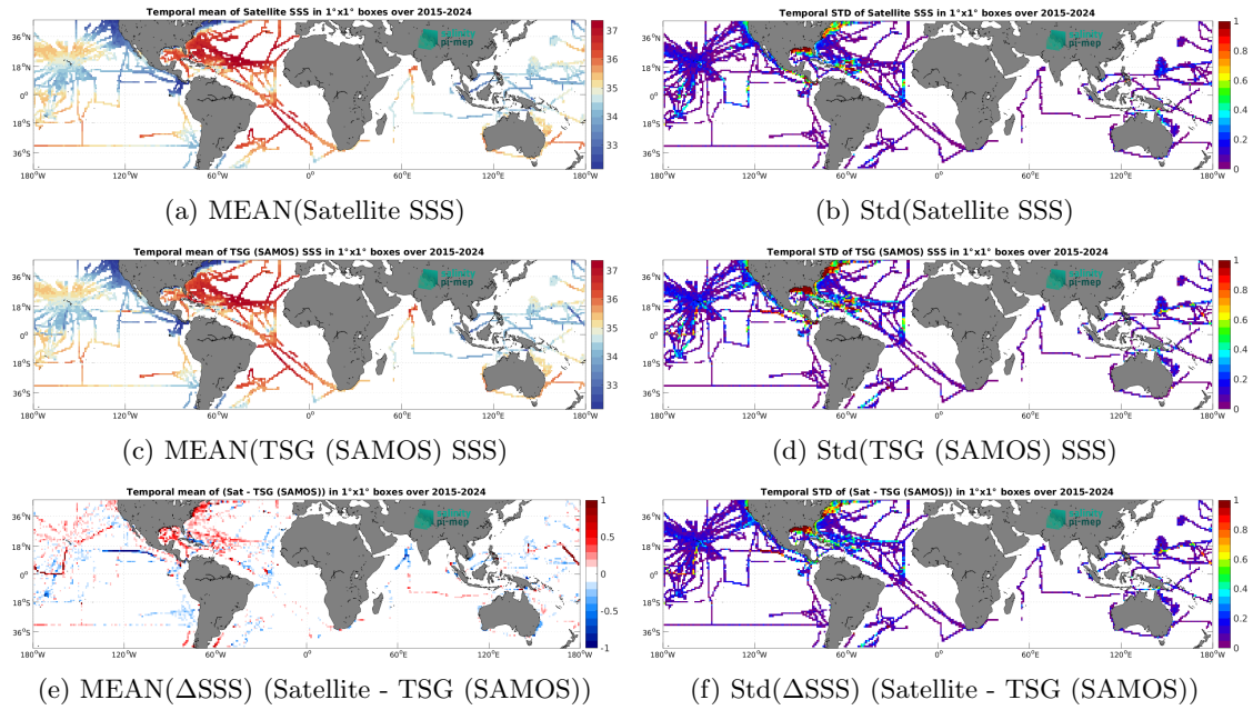
Figure 7: Temporal mean (left) and Std (right) of SSS from SMAP SSS L3 v6 - Monthly (RSS) (top), TSG (SAMOS) (middle), and of \Delta SSS (Satellite - TSG (SAMOS)). Only match-up pairs are used to generate these maps.
