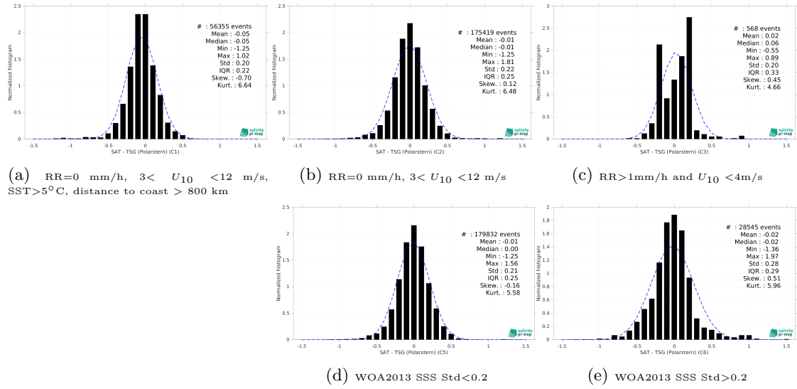
Figure 15: Normalized histogram of \Delta\text{SSS} (SMAP SSS L3 v6 - Monthly (RSS) - TSG (Polarstern)) for 5 different subdatasets corresponding to: RR=0 mm/h, 3 < U_{10} < 12 m/s, SST>5°C, distance to coast > 800 km (a), RR=0 mm/h, 3 < U_{10} < 12 m/s (b), RR>1mm/h and U_{10} < 4 m/s (c), WOA2013 SSS Std<0.2 (d), WOA2013 SSS Std>0.2 (e).
