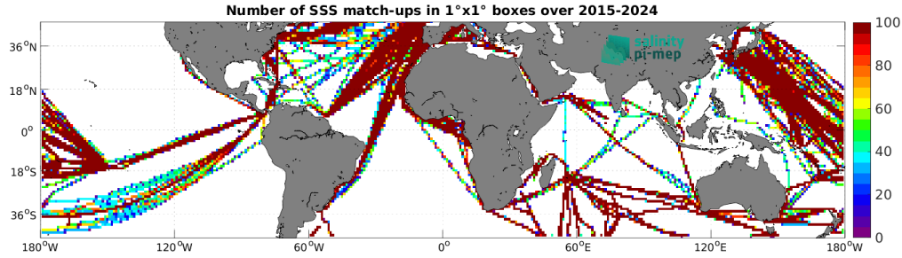
Figure 5: Number of SSS match-ups between TSG (LEGOS-DM) SSS and the SMAP SSS L3 v6 - Monthly (RSS) SSS product for the Mid-Low Latitudes 45N-45S Pi-MEP region over 1^\circ \times 1^\circ boxes and for the full satellite product period.
