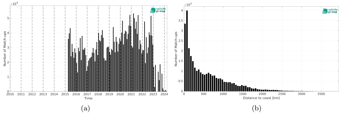
Figure 2: Number of match-ups between TSG (LEGOS-DM) and SMAP SSS L3 v6 - Monthly (RSS) SSS as a function of time (a) and as function of the distance to coast (b) over the Mid-Low Latitudes 45N-45S Pi-MEP region and for the full satellite product period.
