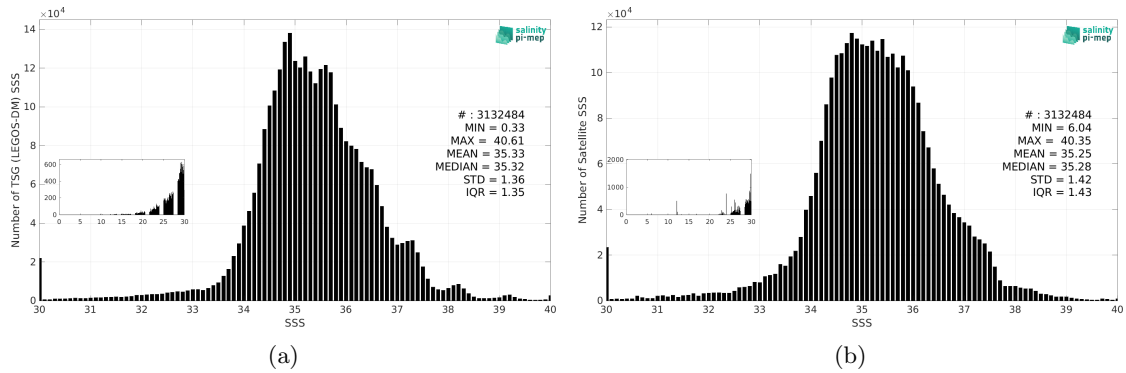
Figure 3: Histograms of SSS from TSG (LEGOS-DM) (a) and SMAP SSS L3 v6 - Monthly (RSS) (b) considering all match-up pairs per bins of 0.1 over the Mid-Low Latitudes 45N-45S Pi-MEP region and for the full satellite product period.
