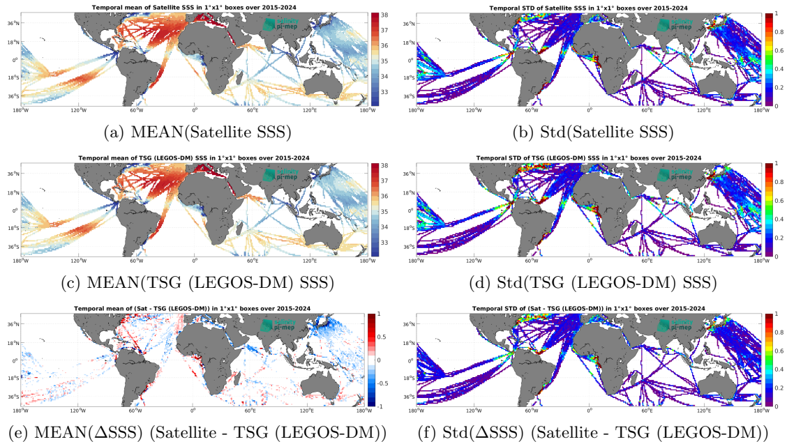
Figure 7: Temporal mean (left) and Std (right) of SSS from SMAP SSS L3 v6 - Monthly (RSS) (top), TSG (LEGOS-DM) (middle), and of \Delta SSS (Satellite - TSG (LEGOS-DM)). Only match-up pairs are used to generate these maps.
