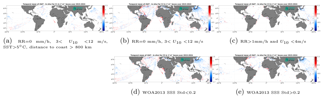
Figure 14: Temporal mean gridded over spatial boxes of size 1^\circ \times 1^\circ of \Delta\text{SSS} (SMAP SSS L3 v6 - Monthly (RSS) - TSG (LEGOS-DM)) for 5 different subdatasets corresponding to: RR=0 mm/h, 3 < U_{10} < 12 m/s, SST > 5°C, distance to coast > 800 km (a), RR=0 mm/h, 3 < U_{10} < 12 m/s (b), RR > 1mm/h and U_{10} < 4 m/s (c), WOA2013 SSS Std < 0.2 (d), WOA2013 SSS Std > 0.2 (e).
