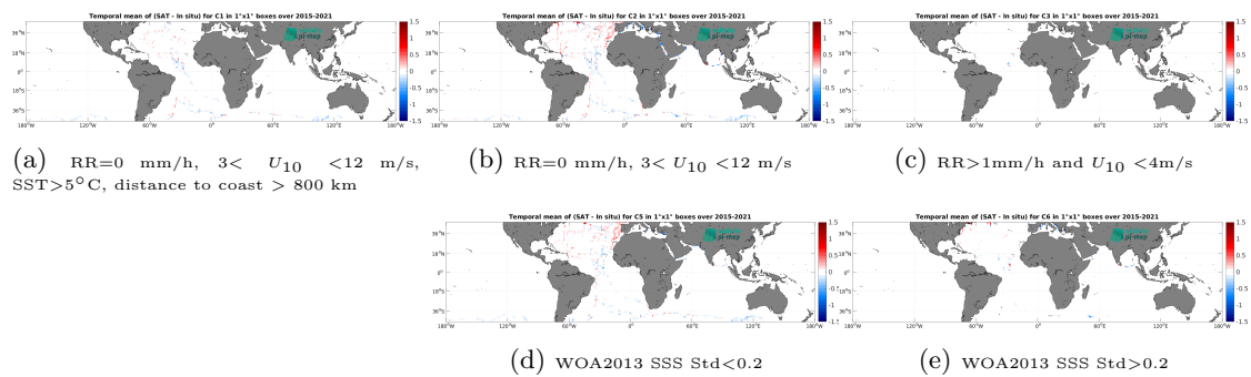
Figure 14: Temporal mean gridded over spatial boxes of size 1^\circ \times 1^\circ of \Delta\text{SSS} (SMAP SSS L3 v6 - Monthly (RSS) - TSG (GOSUD-Sailing-ship)) for 5 different subdatasets corresponding to:RR=0 mm/h, 3 < U_{10} < 12 m/s, SST > 5°C, distance to coast > 800 km (a), RR=0 mm/h, 3 < U_{10} < 12 m/s (b), RR > 1mm/h and U_{10} < 4 m/s (c), WOA2013 SSS Std < 0.2 (d), WOA2013 SSS Std > 0.2 (e).
