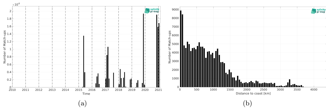
Figure 2: Number of match-ups between TSG (GOSUD-Sailing-ship) and SMAP SSS L3 v6 - Monthly (RSS) SSS as a function of time (a) and as function of the distance to coast (b) over the Mid-Low Latitudes 45N-45S Pi-MEP region and for the full satellite product period.
