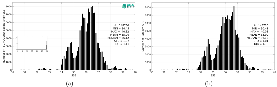
Figure 3: Histograms of SSS from TSG (GOSUD-Sailing-ship) (a) and SMAP SSS L3 v6 - Monthly (RSS) (b) considering all match-up pairs per bins of 0.1 over the Mid-Low Latitudes 45N-45S Pi-MEP region and for the full satellite product period.
