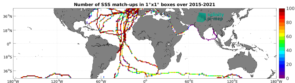
Figure 5: Number of SSS match-ups between TSG (GOSUD-Sailing-ship) SSS and the SMAP SSS L3 v6 - Monthly (RSS) SSS product for the Mid-Low Latitudes 45N-45S Pi-MEP region over 1^\circ \times 1^\circ boxes and for the full satellite product period.
