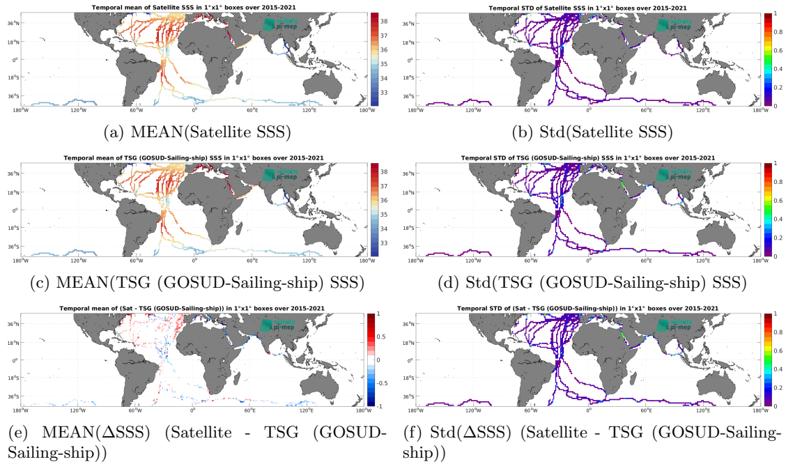
Figure 7: Temporal mean (left) and Std (right) of SSS from SMAP SSS L3 v6 - Monthly (RSS) (top), TSG (GOSUD-Sailing-ship) (middle), and of \Delta SSS (Satellite - TSG (GOSUD-Sailing-ship)). Only match-up pairs are used to generate these maps.
