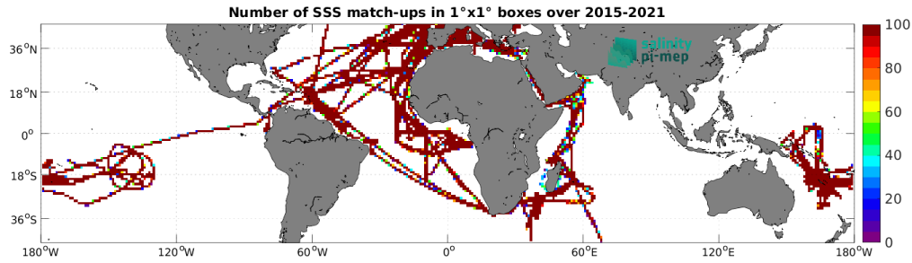
Figure 5: Number of SSS match-ups between TSG (GOSUD-Research-vessel) SSS and the SMAP SSS L3 v6 - Monthly (RSS) SSS product for the Mid-Low Latitudes 45N-45S Pi-MEP region over 1^\circ \times 1^\circ boxes and for the full satellite product period.
