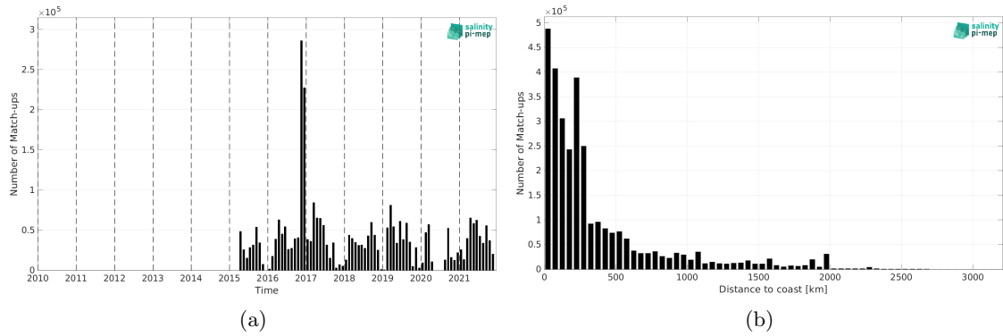
Figure 2: Number of match-ups between TSG (GOSUD-Research-vessel) and SMAP SSS L3 v6 - Monthly (RSS) SSS as a function of time (a) and as function of the distance to coast (b) over the Mid-Low Latitudes 45N-45S Pi-MEP region and for the full satellite product period.
