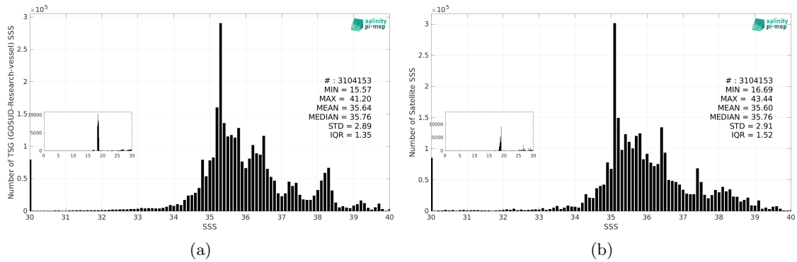
Figure 3: Histograms of SSS from TSG (GOSUD-Research-vessel) (a) and SMAP SSS L3 v6 - Monthly (RSS) (b) considering all match-up pairs per bins of 0.1 over the Mid-Low Latitudes 45N-45S Pi-MEP region and for the full satellite product period.
