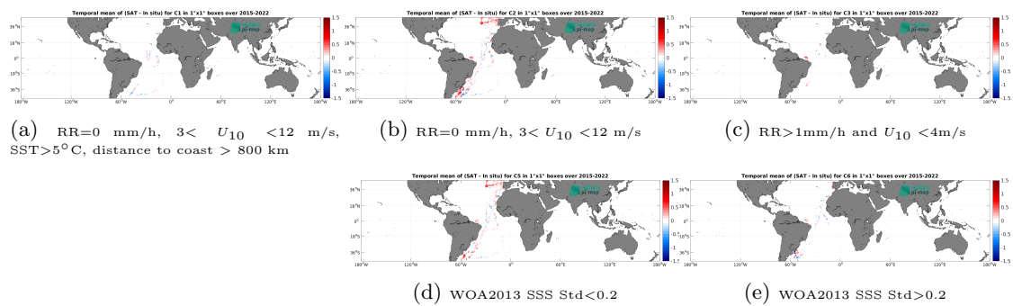
Figure 14: Temporal mean gridded over spatial boxes of size 1^\circ \times 1^\circ of \Delta\text{SSS} (SMAP SSS L3 v6 - Monthly (RSS) - TSG (CSIC-UTM)) for 5 different subdatasets corresponding to:RR=0 mm/h, 3 < U_{10} < 12 m/s, SST >5^\circ\text{C} , distance to coast > 800 km (a), RR=0 mm/h, 3 < U_{10} < 12 m/s (b), RR >1 mm/h and U_{10} < 4 m/s (c), WOA2013 SSS Std <0.2 (d), WOA2013 SSS Std >0.2 (e).
