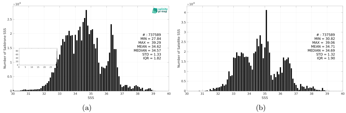
Figure 3: Histograms of SSS from Saildrone (a) and SMAP SSS L3 v6 - Monthly (RSS) (b) considering all match-up pairs per bins of 0.1 over the Mid-Low Latitudes 45N-45S Pi-MEP region and for the full satellite product period.
