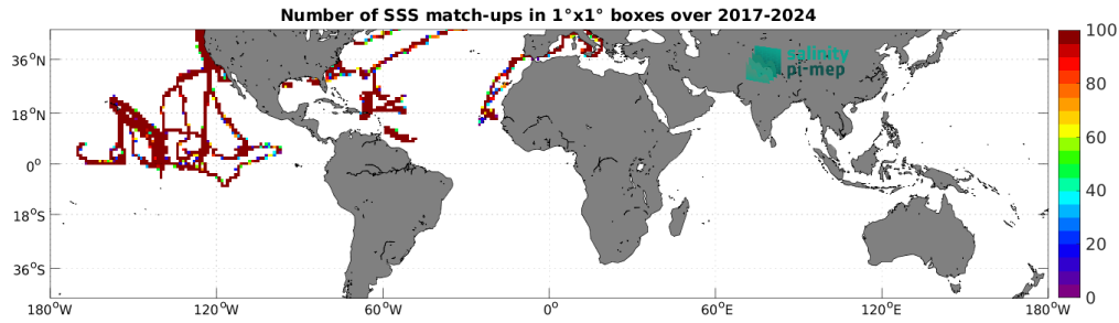
Figure 5: Number of SSS match-ups between Sailability SSS and the SMAP SSS L3 v6 - Monthly (RSS) SSS product for the Mid-Low Latitudes 45N-45S Pi-MEP region over 1^\circ \times 1^\circ boxes and for the full satellite product period.
