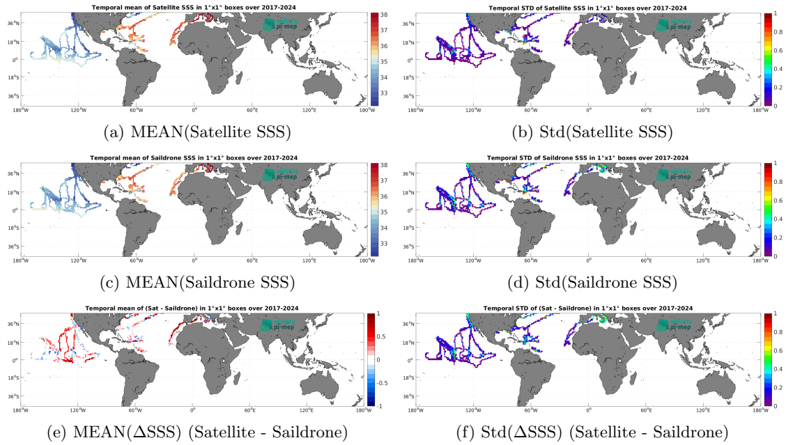
Figure 7: Temporal mean (left) and Std (right) of SSS from SMAP SSS L3 v6 - Monthly (RSS) (top), Saildrone (middle), and of \Delta SSS (Satellite - Saildrone). Only match-up pairs are used to generate these maps.
