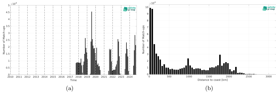
Figure 2: Number of match-ups between Saildrone and SMAP SSS L3 v6 - Monthly (RSS) SSS as a function of time (a) and as function of the distance to coast (b) over the Mid-Low Latitudes 45N-45S Pi-MEP region and for the full satellite product period.
