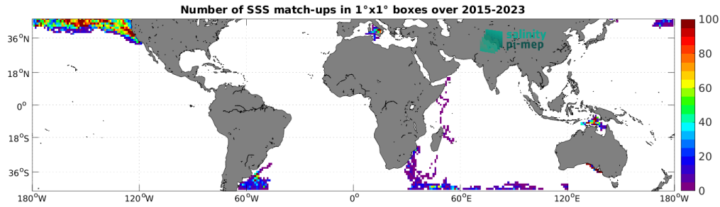
Figure 5: Number of SSS match-ups between Marine mammals SSS and the SMAP SSS L3 v6 - Monthly (RSS) SSS product for the Mid-Low Latitudes 45N-45S Pi-MEP region over 1^\circ \times 1^\circ boxes and for the full satellite product period.
