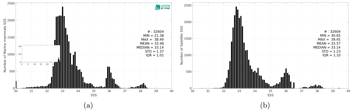
Figure 3: Histograms of SSS from Marine mammals (a) and SMAP SSS L3 v6 - Monthly (RSS) (b) considering all match-up pairs per bins of 0.1 over the Mid-Low Latitudes 45N-45S Pi-MEP region and for the full satellite product period.
