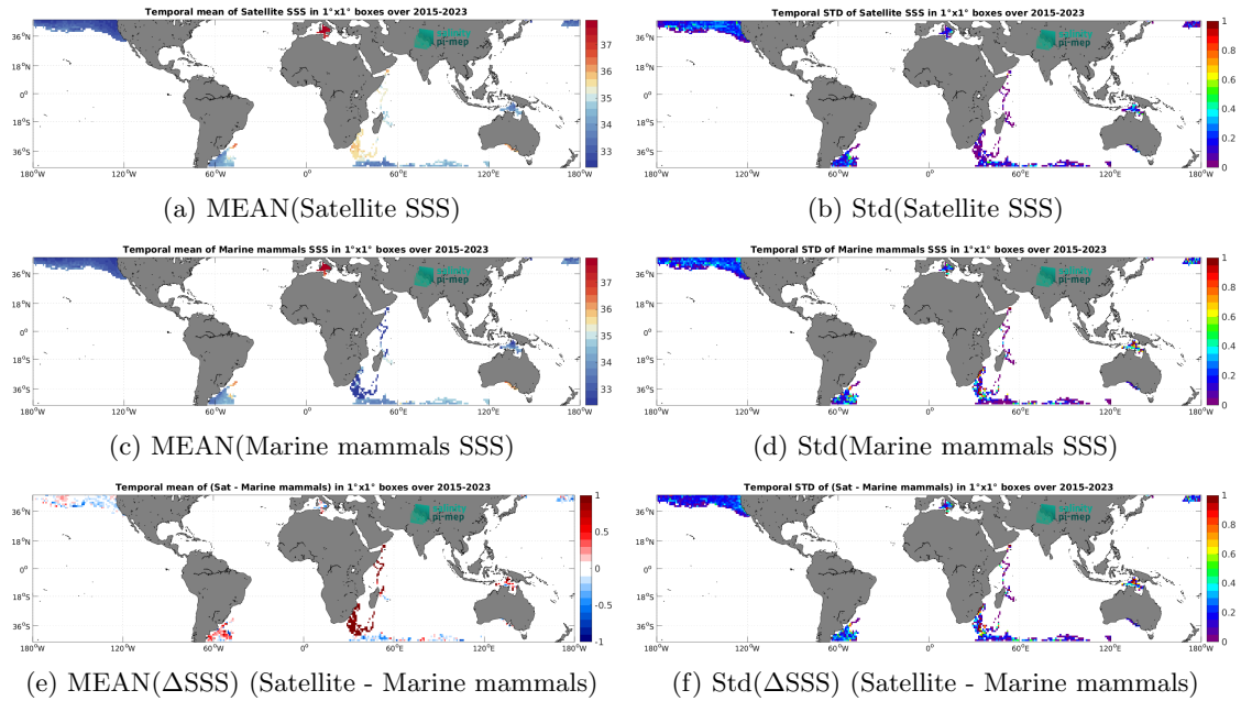
Figure 7: Temporal mean (left) and Std (right) of SSS from SMAP SSS L3 v6 - Monthly (RSS) (top), Marine mammals (middle), and of \Delta SSS (Satellite - Marine mammals). Only match-up pairs are used to generate these maps.
