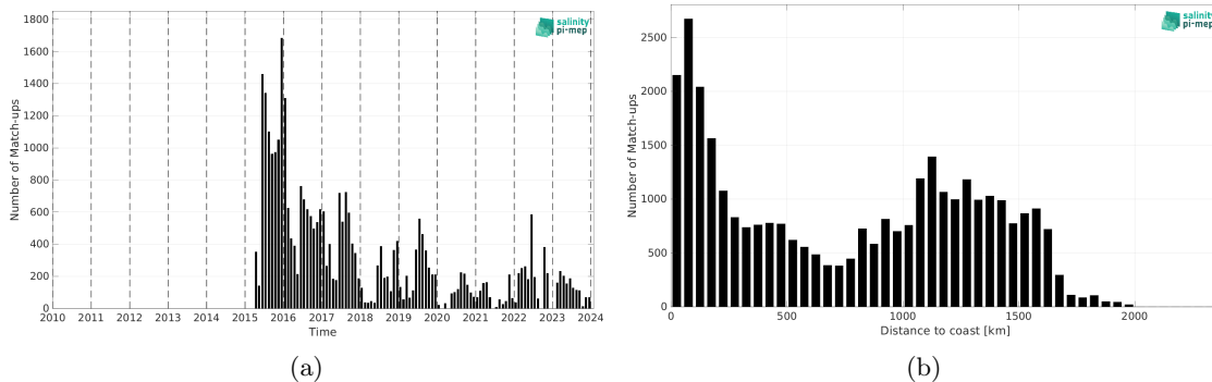
Figure 2: Number of match-ups between Marine mammals and SMAP SSS L3 v6 - Monthly (RSS) SSS as a function of time (a) and as function of the distance to coast (b) over the Mid-Low Latitudes 45N-45S Pi-MEP region and for the full satellite product period.
