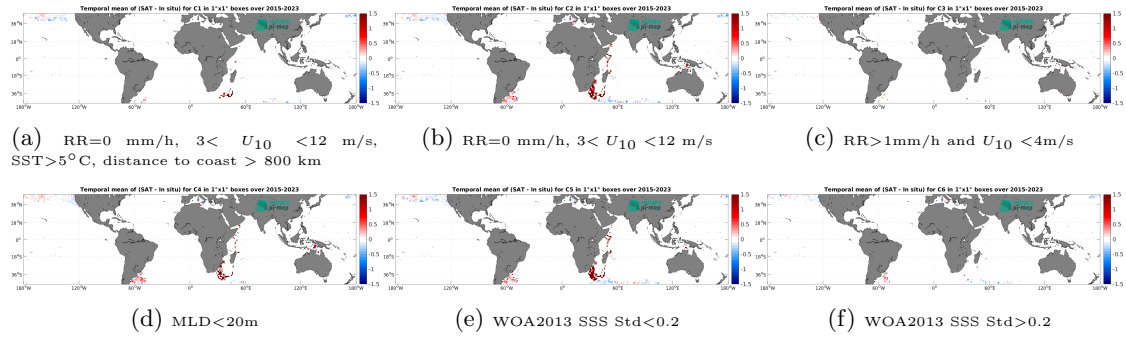
Figure 14: Temporal mean gridded over spatial boxes of size 1^\circ \times 1^\circ of \Delta SSS (SMAP SSS L3 v6 - Monthly (RSS) - Marine mammals) for 6 different subdatasets corresponding to:RR=0 mm/h, 3 < U_{10} < 12 m/s, SST>5°C, distance to coast > 800 km (a), RR=0 mm/h, 3 < U_{10} < 12 m/s (b), RR>1mm/h and U_{10} < 4 m/s (c),MLD<20m (d),WOA2013 SSS Std<0.2 (e),WOA2013 SSS Std>0.2 (f).
