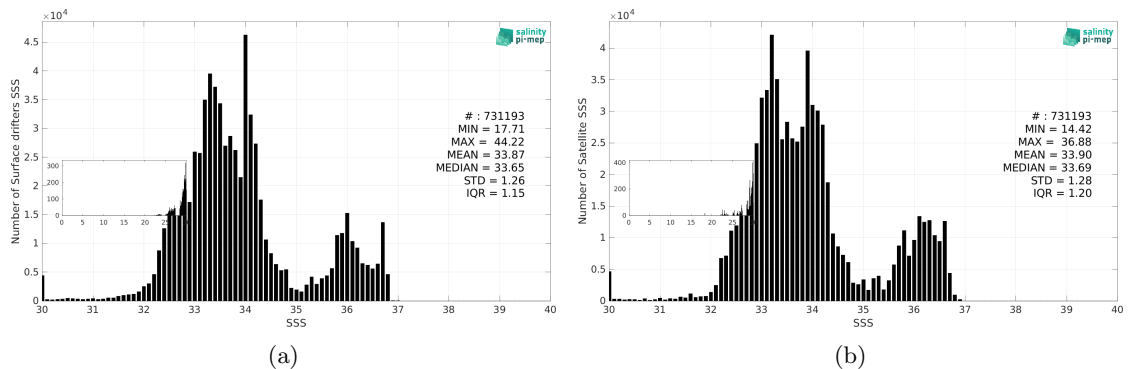
Figure 3: Histograms of SSS from Surface drifters (a) and SMAP SSS L3 v6 - Monthly (RSS) (b) considering all match-up pairs per bins of 0.1 over the Mid-Low Latitudes 45N-45S Pi-MEP region and for the full satellite product period.
