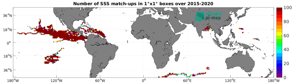
Figure 4: Number of SSS match-ups between Surface drifters SSS and the SMAP SSS L3 v6 - Monthly (RSS) SSS product for the Mid-Low Latitudes 45N-45S Pi-MEP region over 1^\circ \times 1^\circ boxes and for the full satellite product period.
