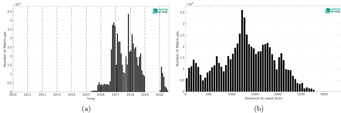
Figure 2: Number of match-ups between Surface drifters and SMAP SSS L3 v6 - Monthly (RSS) SSS as a function of time (a) and as function of the distance to coast (b) over the Mid-Low Latitudes 45N-45S Pi-MEP region and for the full satellite product period.
