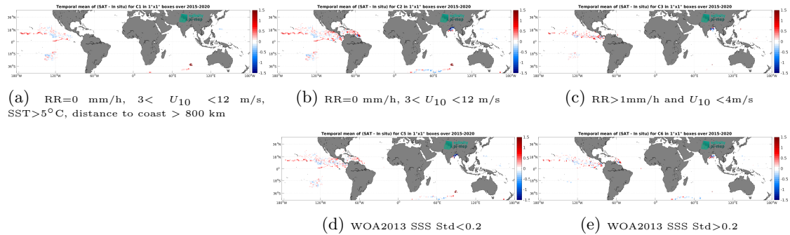
Figure 13: Temporal mean gridded over spatial boxes of size 1^\circ \times 1^\circ of \Delta SSS (SMAP SSS L3 v6 - Monthly (RSS) - Surface drifters) for 5 different subdatasets corresponding to:RR=0 mm/h, 3 < U_{10} < 12 m/s, SST >5^\circ\text{C} , distance to coast > 800 km (a), RR=0 mm/h, 3 < U_{10} < 12 m/s (b), RR >1 mm/h and U_{10} < 4 m/s (c), WOA2013 SSS Std <0.2 (d), WOA2013 SSS Std >0.2 (e).
