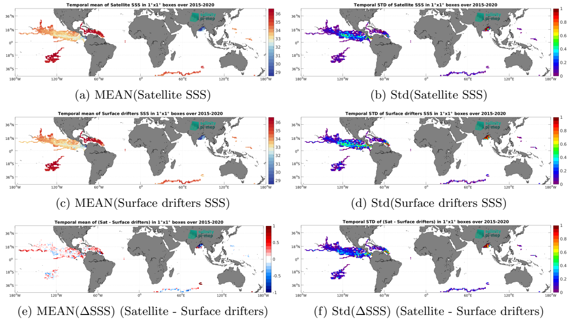
Figure 6: Temporal mean (left) and Std (right) of SSS from SMAP SSS L3 v6 - Monthly (RSS) (top), Surface drifters (middle), and of \Delta\text{SSS} (Satellite - Surface drifters). Only match-up pairs are used to generate these maps.
