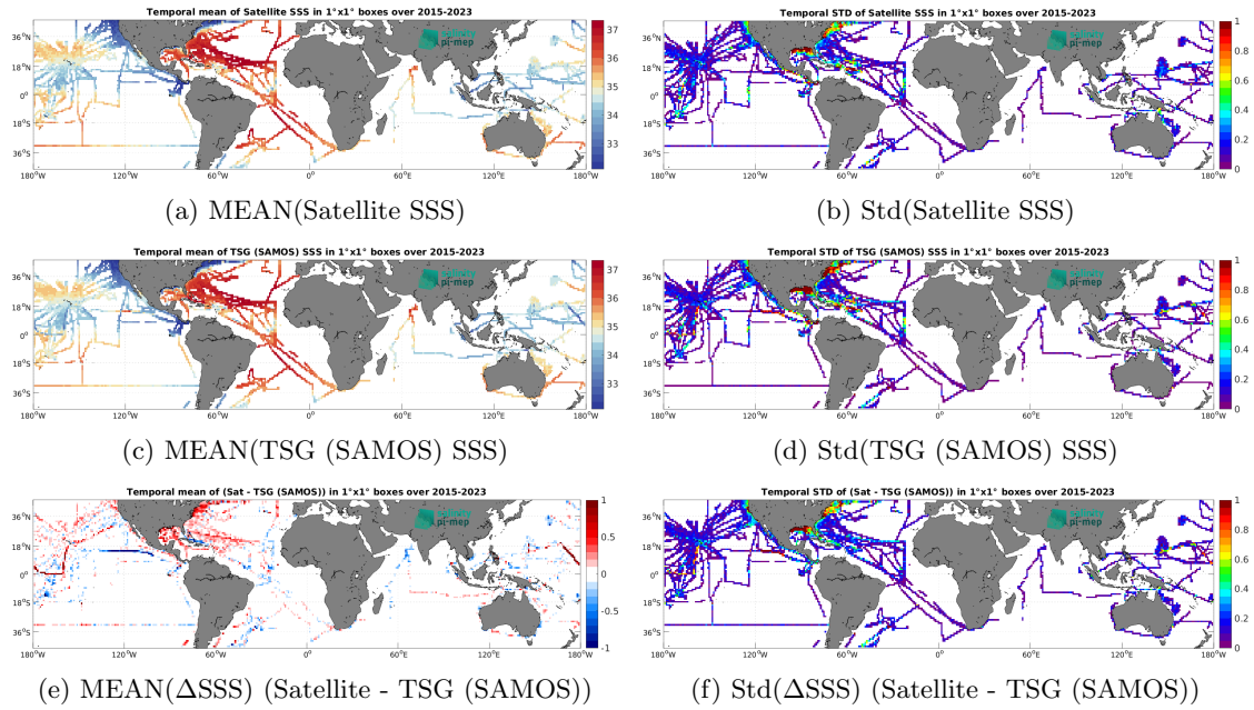
Figure 7: Temporal mean (left) and Std (right) of SSS from SMAP SSS L3 v5.3 - 8-Day running (RSS) (top), TSG (SAMOS) (middle), and of \Delta SSS (Satellite - TSG (SAMOS)). Only match-up pairs are used to generate these maps.
