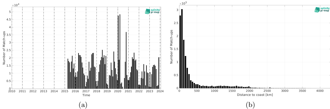
Figure 2: Number of match-ups between TSG (SAMOS) and SMAP SSS L3 v5.3 - 8-Day running (RSS) SSS as a function of time (a) and as function of the distance to coast (b) over the Mid-Low Latitudes 45N-45S Pi-MEP region and for the full satellite product period.
