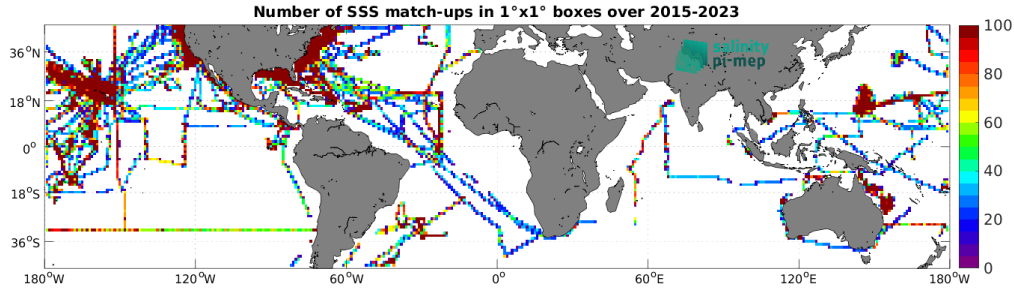
Figure 5: Number of SSS match-ups between TSG (SAMOS) SSS and the SMAP SSS L3 v5.3 - 8-Day running (RSS) SSS product for the Mid-Low Latitudes 45N-45S Pi-MEP region over 1^\circ \times 1^\circ boxes and for the full satellite product period.
