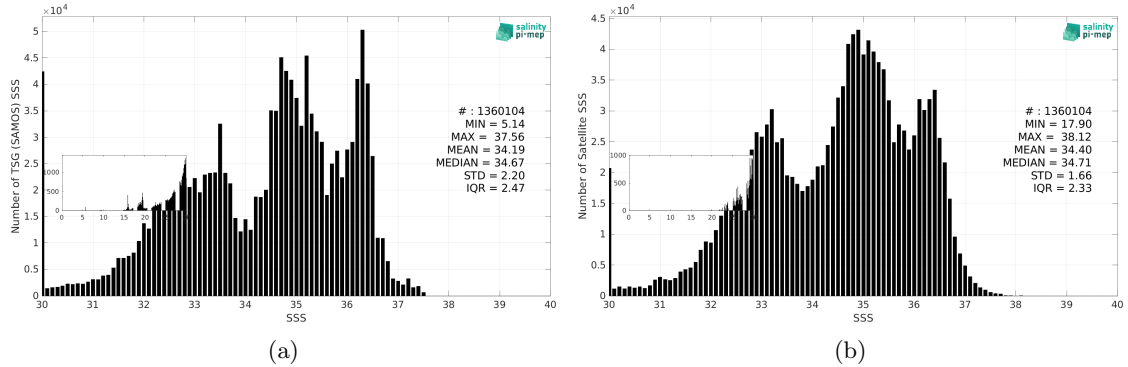
Figure 3: Histograms of SSS from TSG (SAMOS) (a) and SMAP SSS L3 v5.3 - 8-Day running (RSS) (b) considering all match-up pairs per bins of 0.1 over the Mid-Low Latitudes 45N-45S Pi-MEP region and for the full satellite product period.
