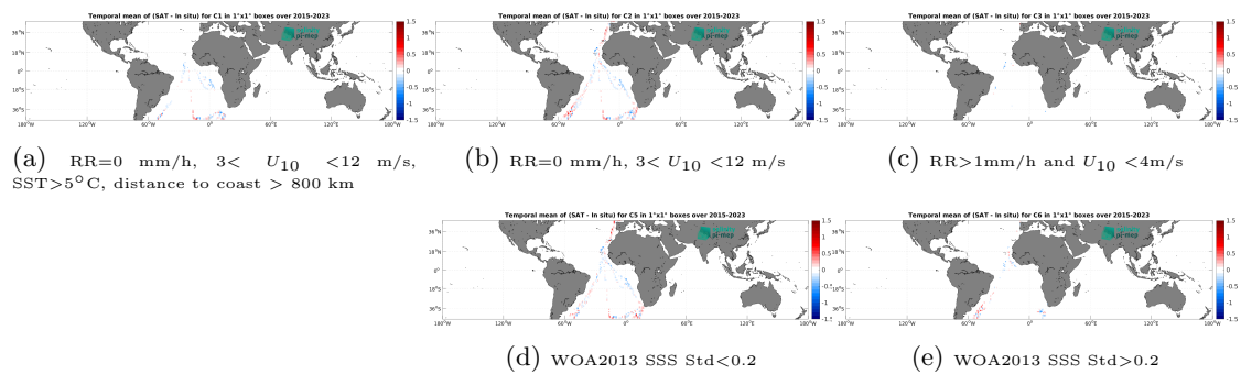
Figure 14: Temporal mean gridded over spatial boxes of size 1^\circ \times 1^\circ of \Delta SSS (SMAP SSS L3 v5.3 - 8-Day running (RSS) - TSG (Polarstern)) for 5 different subdatasets corresponding to: RR=0 mm/h, 3 < U_{10} < 12 m/s, SST > 5°C, distance to coast > 800 km (a), RR=0 mm/h, 3 < U_{10} < 12 m/s (b), RR > 1mm/h and U_{10} < 4 m/s (c), WOA2013 SSS Std < 0.2 (d), WOA2013 SSS Std > 0.2 (e).
