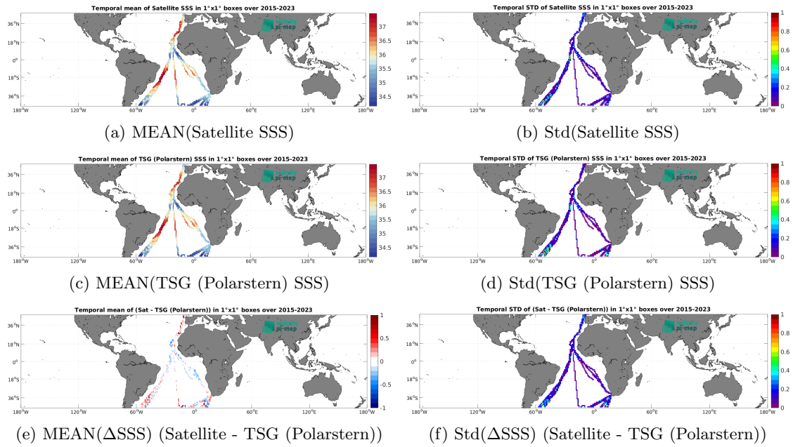
Figure 7: Temporal mean (left) and Std (right) of SSS from SMAP SSS L3 v5.3 - 8-Day running (RSS) (top), TSG (Polarstern) (middle), and of \Delta SSS (Satellite - TSG (Polarstern)). Only match-up pairs are used to generate these maps.
