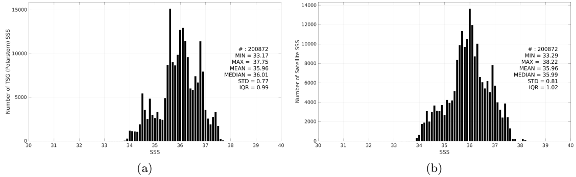
Figure 3: Histograms of SSS from TSG (Polarstern) (a) and SMAP SSS L3 v5.3 - 8-Day running (RSS) (b) considering all match-up pairs per bins of 0.1 over the Mid-Low Latitudes 45N-45S Pi-MEP region and for the full satellite product period.
