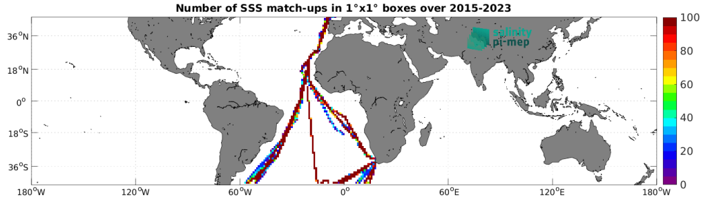
Figure 5: Number of SSS match-ups between TSG (Polarstern) SSS and the SMAP SSS L3 v5.3 - 8-Day running (RSS) SSS product for the Mid-Low Latitudes 45N-45S Pi-MEP region over 1^\circ \times 1^\circ boxes and for the full satellite product period.
