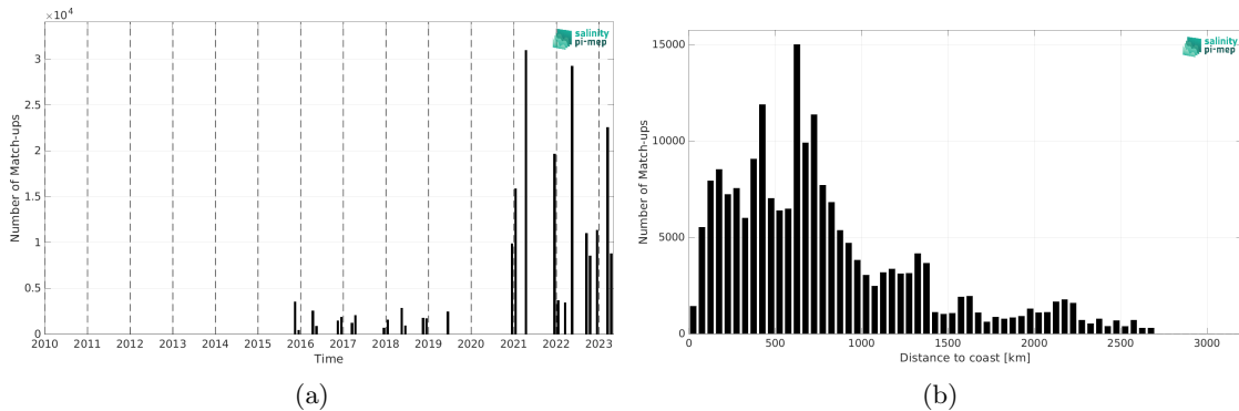
Figure 2: Number of match-ups between TSG (Polarstern) and SMAP SSS L3 v5.3 - 8-Day running (RSS) SSS as a function of time (a) and as function of the distance to coast (b) over the Mid-Low Latitudes 45N-45S Pi-MEP region and for the full satellite product period.
