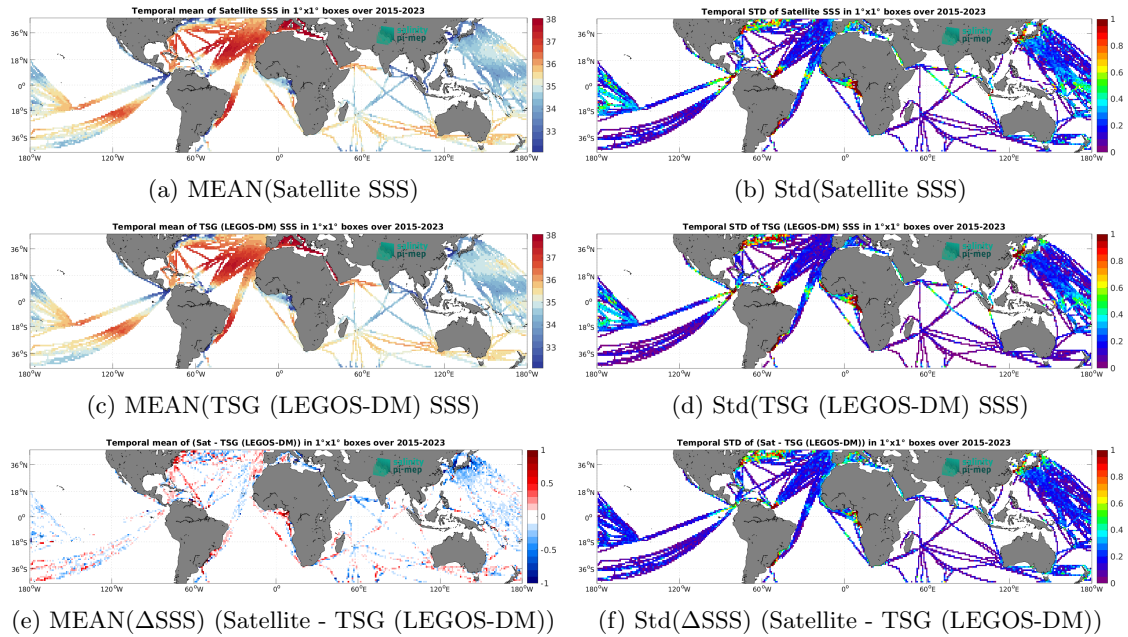
Figure 7: Temporal mean (left) and Std (right) of SSS from SMAP SSS L3 v5.3 - 8-Day running (RSS) (top), TSG (LEGOS-DM) (middle), and of \Delta SSS (Satellite - TSG (LEGOS-DM)). Only match-up pairs are used to generate these maps.
