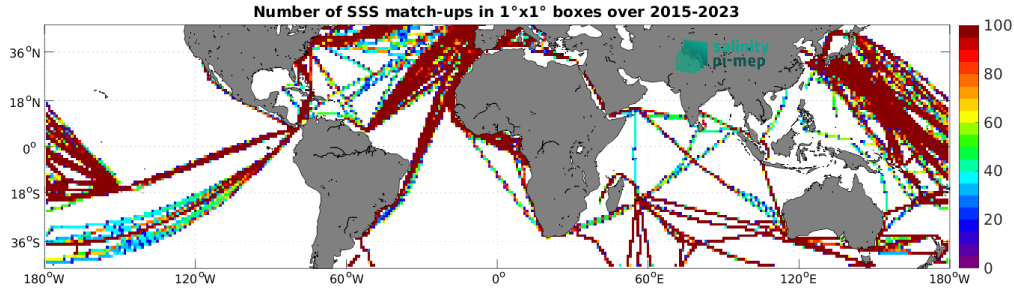
Figure 5: Number of SSS match-ups between TSG (LEGOS-DM) SSS and the SMAP SSS L3 v5.3 - 8-Day running (RSS) SSS product for the Mid-Low Latitudes 45N-45S Pi-MEP region over 1^\circ \times 1^\circ boxes and for the full satellite product period.
