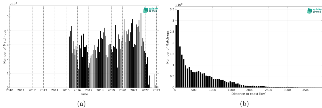
Figure 2: Number of match-ups between TSG (LEGOS-DM) and SMAP SSS L3 v5.3 - 8-Day running (RSS) SSS as a function of time (a) and as function of the distance to coast (b) over the Mid-Low Latitudes 45N-45S Pi-MEP region and for the full satellite product period.
