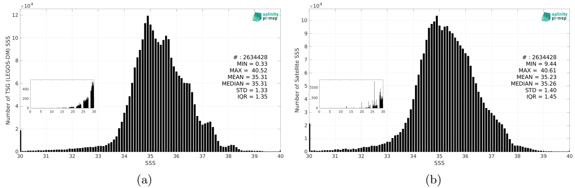
Figure 3: Histograms of SSS from TSG (LEGOS-DM) (a) and SMAP SSS L3 v5.3 - 8-Day running (RSS) (b) considering all match-up pairs per bins of 0.1 over the Mid-Low Latitudes 45N-45S Pi-MEP region and for the full satellite product period.
