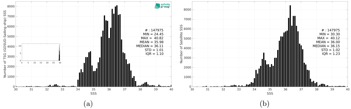
Figure 3: Histograms of SSS from TSG (GOSUD-Sailing-ship) (a) and SMAP SSS L3 v5.3 - 8-Day running (RSS) (b) considering all match-up pairs per bins of 0.1 over the Mid-Low Latitudes 45N-45S Pi-MEP region and for the full satellite product period.
