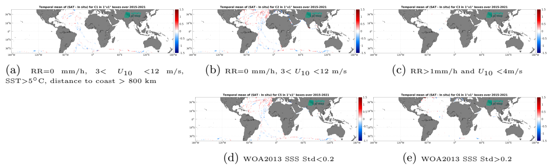
Figure 14: Temporal mean gridded over spatial boxes of size 1^\circ \times 1^\circ of \Delta\text{SSS} (SMAP SSS L3 v5.3 - 8-Day running (RSS) - TSG (GOSUD-Sailing-ship)) for 5 different subdatasets corresponding to: RR=0 mm/h, 3 < U_{10} < 12 m/s, SST > 5°C, distance to coast > 800 km (a), RR=0 mm/h, 3 < U_{10} < 12 m/s (b), RR > 1mm/h and U_{10} < 4 m/s (c), WOA2013 SSS Std < 0.2 (d), WOA2013 SSS Std > 0.2 (e).
