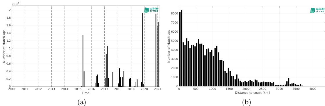
Figure 2: Number of match-ups between TSG (GOSUD-Sailing-ship) and SMAP SSS L3 v5.3 - 8-Day running (RSS) SSS as a function of time (a) and as function of the distance to coast (b) over the Mid-Low Latitudes 45N-45S Pi-MEP region and for the full satellite product period.
