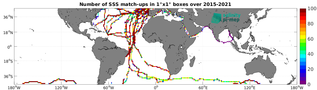
Figure 5: Number of SSS match-ups between TSG (GOSUD-Sailing-ship) SSS and the SMAP SSS L3 v5.3 - 8-Day running (RSS) SSS product for the Mid-Low Latitudes 45N-45S Pi-MEP region over 1^\circ \times 1^\circ boxes and for the full satellite product period.
