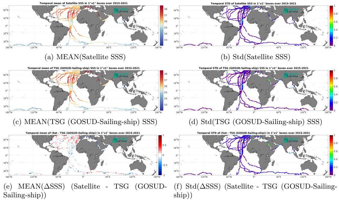
Figure 7: Temporal mean (left) and Std (right) of SSS from SMAP SSS L3 v5.3 - 8-Day running (RSS) (top), TSG (GOSUD-Sailing-ship) (middle), and of \Delta SSS (Satellite - TSG (GOSUD-Sailing-ship)). Only match-up pairs are used to generate these maps.
