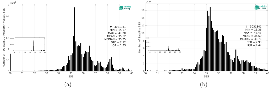
Figure 3: Histograms of SSS from TSG (GOSUD-Research-vessel) (a) and SMAP SSS L3 v5.3 - 8-Day running (RSS) (b) considering all match-up pairs per bins of 0.1 over the Mid-Low Latitudes 45N-45S Pi-MEP region and for the full satellite product period.
