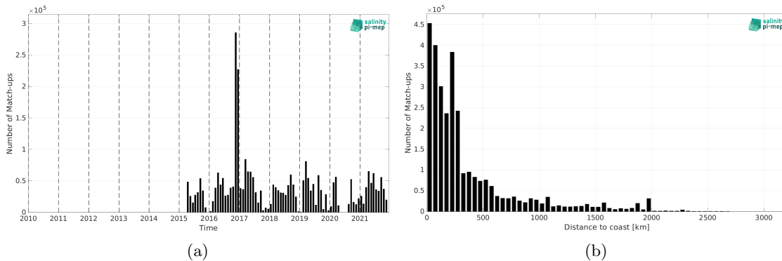
Figure 2: Number of match-ups between TSG (GOSUD-Research-vessel) and SMAP SSS L3 v5.3 - 8-Day running (RSS) SSS as a function of time (a) and as function of the distance to coast (b) over the Mid-Low Latitudes 45N-45S Pi-MEP region and for the full satellite product period.
