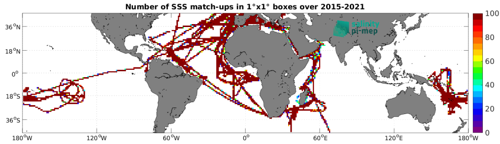
Figure 5: Number of SSS match-ups between TSG (GOSUD-Research-vessel) SSS and the SMAP SSS L3 v5.3 - 8-Day running (RSS) SSS product for the Mid-Low Latitudes 45N-45S Pi-MEP region over 1^\circ \times 1^\circ boxes and for the full satellite product period.
