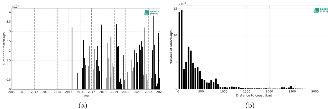
Figure 2: Number of match-ups between TSG (CSIC-UTM) and SMAP SSS L3 v5.3 - 8-Day running (RSS) SSS as a function of time (a) and as function of the distance to coast (b) over the Mid-Low Latitudes 45N-45S Pi-MEP region and for the full satellite product period.
