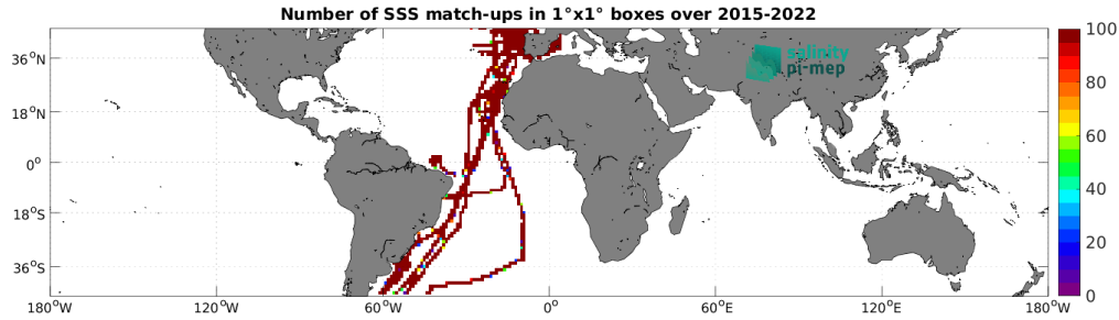
Figure 5: Number of SSS match-ups between TSG (CSIC-UTM) SSS and the SMAP SSS L3 v5.3 - 8-Day running (RSS) SSS product for the Mid-Low Latitudes 45N-45S Pi-MEP region over 1^\circ \times 1^\circ boxes and for the full satellite product period.
