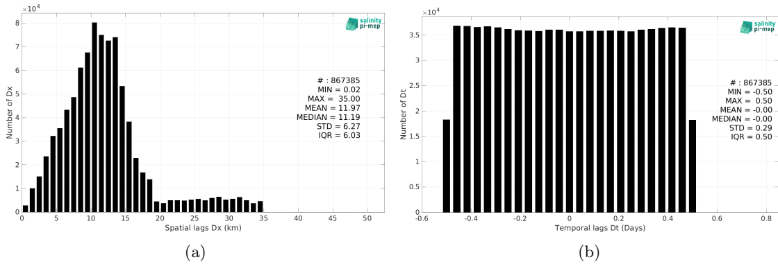
Figure 6: Histograms of the spatial (a) and temporal (b) lags between the location/time of the TSG (CSIC-UTM) measurement and the date of the corresponding SMAP SSS L3 v5.3 - 8-Day running (RSS) SSS pixel.
