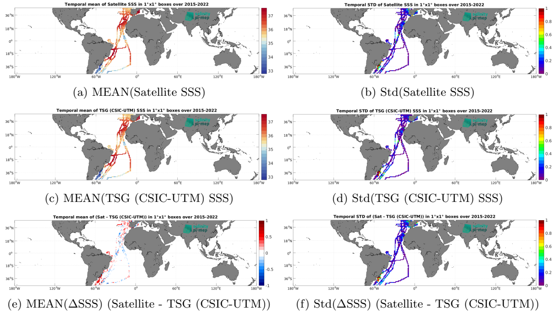
Figure 7: Temporal mean (left) and Std (right) of SSS from SMAP SSS L3 v5.3 - 8-Day running (RSS) (top), TSG (CSIC-UTM) (middle), and of \Delta SSS (Satellite - TSG (CSIC-UTM)). Only match-up pairs are used to generate these maps.
