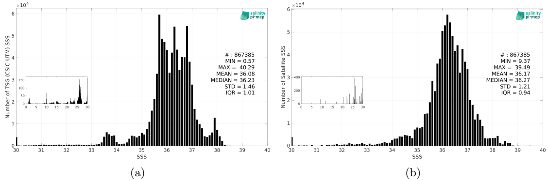
Figure 3: Histograms of SSS from TSG (CSIC-UTM) (a) and SMAP SSS L3 v5.3 - 8-Day running (RSS) (b) considering all match-up pairs per bins of 0.1 over the Mid-Low Latitudes 45N-45S Pi-MEP region and for the full satellite product period.
