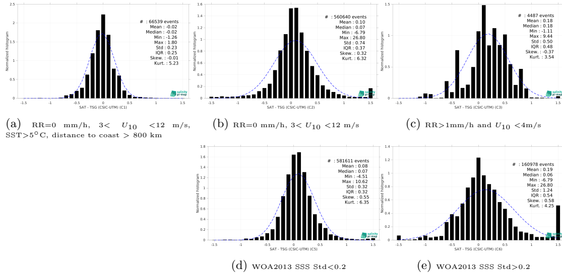
Figure 15: Normalized histogram of \Delta\text{SSS} (SMAP SSS L3 v5.3 - 8-Day running (RSS) - TSG (CSIC-UTM)) for 5 different subdatasets corresponding to: RR=0 mm/h, 3 < U_{10} < 12 m/s, SST>5°C, distance to coast > 800 km (a), RR=0 mm/h, 3 < U_{10} < 12 m/s (b), RR>1mm/h and U_{10} < 4 m/s (c), WOA2013 SSS Std<0.2 (d), WOA2013 SSS Std>0.2 (e).
