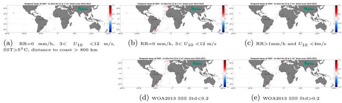
Figure 14: Temporal mean gridded over spatial boxes of size 1^\circ \times 1^\circ of \Delta SSS (SMAP SSS L3 v5.3 - 8-Day running (RSS) - TSG (CSIC-UTM)) for 5 different subdatasets corresponding to: RR=0 mm/h, 3 < U_{10} < 12 m/s, SST > 5°C, distance to coast > 800 km (a), RR=0 mm/h, 3 < U_{10} < 12 m/s (b), RR > 1mm/h and U_{10} < 4 m/s (c), WOA2013 SSS Std < 0.2 (d), WOA2013 SSS Std > 0.2 (e).
