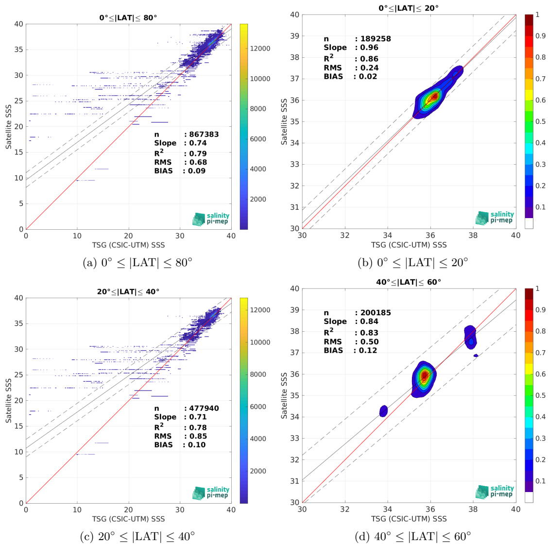
Figure 10: Contour maps of the concentration of SMAP SSS L3 v5.3 - 8-Day running (RSS) SSS (y-axis) versus TSG (CSIC-UTM) SSS (x-axis) at match-up pairs for different latitude bands. For each plot, the red line shows x=y . The black thin and dashed lines indicate a linear fit through the data cloud and the \pm 95\% confidence levels, respectively. The number match-up pairs n , the slope and R^2 coefficient of the linear fit, the root mean square (RMS) and the mean bias between satellite and in situ data are indicated for each latitude band in each plots.
