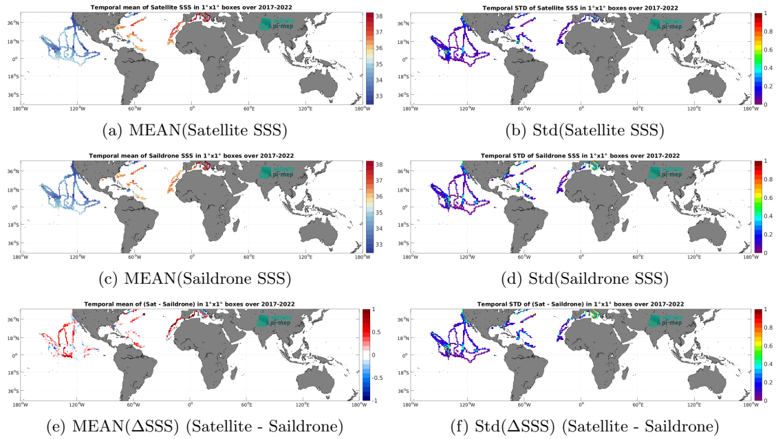
Figure 7: Temporal mean (left) and Std (right) of SSS from SMAP SSS L3 v5.3 - 8-Day running (RSS) (top), Saildrone (middle), and of \Delta SSS (Satellite - Saildrone). Only match-up pairs are used to generate these maps.
