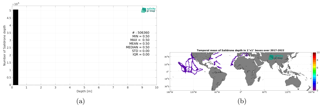
Figure 4: Histograms of the depth of the upper level SSS measurements from Sairdrone in the Match-up DataBase for the Mid-Low Latitudes 45N-45S Pi-MEP region (a) and temporal mean spatial distribution of pressure of the in situ SSS data over 1^\circ \times 1^\circ boxes and for the full satellite product period (b).
