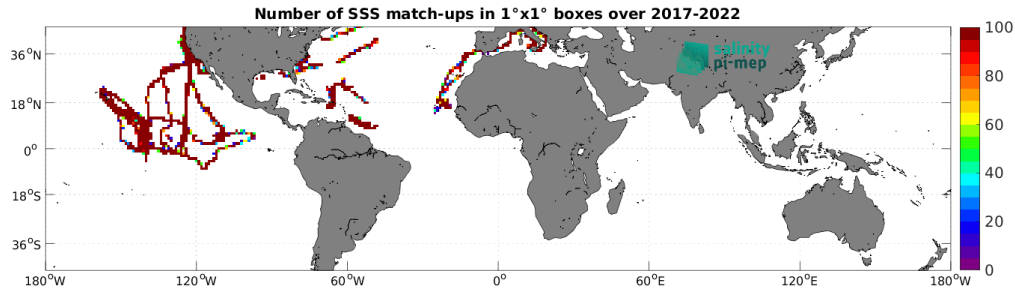
Figure 5: Number of SSS match-ups between Saildrone SSS and the SMAP SSS L3 v5.3 - 8-Day running (RSS) SSS product for the Mid-Low Latitudes 45N-45S Pi-MEP region over 1^\circ \times 1^\circ boxes and for the full satellite product period.
