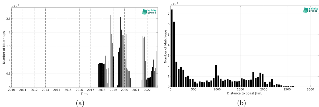
Figure 2: Number of match-ups between Saildrone and SMAP SSS L3 v5.3 - 8-Day running (RSS) SSS as a function of time (a) and as function of the distance to coast (b) over the Mid-Low Latitudes 45N-45S Pi-MEP region and for the full satellite product period.
