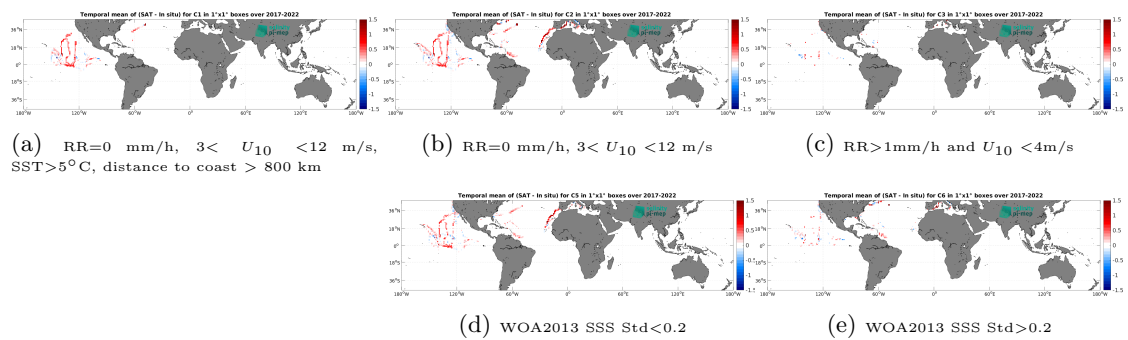
Figure 14: Temporal mean gridded over spatial boxes of size 1^\circ \times 1^\circ of \Delta\text{SSS} (SMAP SSS L3 v5.3 - 8-Day running (RSS) - Saildrone) for 5 different subdatasets corresponding to: RR=0 mm/h, 3 < U_{10} < 12 m/s, SST > 5°C, distance to coast > 800 km (a), RR=0 mm/h, 3 < U_{10} < 12 m/s (b), RR > 1mm/h and U_{10} < 4 m/s (c), WOA2013 SSS Std < 0.2 (d), WOA2013 SSS Std > 0.2 (e).
