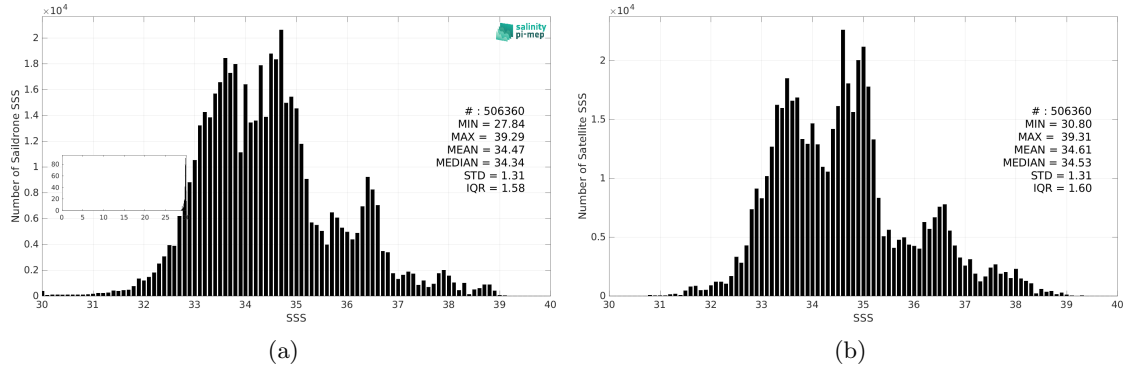
Figure 3: Histograms of SSS from Sairdrone (a) and SMAP SSS L3 v5.3 - 8-Day running (RSS) (b) considering all match-up pairs per bins of 0.1 over the Mid-Low Latitudes 45N-45S Pi-MEP region and for the full satellite product period.
