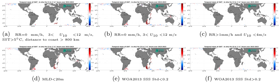
Figure 14: Temporal mean gridded over spatial boxes of size 1^\circ \times 1^\circ of \Delta SSS (SMAP SSS L3 v5.3 - 8-Day running (RSS) - Marine mammals) for 6 different subdatasets corresponding to:RR=0 mm/h, 3 < U_{10} < 12 m/s, SST > 5°C, distance to coast > 800 km (a), RR=0 mm/h, 3 < U_{10} < 12 m/s (b), RR > 1mm/h and U_{10} < 4 m/s (c),MLD < 20m (d),WOA2013 SSS Std < 0.2 (e),WOA2013 SSS Std > 0.2 (f).
