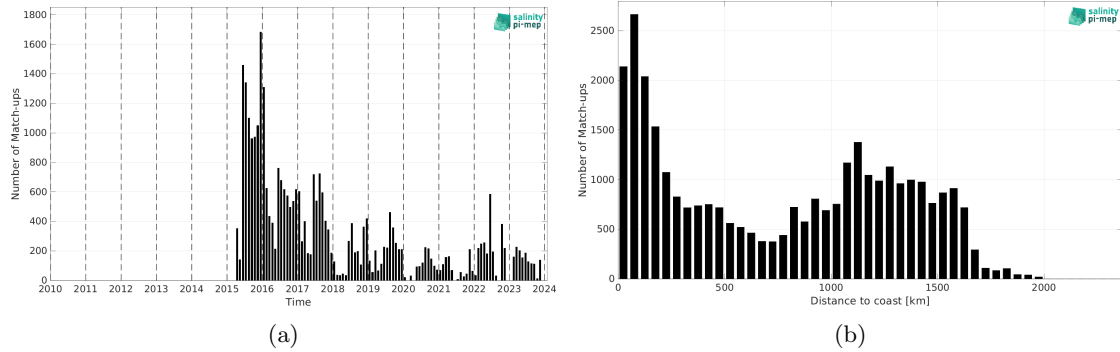
Figure 2: Number of match-ups between Marine mammals and SMAP SSS L3 v5.3 - 8-Day running (RSS) SSS as a function of time (a) and as function of the distance to coast (b) over the Mid-Low Latitudes 45N-45S Pi-MEP region and for the full satellite product period.
