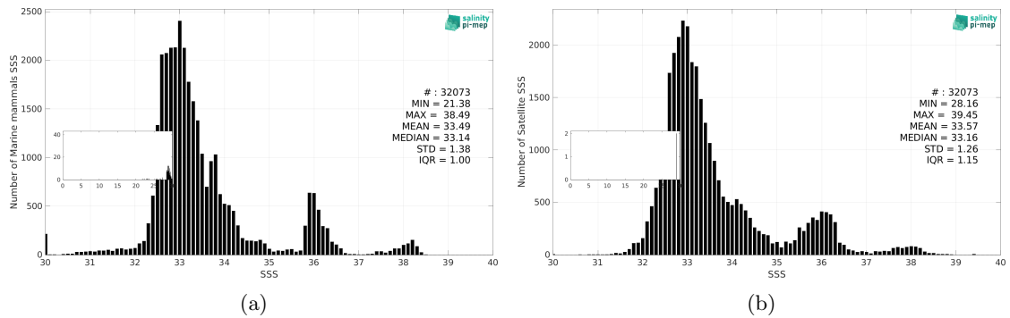
Figure 3: Histograms of SSS from Marine mammals (a) and SMAP SSS L3 v5.3 - 8-Day running (RSS) (b) considering all match-up pairs per bins of 0.1 over the Mid-Low Latitudes 45N-45S Pi-MEP region and for the full satellite product period.
