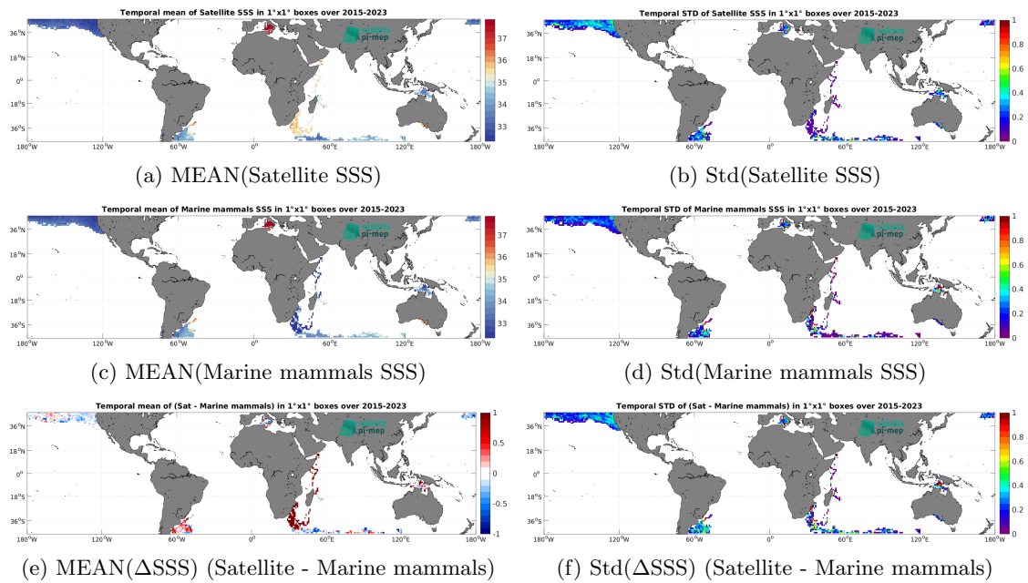
Figure 7: Temporal mean (left) and Std (right) of SSS from SMAP SSS L3 v5.3 - 8-Day running (RSS) (top), Marine mammals (middle), and of \Delta SSS (Satellite - Marine mammals). Only match-up pairs are used to generate these maps.
