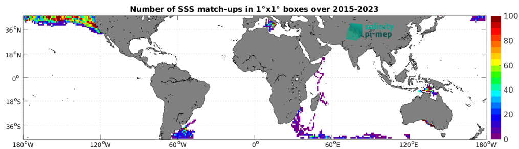
Figure 5: Number of SSS match-ups between Marine mammals SSS and the SMAP SSS L3 v5.3 - 8-Day running (RSS) SSS product for the Mid-Low Latitudes 45N-45S Pi-MEP region over 1^\circ \times 1^\circ boxes and for the full satellite product period.
