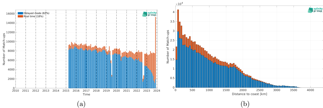
Figure 2: Number of match-ups between Argo and SMAP SSS L3 v5.3 - 8-Day running (RSS) SSS as a function of time (a) and as function of the distance to coast (b) over the Mid-Low Latitudes 45N-45S Pi-MEP region and for the full satellite product period.
