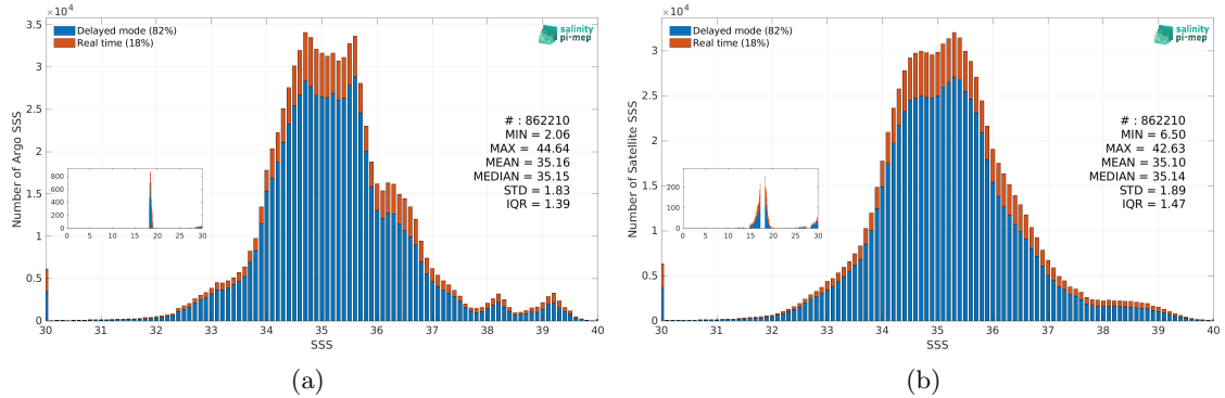
Figure 3: Histograms of SSS from Argo (a) and SMAP SSS L3 v5.3 - 8-Day running (RSS) (b) considering all match-up pairs per bins of 0.1 over the Mid-Low Latitudes 45N-45S Pi-MEP region and for the full satellite product period.
