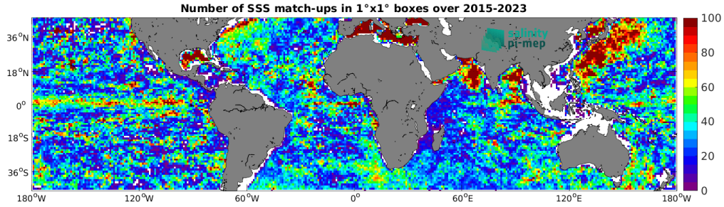
Figure 5: Number of SSS match-ups between Argo SSS and the SMAP SSS L3 v5.3 - 8-Day running (RSS) SSS product for the Mid-Low Latitudes 45N-45S Pi-MEP region over 1^\circ \times 1^\circ boxes and for the full satellite product period.
