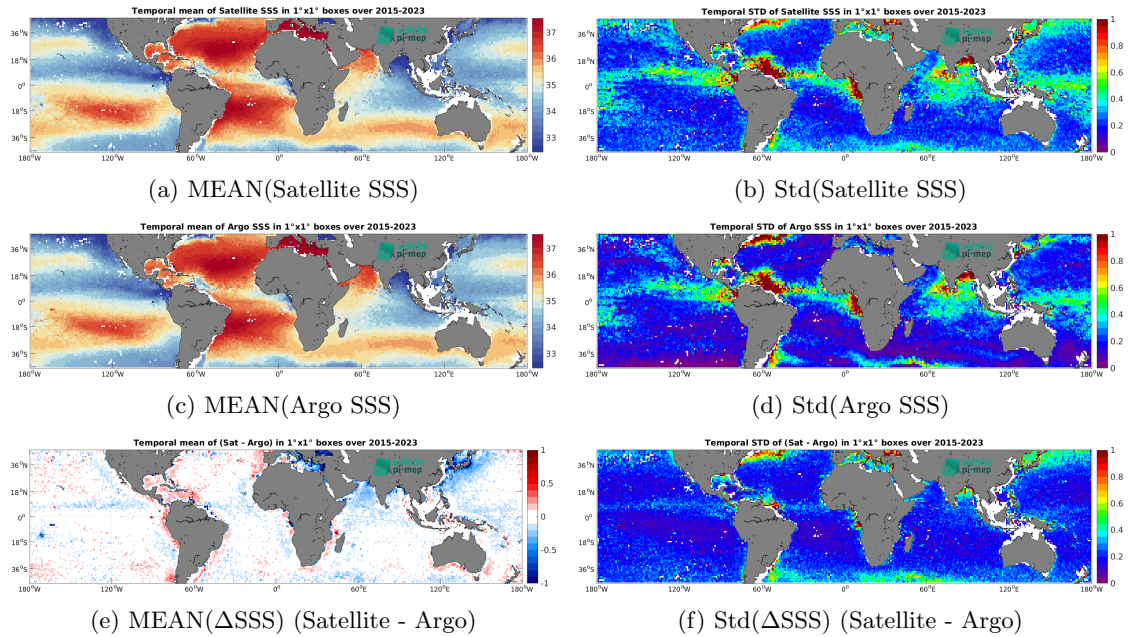
Figure 7: Temporal mean (left) and Std (right) of SSS from SMAP SSS L3 v5.3 - 8-Day running (RSS) (top), Argo (middle), and of \Delta SSS (Satellite - Argo). Only match-up pairs are used to generate these maps.
