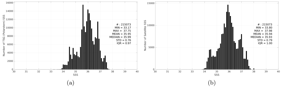
Figure 3: Histograms of SSS from TSG (Polarstern) (a) and SMAP SSS L3 v5.3 - Monthly (RSS) (b) considering all match-up pairs per bins of 0.1 over the Mid-Low Latitudes 45N-45S Pi-MEP region and for the full satellite product period.
