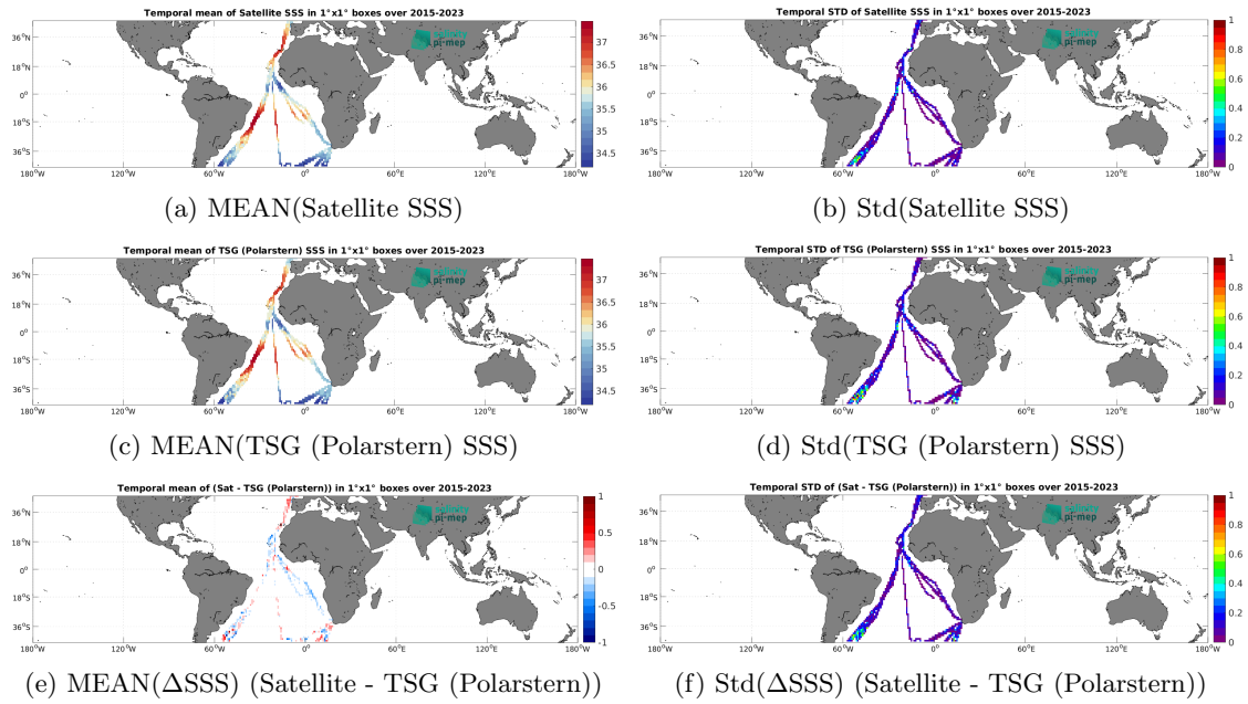
Figure 7: Temporal mean (left) and Std (right) of SSS from SMAP SSS L3 v5.3 - Monthly (RSS) (top), TSG (Polarstern) (middle), and of \Delta SSS (Satellite - TSG (Polarstern)). Only match-up pairs are used to generate these maps.
