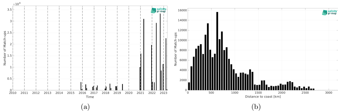
Figure 2: Number of match-ups between TSG (Polarstern) and SMAP SSS L3 v5.3 - Monthly (RSS) SSS as a function of time (a) and as function of the distance to coast (b) over the Mid-Low Latitudes 45N-45S Pi-MEP region and for the full satellite product period.
