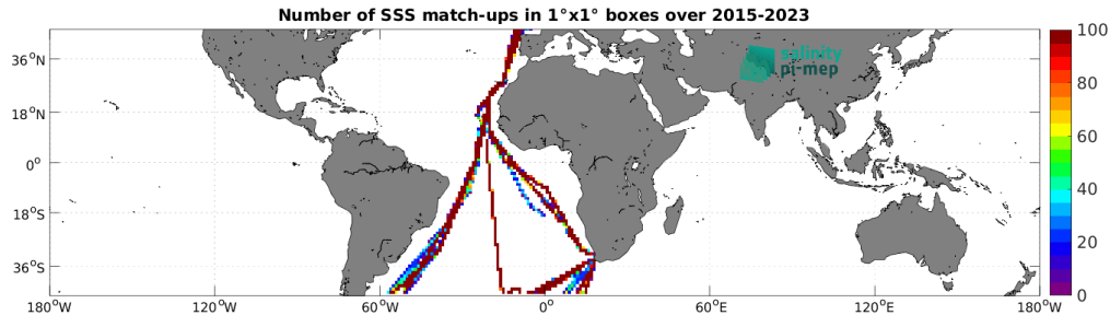
Figure 5: Number of SSS match-ups between TSG (Polarstern) SSS and the SMAP SSS L3 v5.3 - Monthly (RSS) SSS product for the Mid-Low Latitudes 45N-45S Pi-MEP region over 1^\circ \times 1^\circ boxes and for the full satellite product period.
