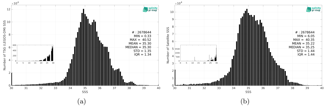
Figure 3: Histograms of SSS from TSG (LEGOS-DM) (a) and SMAP SSS L3 v5.3 - Monthly (RSS) (b) considering all match-up pairs per bins of 0.1 over the Mid-Low Latitudes 45N-45S Pi-MEP region and for the full satellite product period.
