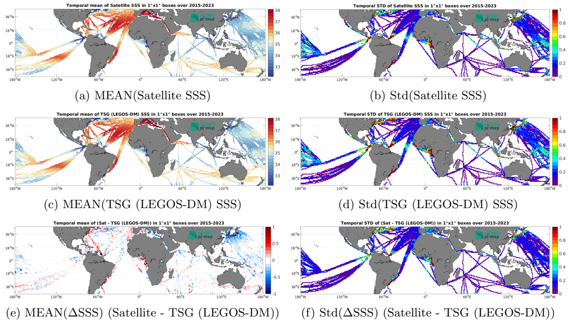
Figure 7: Temporal mean (left) and Std (right) of SSS from SMAP SSS L3 v5.3 - Monthly (RSS) (top), TSG (LEGOS-DM) (middle), and of \Delta SSS (Satellite - TSG (LEGOS-DM)). Only match-up pairs are used to generate these maps.
