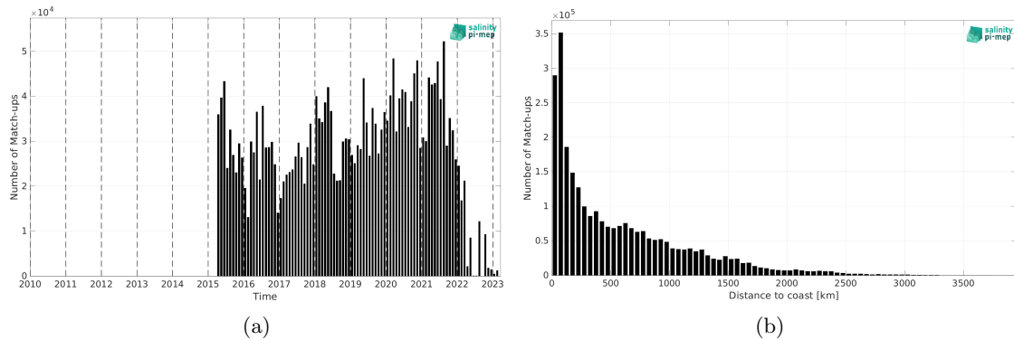
Figure 2: Number of match-ups between TSG (LEGOS-DM) and SMAP SSS L3 v5.3 - Monthly (RSS) SSS as a function of time (a) and as function of the distance to coast (b) over the Mid-Low Latitudes 45N-45S Pi-MEP region and for the full satellite product period.
