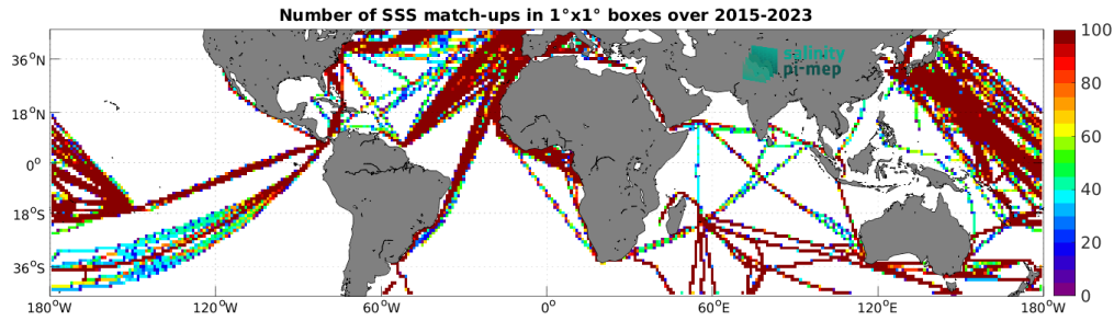
Figure 5: Number of SSS match-ups between TSG (LEGOS-DM) SSS and the SMAP SSS L3 v5.3 - Monthly (RSS) SSS product for the Mid-Low Latitudes 45N-45S Pi-MEP region over 1^\circ \times 1^\circ boxes and for the full satellite product period.
