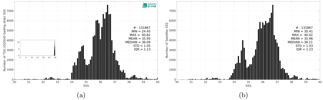
Figure 3: Histograms of SSS from TSG (GOSUD-Sailing-ship) (a) and SMAP SSS L3 v5.3 - Monthly (RSS) (b) considering all match-up pairs per bins of 0.1 over the Mid-Low Latitudes 45N-45S Pi-MEP region and for the full satellite product period.
