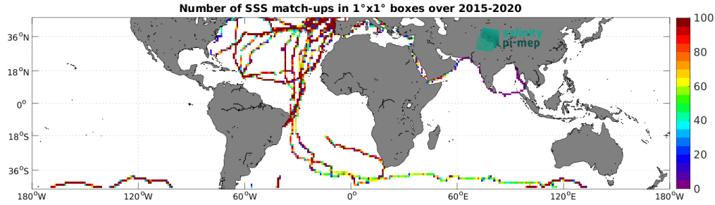
Figure 5: Number of SSS match-ups between TSG (GOSUD-Sailing-ship) SSS and the SMAP SSS L3 v5.3 - Monthly (RSS) SSS product for the Mid-Low Latitudes 45N-45S Pi-MEP region over 1^\circ \times 1^\circ boxes and for the full satellite product period.
