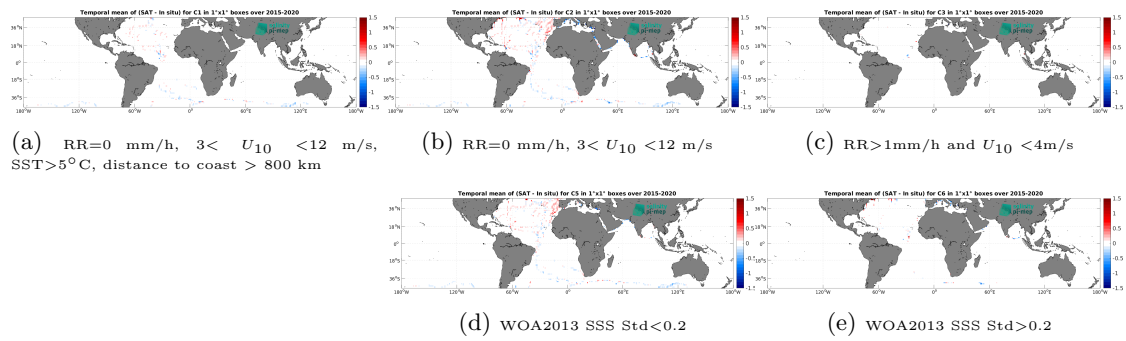
Figure 14: Temporal mean gridded over spatial boxes of size 1^\circ \times 1^\circ of \Delta\text{SSS} (SMAP SSS L3 v5.3 - Monthly (RSS) - TSG (GOSUD-Sailing-ship)) for 5 different subdatasets corresponding to: RR=0 mm/h, 3 < U_{10} < 12 m/s, SST > 5°C, distance to coast > 800 km (a), RR=0 mm/h, 3 < U_{10} < 12 m/s (b), RR > 1mm/h and U_{10} < 4 m/s (c), WOA2013 SSS Std < 0.2 (d), WOA2013 SSS Std > 0.2 (e).
