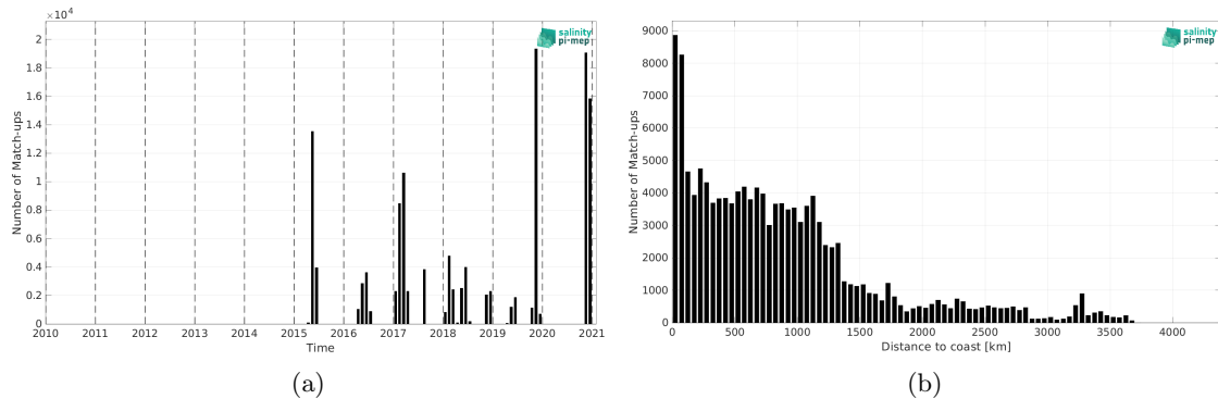
Figure 2: Number of match-ups between TSG (GOSUD-Sailing-ship) and SMAP SSS L3 v5.3 - Monthly (RSS) SSS as a function of time (a) and as function of the distance to coast (b) over the Mid-Low Latitudes 45N-45S Pi-MEP region and for the full satellite product period.
