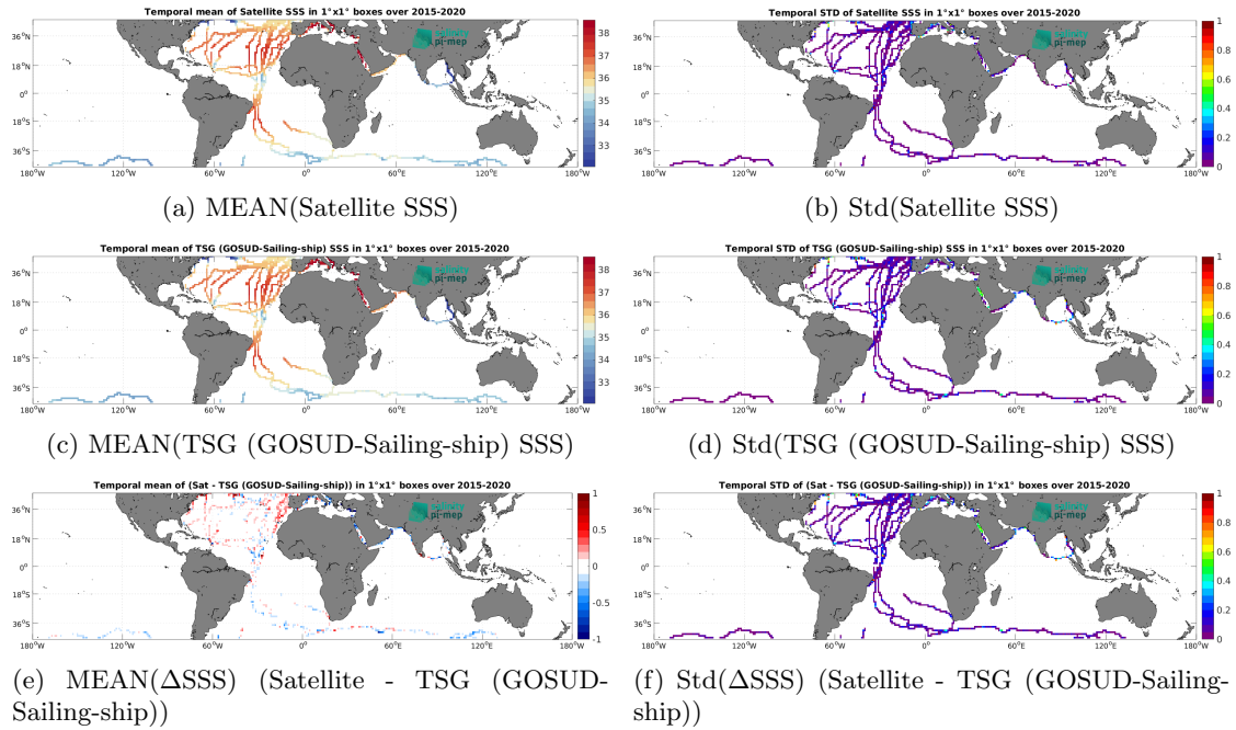
Figure 7: Temporal mean (left) and Std (right) of SSS from SMAP SSS L3 v5.3 - Monthly (RSS) (top), TSG (GOSUD-Sailing-ship) (middle), and of \Delta SSS (Satellite - TSG (GOSUD-Sailing-ship)). Only match-up pairs are used to generate these maps.
