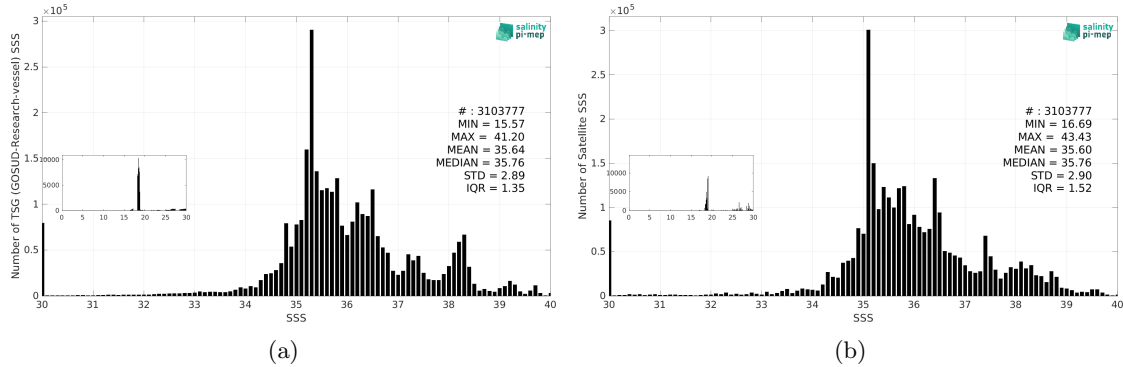
Figure 3: Histograms of SSS from TSG (GOSUD-Research-vessel) (a) and SMAP SSS L3 v5.3 - Monthly (RSS) (b) considering all match-up pairs per bins of 0.1 over the Mid-Low Latitudes 45N-45S Pi-MEP region and for the full satellite product period.
