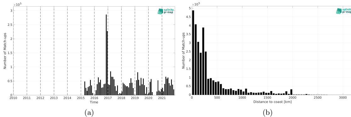
Figure 2: Number of match-ups between TSG (GOSUD-Research-vessel) and SMAP SSS L3 v5.3 - Monthly (RSS) SSS as a function of time (a) and as function of the distance to coast (b) over the Mid-Low Latitudes 45N-45S Pi-MEP region and for the full satellite product period.
