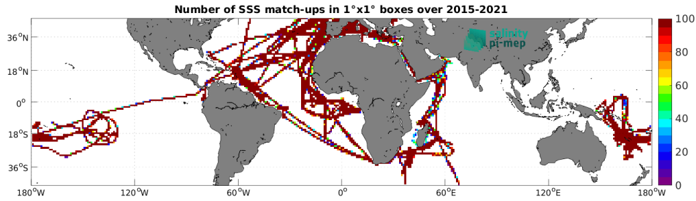
Figure 5: Number of SSS match-ups between TSG (GOSUD-Research-vessel) SSS and the SMAP SSS L3 v5.3 - Monthly (RSS) SSS product for the Mid-Low Latitudes 45N-45S Pi-MEP region over 1^\circ \times 1^\circ boxes and for the full satellite product period.
