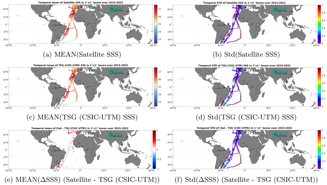
Figure 7: Temporal mean (left) and Std (right) of SSS from SMAP SSS L3 v5.3 - Monthly (RSS) (top), TSG (CSIC-UTM) (middle), and of \Delta SSS (Satellite - TSG (CSIC-UTM)). Only match-up pairs are used to generate these maps.
