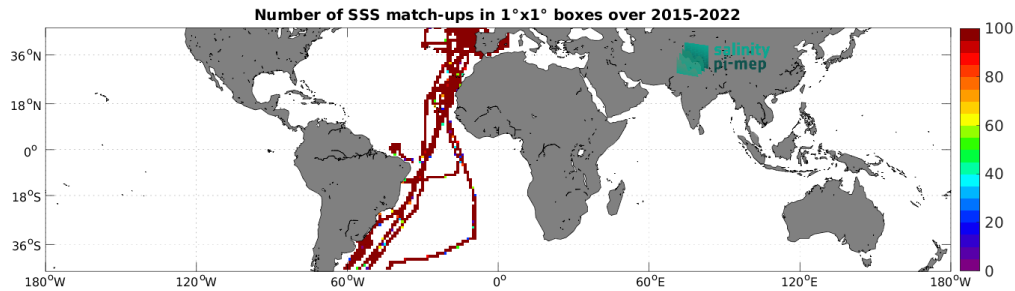
Figure 5: Number of SSS match-ups between TSG (CSIC-UTM) SSS and the SMAP SSS L3 v5.3 - Monthly (RSS) SSS product for the Mid-Low Latitudes 45N-45S Pi-MEP region over 1^\circ \times 1^\circ boxes and for the full satellite product period.
