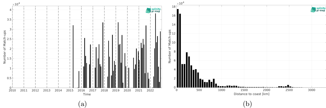
Figure 2: Number of match-ups between TSG (CSIC-UTM) and SMAP SSS L3 v5.3 - Monthly (RSS) SSS as a function of time (a) and as function of the distance to coast (b) over the Mid-Low Latitudes 45N-45S Pi-MEP region and for the full satellite product period.
