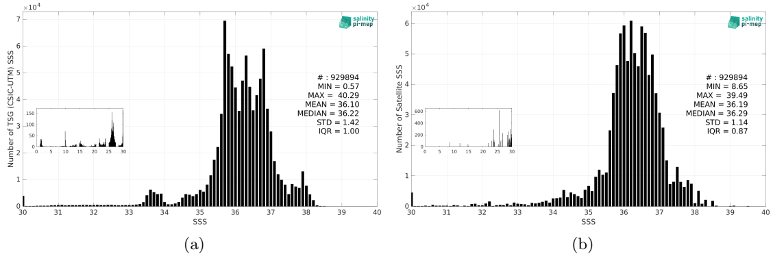
Figure 3: Histograms of SSS from TSG (CSIC-UTM) (a) and SMAP SSS L3 v5.3 - Monthly (RSS) (b) considering all match-up pairs per bins of 0.1 over the Mid-Low Latitudes 45N-45S Pi-MEP region and for the full satellite product period.
