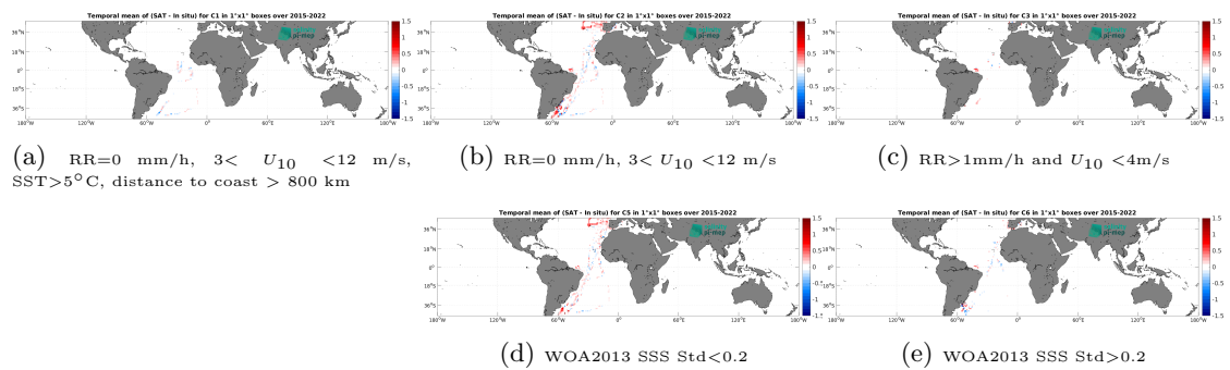
Figure 14: Temporal mean gridded over spatial boxes of size 1^\circ \times 1^\circ of \Delta SSS (SMAP SSS L3 v5.3 - Monthly (RSS) - TSG (CSIC-UTM)) for 5 different subdatasets corresponding to: RR=0 mm/h, 3 < U_{10} < 12 m/s, SST > 5°C, distance to coast > 800 km (a), RR=0 mm/h, 3 < U_{10} < 12 m/s (b), RR > 1mm/h and U_{10} < 4 m/s (c), WOA2013 SSS Std < 0.2 (d), WOA2013 SSS Std > 0.2 (e).
