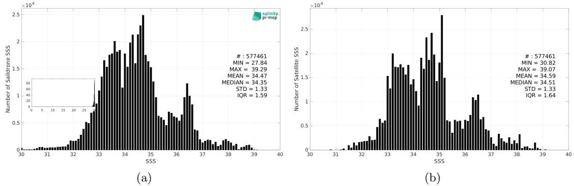
Figure 3: Histograms of SSS from Saildrone (a) and SMAP SSS L3 v5.3 - Monthly (RSS) (b) considering all match-up pairs per bins of 0.1 over the Mid-Low Latitudes 45N-45S Pi-MEP region and for the full satellite product period.
