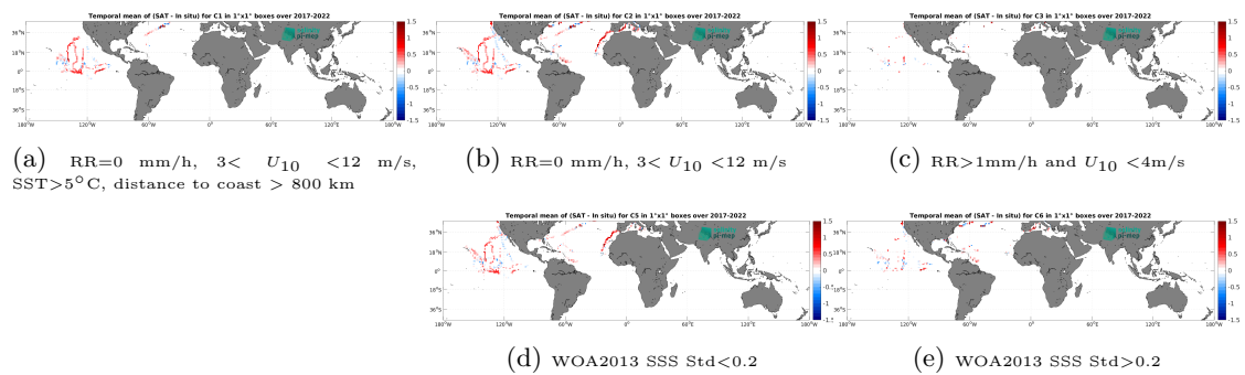
Figure 14: Temporal mean gridded over spatial boxes of size 1^\circ \times 1^\circ of \Delta\text{SSS} (SMAP SSS L3 v5.3 - Monthly (RSS) - Sairdrone) for 5 different subdatasets corresponding to:RR=0 mm/h, 3 < U_{10} < 12 m/s, SST > 5^\circ\text{C} , distance to coast > 800 km (a), RR=0 mm/h, 3 < U_{10} < 12 m/s (b), RR > 1 mm/h and U_{10} < 4 m/s (c), WOA2013 SSS Std < 0.2 (d), WOA2013 SSS Std > 0.2 (e).
