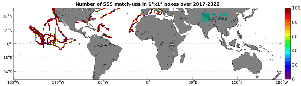
Figure 5: Number of SSS match-ups between Saildrone SSS and the SMAP SSS L3 v5.3 - Monthly (RSS) SSS product for the Mid-Low Latitudes 45N-45S Pi-MEP region over 1^\circ \times 1^\circ boxes and for the full satellite product period.
