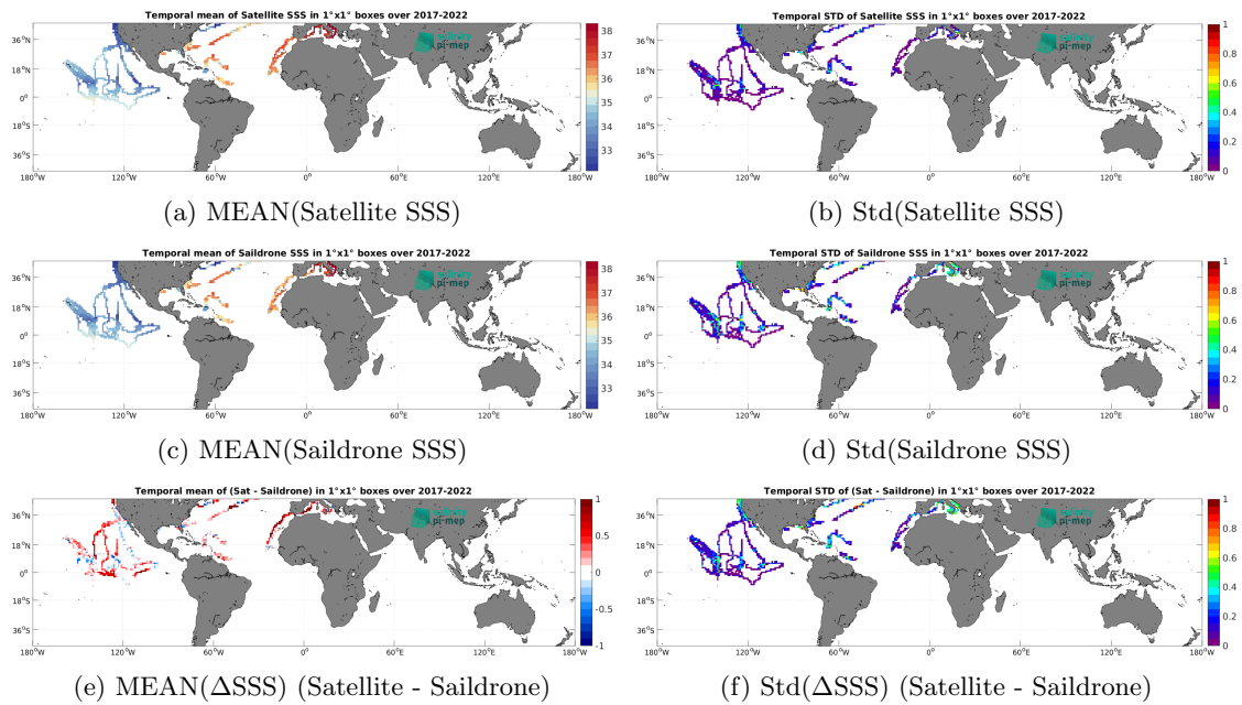
Figure 7: Temporal mean (left) and Std (right) of SSS from SMAP SSS L3 v5.3 - Monthly (RSS) (top), Saildrone (middle), and of \Delta SSS (Satellite - Saildrone). Only match-up pairs are used to generate these maps.
