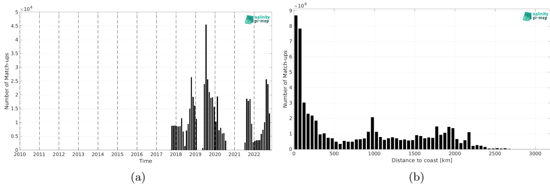
Figure 2: Number of match-ups between Saildrone and SMAP SSS L3 v5.3 - Monthly (RSS) SSS as a function of time (a) and as function of the distance to coast (b) over the Mid-Low Latitudes 45N-45S Pi-MEP region and for the full satellite product period.
