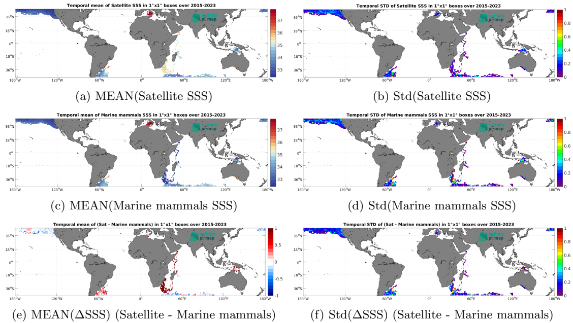
Figure 7: Temporal mean (left) and Std (right) of SSS from SMAP SSS L3 v5.3 - Monthly (RSS) (top), Marine mammals (middle), and of \Delta SSS (Satellite - Marine mammals). Only match-up pairs are used to generate these maps.
