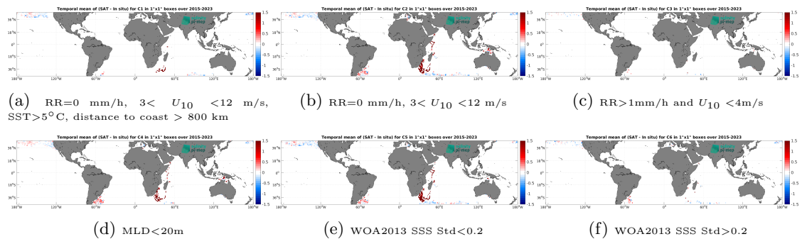
Figure 14: Temporal mean gridded over spatial boxes of size 1^\circ \times 1^\circ of \Delta SSS (SMAP SSS L3 v5.3 - Monthly (RSS) - Marine mammals) for 6 different subdatasets corresponding to:RR=0 mm/h, 3 < U_{10} < 12 m/s, SST >5^\circ C, distance to coast > 800 km (a), RR=0 mm/h, 3 < U_{10} < 12 m/s (b), RR >1 mm/h and U_{10} < 4 m/s (c),MLD <20 m (d),WOA2013 SSS Std <0.2 (e),WOA2013 SSS Std >0.2 (f).
