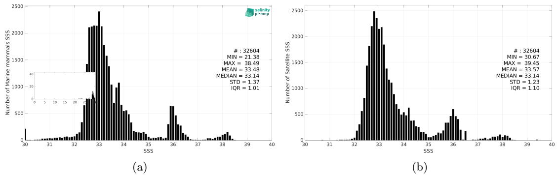
Figure 3: Histograms of SSS from Marine mammals (a) and SMAP SSS L3 v5.3 - Monthly (RSS) (b) considering all match-up pairs per bins of 0.1 over the Mid-Low Latitudes 45N-45S Pi-MEP region and for the full satellite product period.
