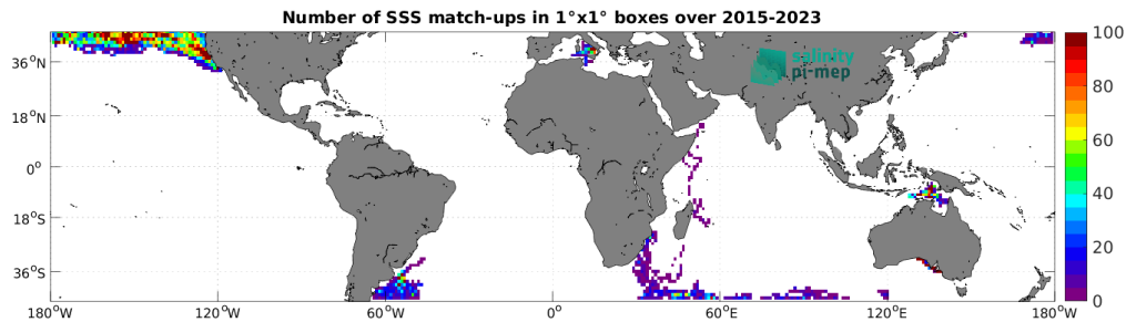
Figure 5: Number of SSS match-ups between Marine mammals SSS and the SMAP SSS L3 v5.3 - Monthly (RSS) SSS product for the Mid-Low Latitudes 45N-45S Pi-MEP region over 1^\circ \times 1^\circ boxes and for the full satellite product period.
