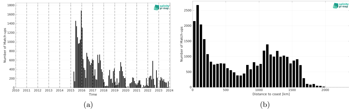
Figure 2: Number of match-ups between Marine mammals and SMAP SSS L3 v5.3 - Monthly (RSS) SSS as a function of time (a) and as function of the distance to coast (b) over the Mid-Low Latitudes 45N-45S Pi-MEP region and for the full satellite product period.
