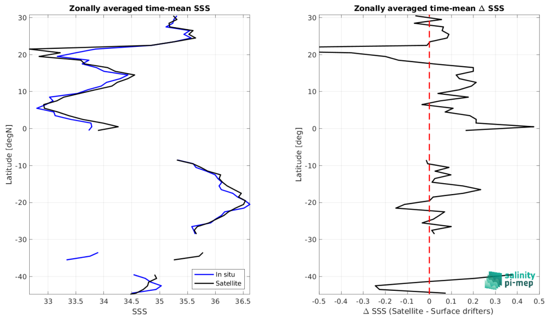
Figure 8: Left panel: Zonal mean SSS from SMAP SSS L3 v5.3 - Monthly (RSS) satellite product (black) and from Surface drifters (blue). Right panel: Zonal mean of \Delta SSS (Satellite - Surface drifters) for all the collected Pi-MEP match-up pairs estimated over the full satellite product period.
