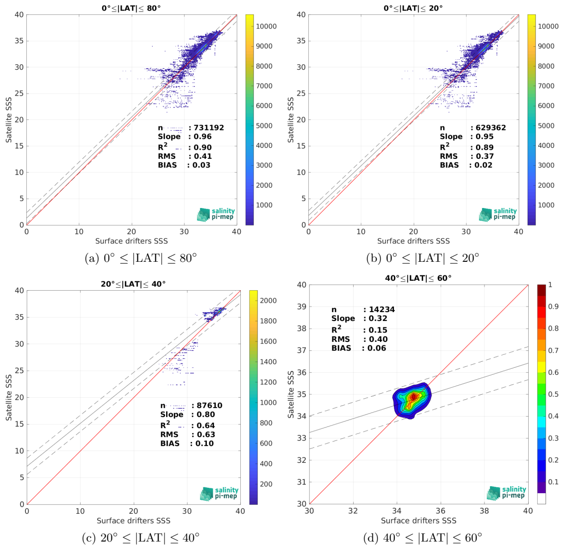
Figure 9: Contour maps of the concentration of SMAP SSS L3 v5.3 - Monthly (RSS) SSS (y-axis) versus Surface drifters SSS (x-axis) at match-up pairs for different latitude bands. For each plot, the red line shows x=y . The black thin and dashed lines indicate a linear fit through the data cloud and the \pm 95\% confidence levels, respectively. The number match-up pairs n , the slope and R^2 coefficient of the linear fit, the root mean square (RMS) and the mean bias between satellite and in situ data are indicated for each latitude band in each plot.
