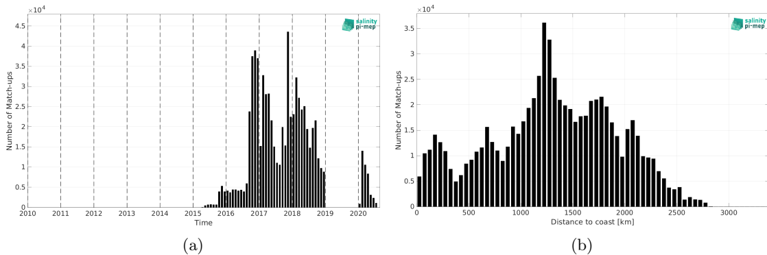
Figure 2: Number of match-ups between Surface drifters and SMAP SSS L3 v5.3 - Monthly (RSS) SSS as a function of time (a) and as function of the distance to coast (b) over the Mid-Low Latitudes 45N-45S Pi-MEP region and for the full satellite product period.
