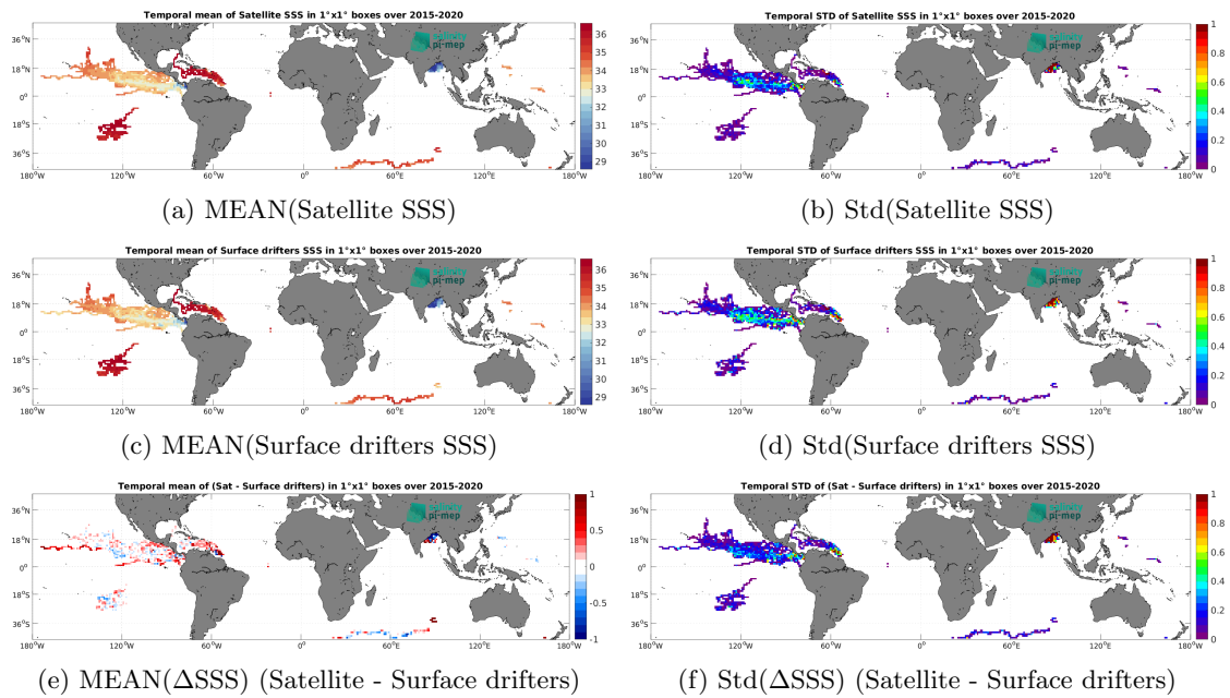
Figure 6: Temporal mean (left) and Std (right) of SSS from SMAP SSS L3 v5.3 - Monthly (RSS) (top), Surface drifters (middle), and of \Delta SSS (Satellite - Surface drifters). Only match-up pairs are used to generate these maps.
