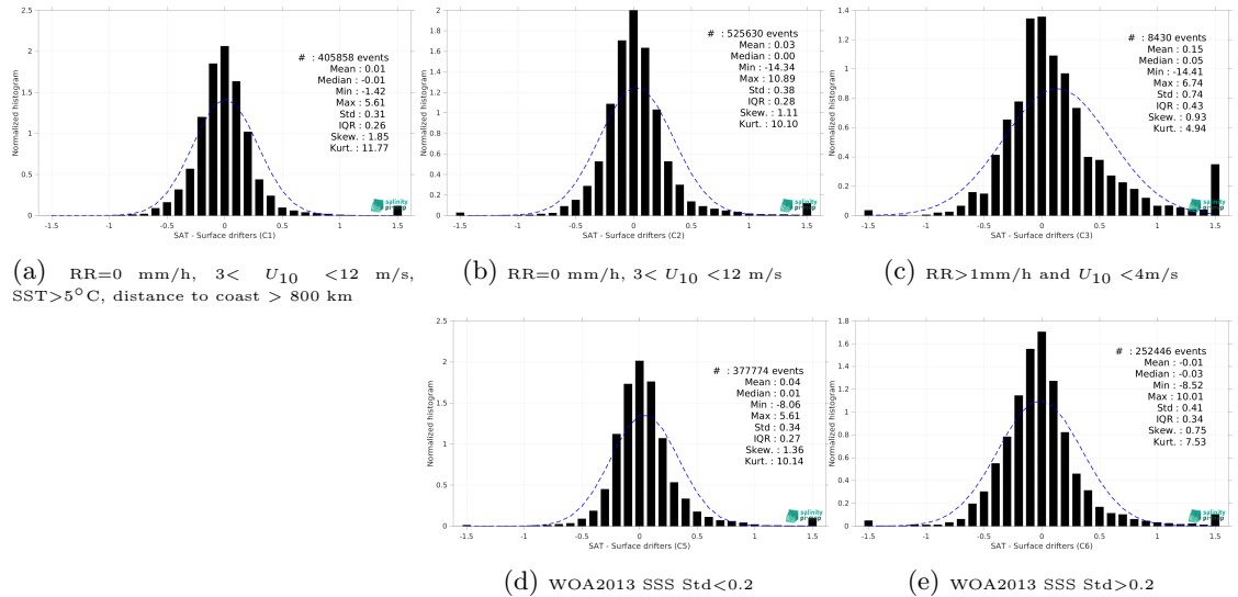
Figure 14: Normalized histogram of \Delta SSS (SMAP SSS L3 v5.3 - Monthly (RSS) - Surface drifters) for 5 different subdatasets corresponding to: RR=0 mm/h, 3 < U_{10} < 12 m/s, SST >5^\circ C, distance to coast > 800 km (a), RR=0 mm/h, 3 < U_{10} < 12 m/s (b), RR >1 mm/h and U_{10} < 4 m/s (c), WOA2013 SSS Std <0.2 (d), WOA2013 SSS Std >0.2 (e).
