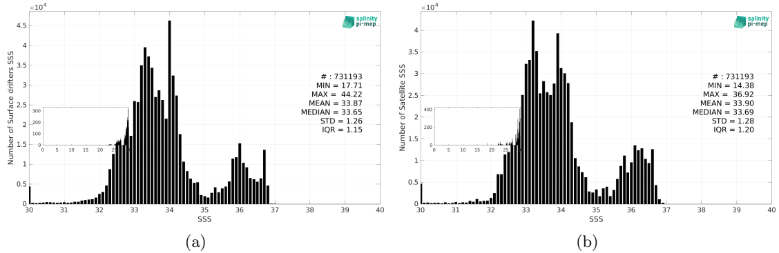
Figure 3: Histograms of SSS from Surface drifters (a) and SMAP SSS L3 v5.3 - Monthly (RSS) (b) considering all match-up pairs per bins of 0.1 over the Mid-Low Latitudes 45N-45S Pi-MEP region and for the full satellite product period.
