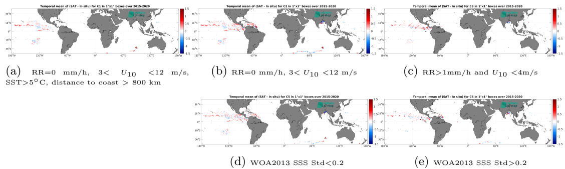
Figure 13: Temporal mean gridded over spatial boxes of size 1^\circ \times 1^\circ of \Delta SSS (SMAP SSS L3 v5.3 - Monthly (RSS) - Surface drifters) for 5 different subdatasets corresponding to:RR=0 mm/h, 3 < U_{10} < 12 m/s, SST >5^\circ C, distance to coast > 800 km (a), RR=0 mm/h, 3 < U_{10} < 12 m/s (b), RR >1 mm/h and U_{10} < 4 m/s (c), WOA2013 SSS Std <0.2 (d), WOA2013 SSS Std >0.2 (e).
