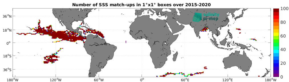
Figure 4: Number of SSS match-ups between Surface drifters SSS and the SMAP SSS L3 v5.3 - Monthly (RSS) SSS product for the Mid-Low Latitudes 45N-45S Pi-MEP region over 1^\circ \times 1^\circ boxes and for the full satellite product period.
