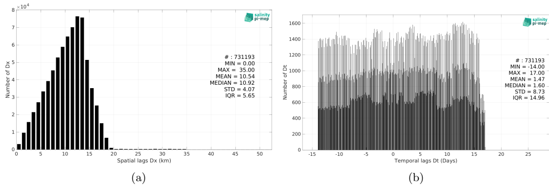
Figure 5: Histograms of the spatial (a) and temporal (b) lags between the location/time of the Surface drifters measurement and the date of the corresponding SMAP SSS L3 v5.3 - Monthly (RSS) SSS pixel.
