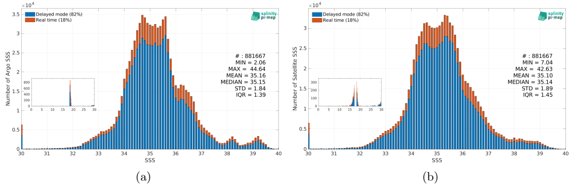
Figure 3: Histograms of SSS from Argo (a) and SMAP SSS L3 v5.3 - Monthly (RSS) (b) considering all match-up pairs per bins of 0.1 over the Mid-Low Latitudes 45N-45S Pi-MEP region and for the full satellite product period.
