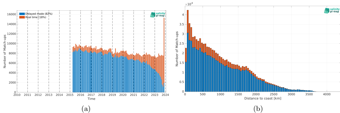
Figure 2: Number of match-ups between Argo and SMAP SSS L3 v5.3 - Monthly (RSS) SSS as a function of time (a) and as function of the distance to coast (b) over the Mid-Low Latitudes 45N-45S Pi-MEP region and for the full satellite product period.
