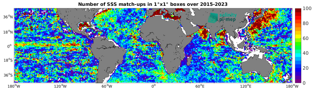
Figure 5: Number of SSS match-ups between Argo SSS and the SMAP SSS L3 v5.3 - Monthly (RSS) SSS product for the Mid-Low Latitudes 45N-45S Pi-MEP region over 1^\circ \times 1^\circ boxes and for the full satellite product period.
