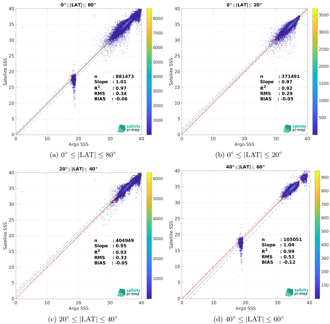
Figure 10: Contour maps of the concentration of SMAP SSS L3 v5.3 - Monthly (RSS) SSS (y-axis) versus Argo SSS (x-axis) at match-up pairs for different latitude bands. For each plot, the red line shows x=y . The black thin and dashed lines indicate a linear fit through the data cloud and the \pm 95\% confidence levels, respectively. The number match-up pairs n , the slope and R^2 coefficient of the linear fit, the root mean square (RMS) and the mean bias between satellite and in situ data are indicated for each latitude band in each plots.
