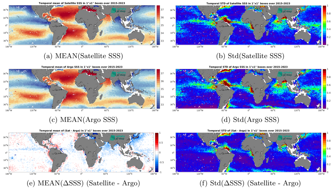
Figure 7: Temporal mean (left) and Std (right) of SSS from SMAP SSS L3 v5.3 - Monthly (RSS) (top), Argo (middle), and of \Delta SSS (Satellite - Argo). Only match-up pairs are used to generate these maps.
