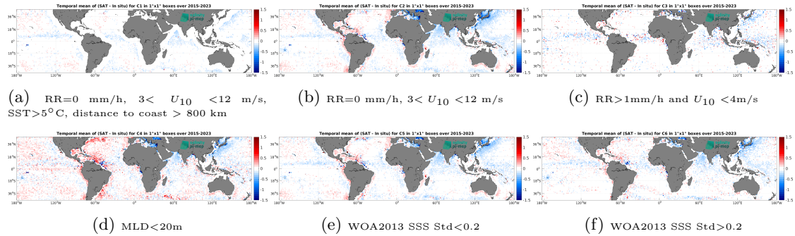
Figure 14: Temporal mean gridded over spatial boxes of size 1^\circ \times 1^\circ of \Delta\text{SSS} (SMAP SSS L3 v5.3 - Monthly (RSS) - Argo) for 6 different subdatasets corresponding to:RR=0 mm/h, 3 < U_{10} < 12 m/s, SST>5°C, distance to coast > 800 km (a), RR=0 mm/h, 3 < U_{10} < 12 m/s (b), RR>1mm/h and U_{10} < 4 m/s (c),MLD<20m (d),WOA2013 SSS Std<0.2 (e),WOA2013 SSS Std>0.2 (f).
