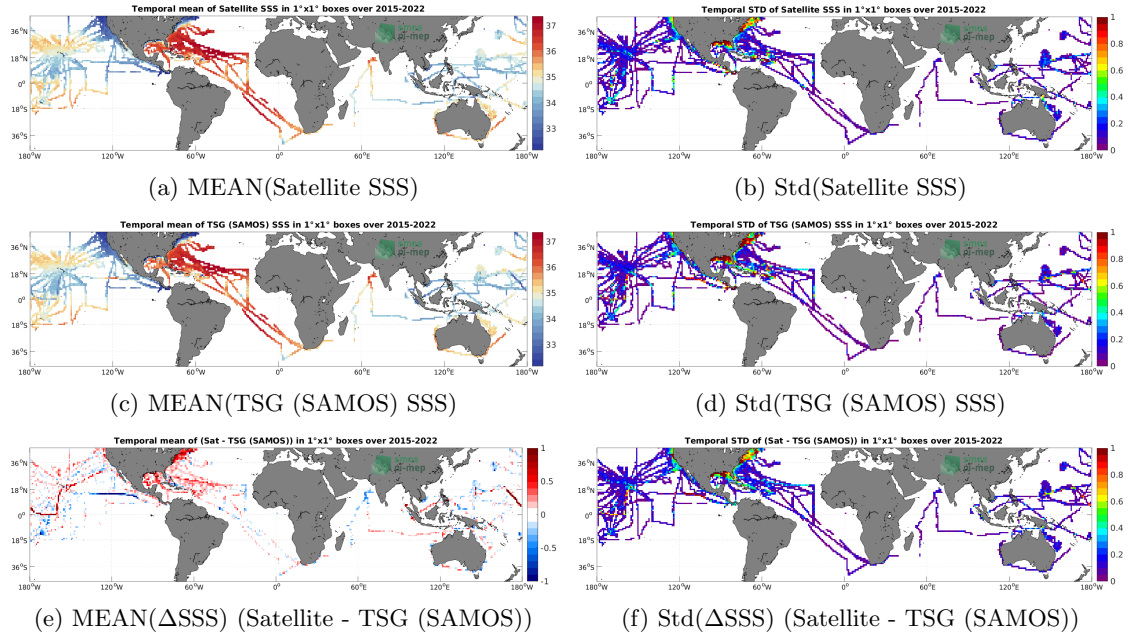
Figure 6: Temporal mean (left) and Std (right) of SSS from SMAP SSS L3 v5 - 8-Day running (RSS) (top), TSG (SAMOS) (middle), and of \Delta SSS (Satellite - TSG (SAMOS)). Only match-up pairs are used to generate these maps.
