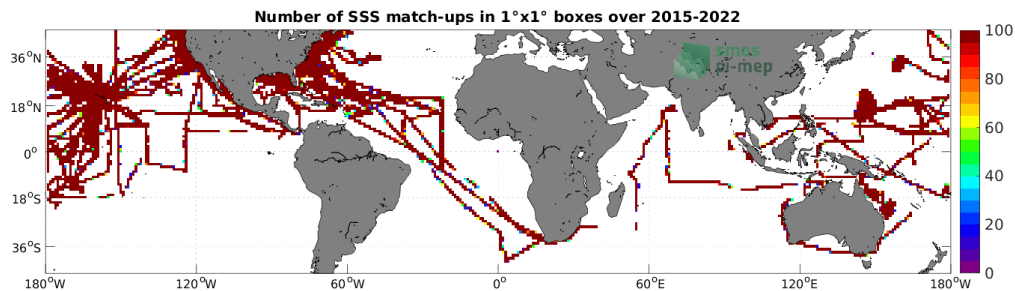
Figure 4: Number of SSS match-ups between TSG (SAMOS) SSS and the SMAP SSS L3 v5 - 8-Day running (RSS) SSS product for the Mid-Low Latitudes 45N-45S Pi-MEP region over 1^\circ \times 1^\circ boxes and for the full satellite product period.
