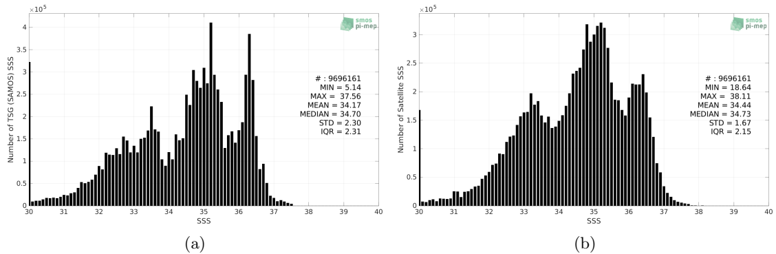
Figure 2: Histograms of SSS from TSG (SAMOS) (a) and SMAP SSS L3 v5 - 8-Day running (RSS) (b) considering all match-up pairs per bins of 0.1 over the Mid-Low Latitudes 45N-45S Pi-MEP region and for the full satellite product period.
