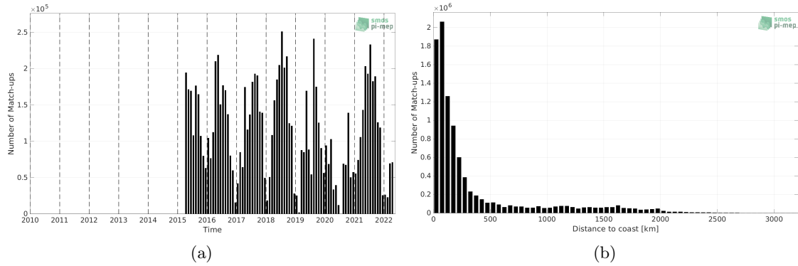
Figure 1: Number of match-ups between TSG (SAMOS) and SMAP SSS L3 v5 - 8-Day running (RSS) SSS as a function of time (a) and as function of the distance to coast (b) over the Mid-Low Latitudes 45N-45S Pi-MEP region and for the full satellite product period.
