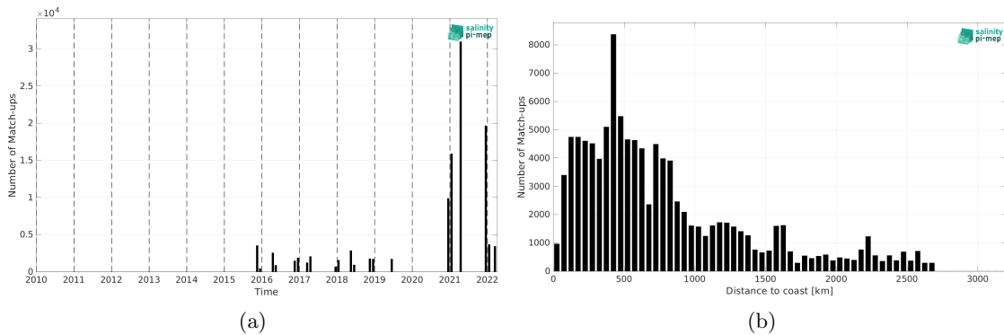
Figure 1: Number of match-ups between TSG (Polarstern) and SMAP SSS L3 v5 - 8-Day running (RSS) SSS as a function of time (a) and as function of the distance to coast (b) over the Mid-Low Latitudes 45N-45S Pi-MEP region and for the full satellite product period.
