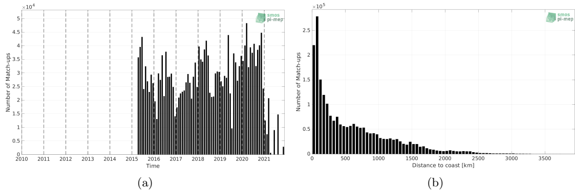
Figure 1: Number of match-ups between TSG (LEGOS-DM) and SMAP SSS L3 v5 - 8-Day running (RSS) SSS as a function of time (a) and as function of the distance to coast (b) over the Mid-Low Latitudes 45N-45S Pi-MEP region and for the full satellite product period.
