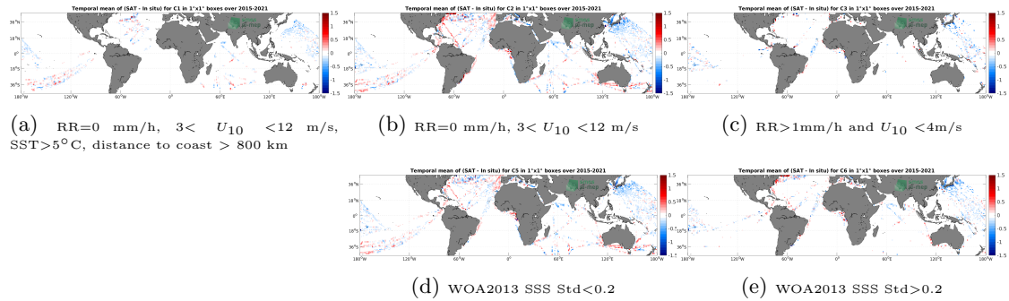
Figure 12: Temporal mean gridded over spatial boxes of size 1^\circ \times 1^\circ of \Delta SSS (SMAP SSS L3 v5 - 8-Day running (RSS) - TSG (LEGOS-DM)) for 5 different subdatasets corresponding to: RR=0 mm/h, 3 < U_{10} < 12 m/s, SST > 5^\circ\text{C} , distance to coast > 800 km (a), RR=0 mm/h, 3 < U_{10} < 12 m/s (b), RR > 1\text{mm/h} and U_{10} < 4\text{m/s} (c), WOA2013 SSS Std < 0.2 (d), WOA2013 SSS Std > 0.2 (e).
