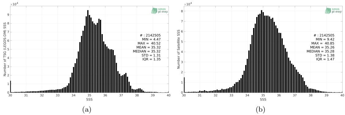
Figure 2: Histograms of SSS from TSG (LEGOS-DM) (a) and SMAP SSS L3 v5 - 8-Day running (RSS) (b) considering all match-up pairs per bins of 0.1 over the Mid-Low Latitudes 45N-45S Pi-MEP region and for the full satellite product period.
