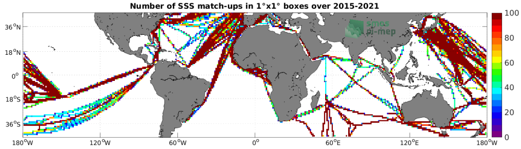
Figure 4: Number of SSS match-ups between TSG (LEGOS-DM) SSS and the SMAP SSS L3 v5 - 8-Day running (RSS) SSS product for the Mid-Low Latitudes 45N-45S Pi-MEP region over 1^\circ \times 1^\circ boxes and for the full satellite product period.
