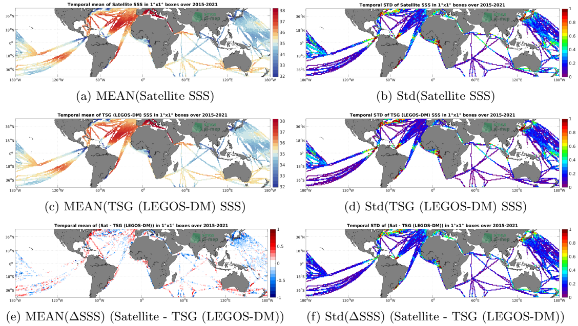
Figure 6: Temporal mean (left) and Std (right) of SSS from SMAP SSS L3 v5 - 8-Day running (RSS) (top), TSG (LEGOS-DM) (middle), and of \Delta SSS (Satellite - TSG (LEGOS-DM)). Only match-up pairs are used to generate these maps.
