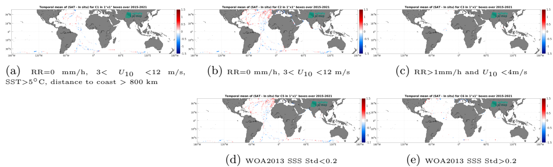
Figure 12: Temporal mean gridded over spatial boxes of size 1^\circ \times 1^\circ of \Delta\text{SSS} (SMAP SSS L3 v5 - 8-Day running (RSS) - TSG (GOSUD-Sailing-ship)) for 5 different subdatasets corresponding to: RR=0 mm/h, 3 < U_{10} < 12 m/s, SST > 5°C, distance to coast > 800 km (a), RR=0 mm/h, 3 < U_{10} < 12 m/s (b), RR > 1mm/h and U_{10} < 4 m/s (c), WOA2013 SSS Std < 0.2 (d), WOA2013 SSS Std > 0.2 (e).
